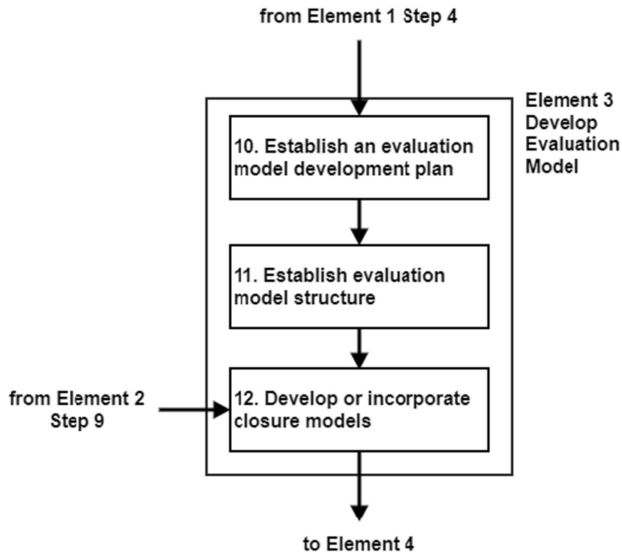
Figure 5-15 Steps in EMDAP Element 3 [1]
