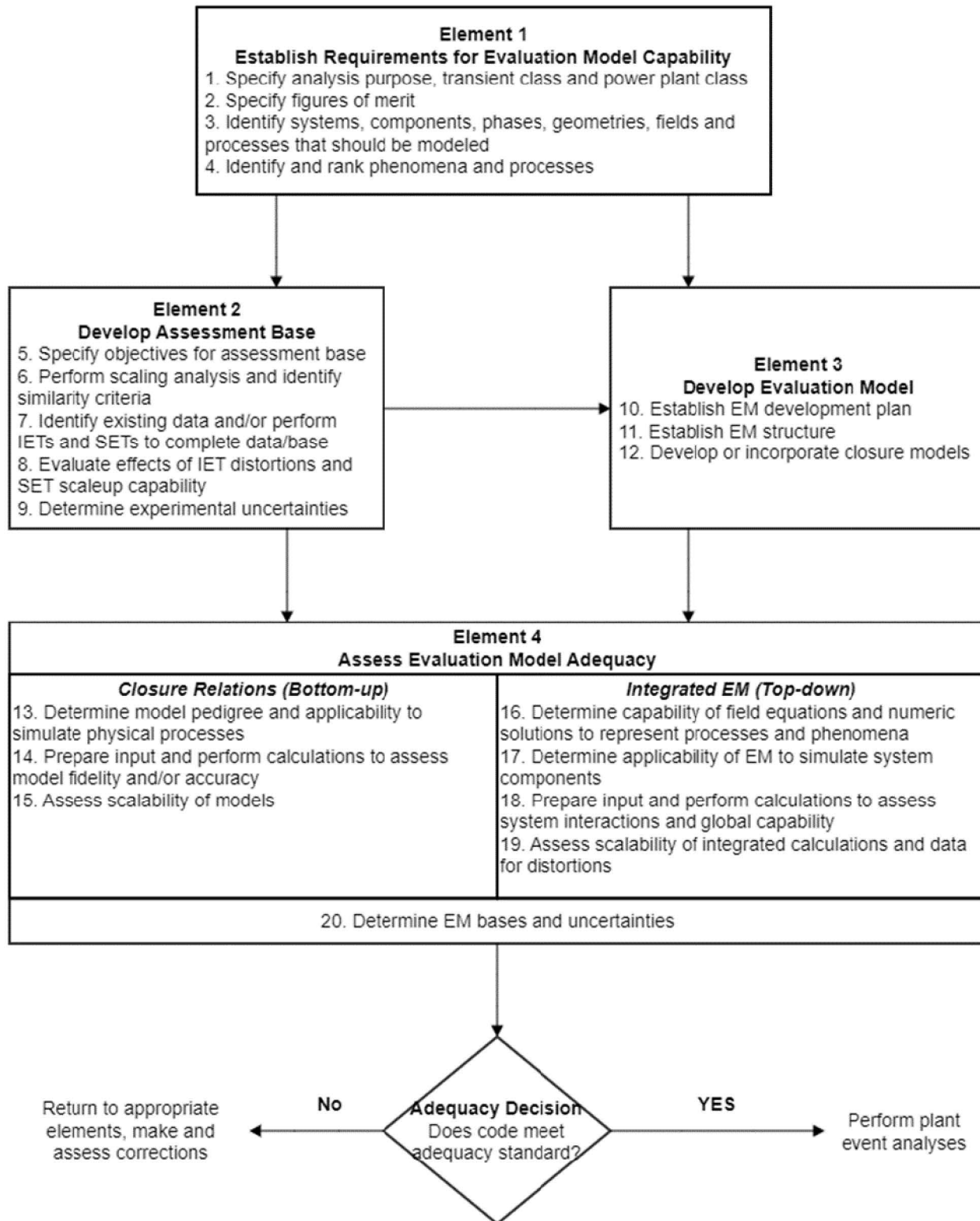
Figure 5-1 Overall Diagram of EMDAP and Relationships among Elements [1]
