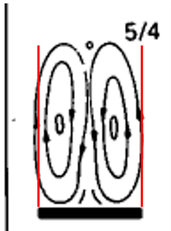
Figure 5-13: Streamlines from 169 Pin SNR Bundle [11] with Red Lines added to Represent Gap Faces
