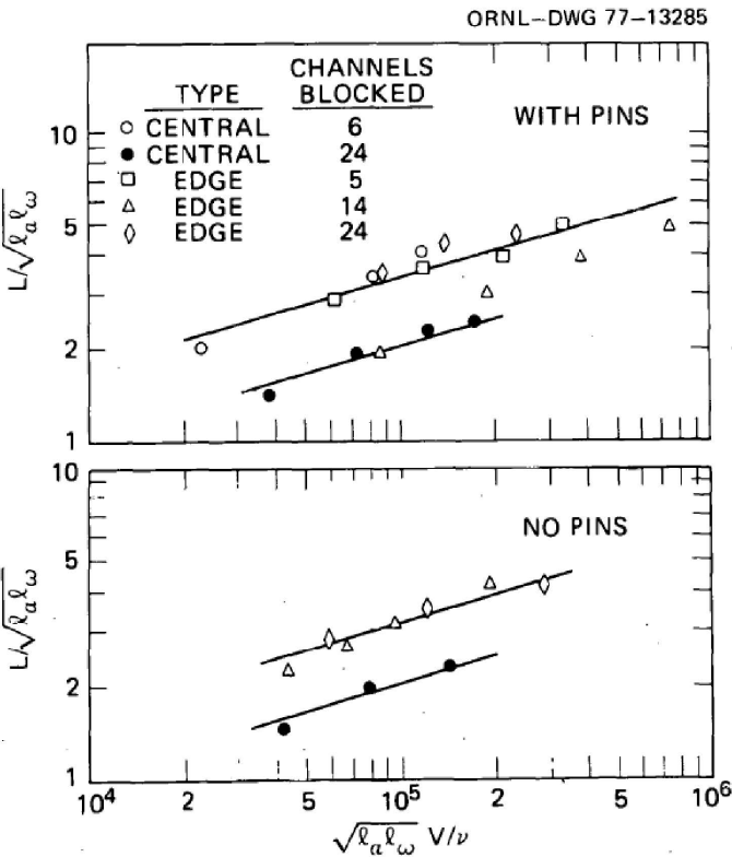
Figure 5-17 Wake Length to Blockage Diameter Ratio versus Blockage Reynolds Number from ORNL (Reference [11], Page 71)
