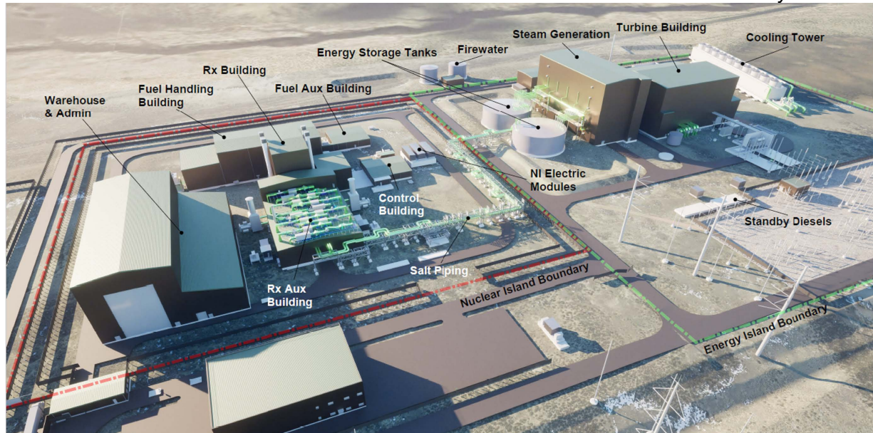
Figure 5-4 Natrium Plant Layout
