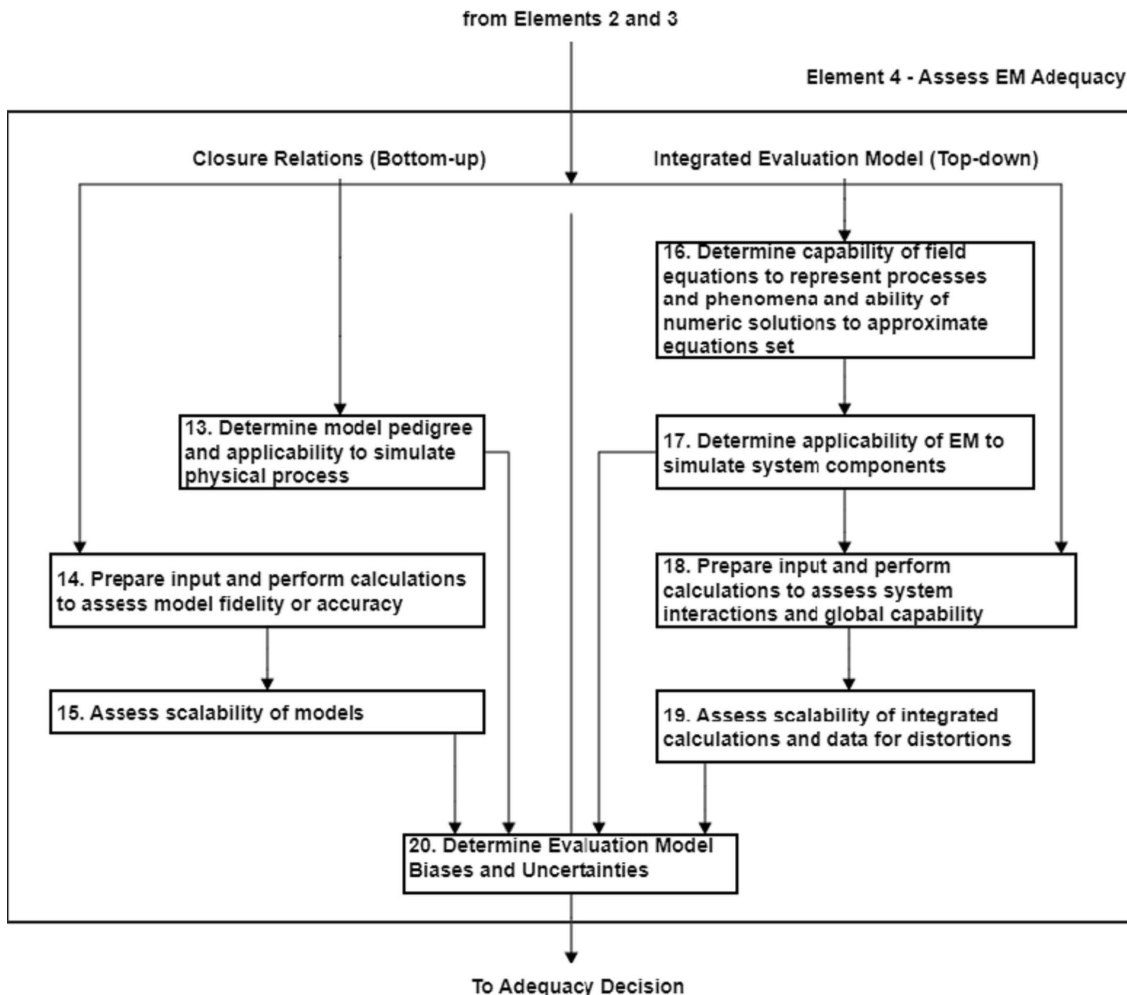
Figure 5-31 Steps in EMDAP Element 4 [1]
