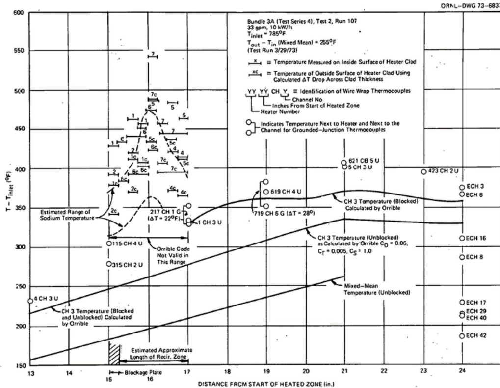
Figure 5-21 Measured Cladding and Coolant Temperature from ORNL 3A Experiments (References [14], [11], and [32]) with 32.8 kW/m and 33 gpm
