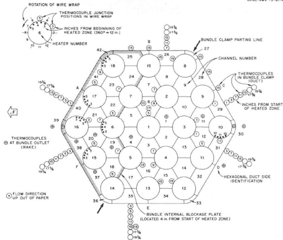
Figure 5-26 Schematic of ORNL THORS 5B 14-Subchannel Edge Blockage [33]
