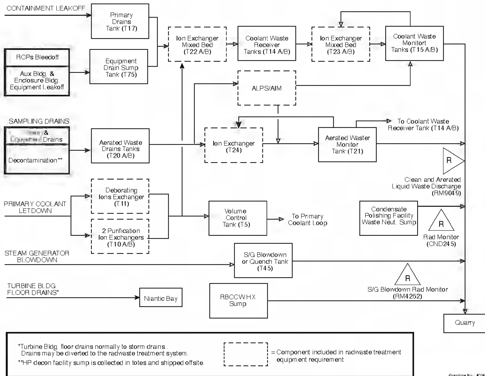
Figure I.C.-2, "Simplified Liquid Effluent Flow Diagram Millstone Unit 2"
