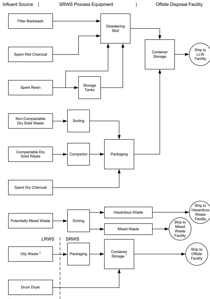
Figure 11.4-1: Block Diagram of the Solid Radioactive Waste System
