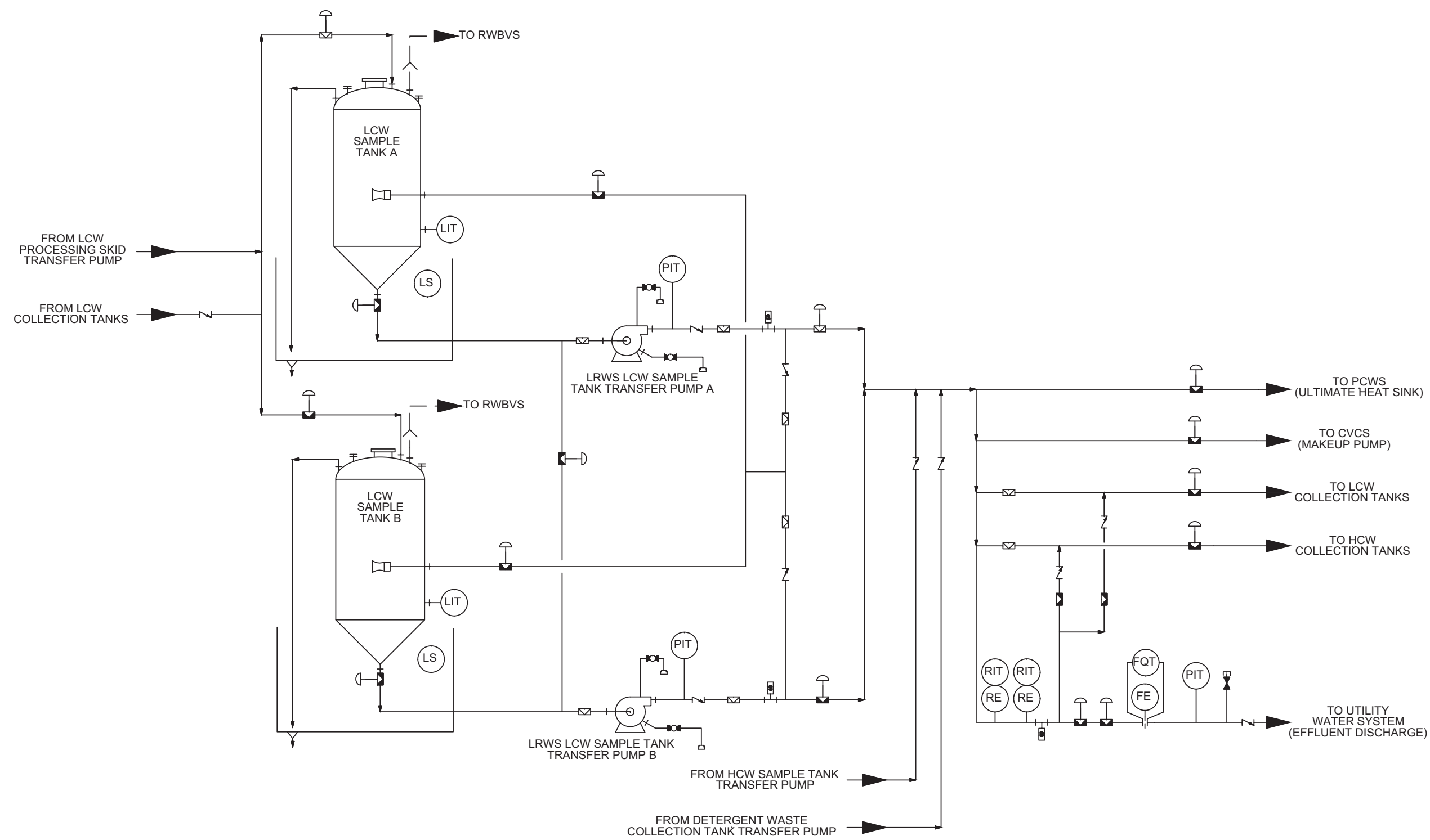
Figure 11.2-1g: Liquid Radioactive Waste System Diagram
