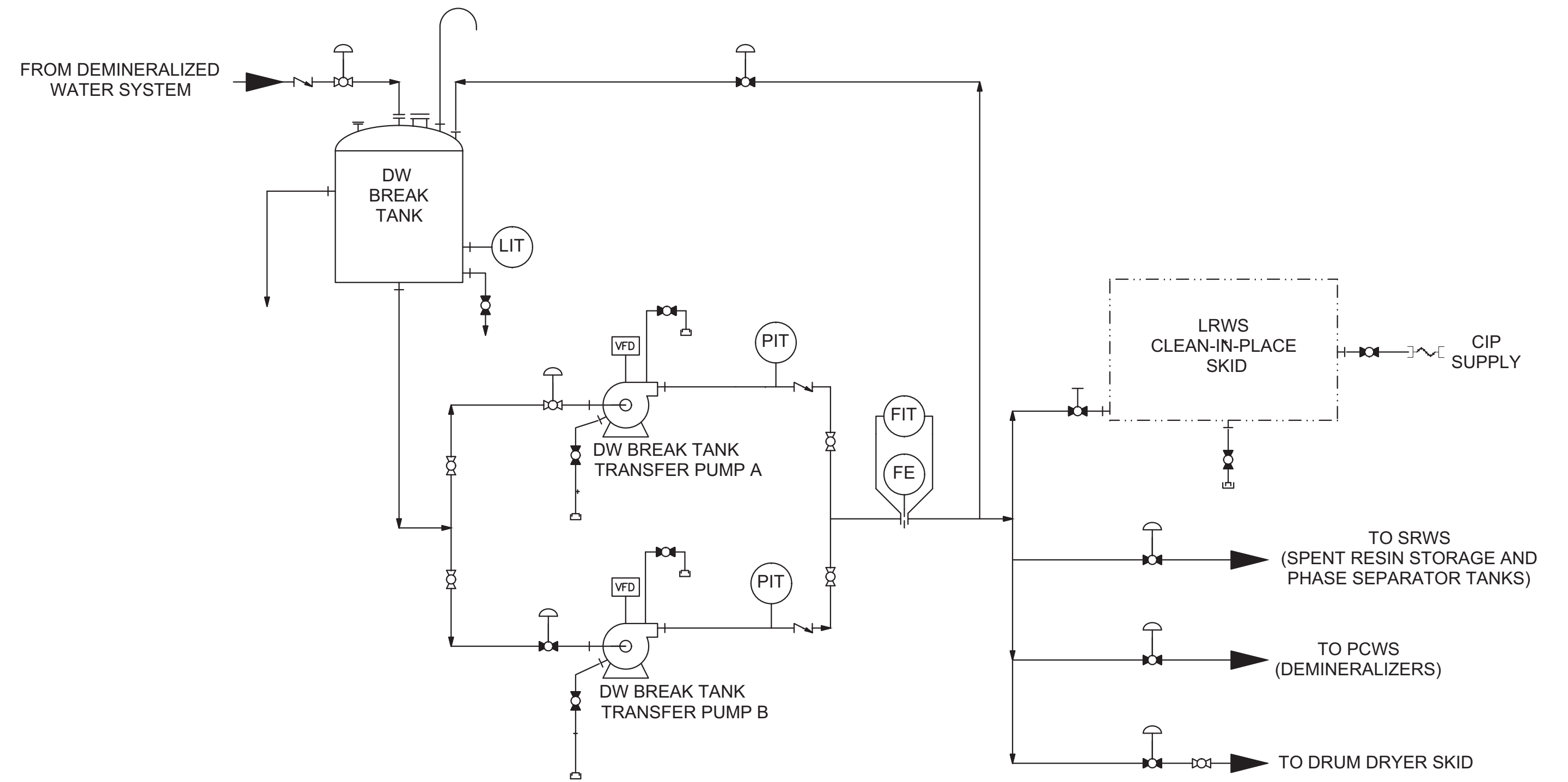
Figure 11.2-1d: Liquid Radioactive Waste System Diagram
