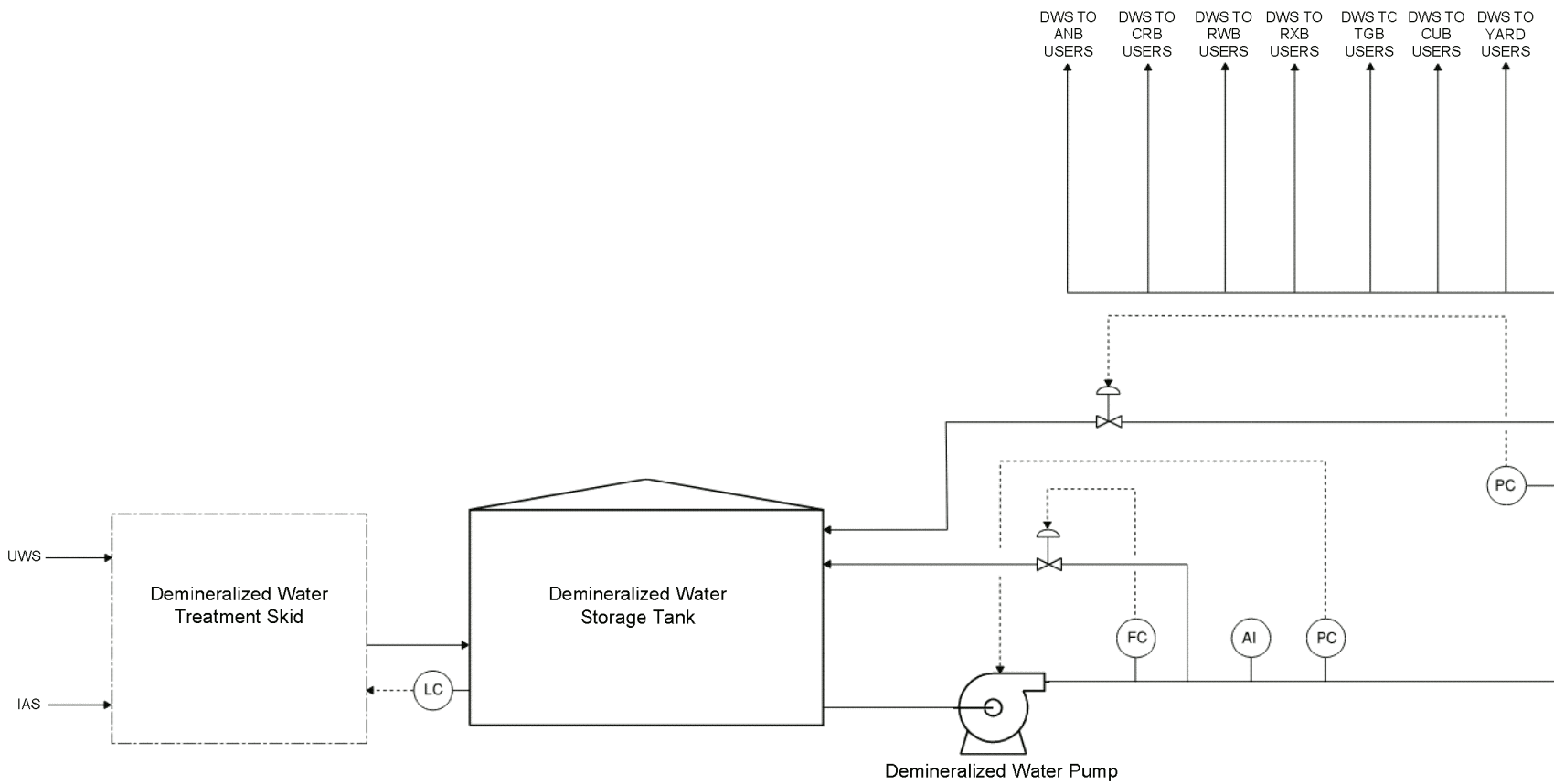
Figure 9.2.3-1: Demineralized Water System Simplified Diagram
