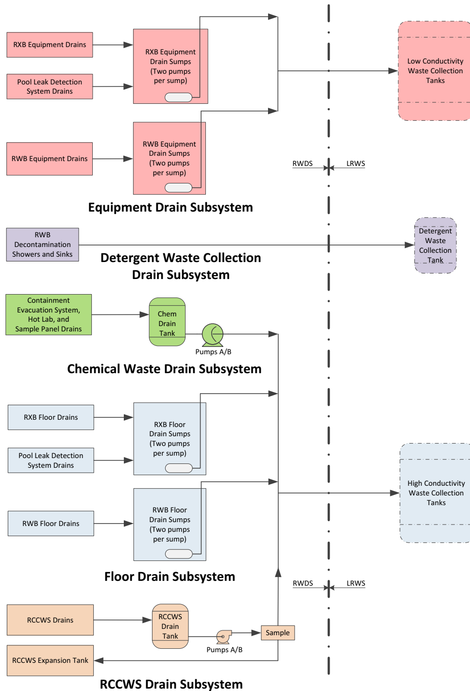
Figure 9.3.3-1: Radioactive Waste Drain System Diagram
