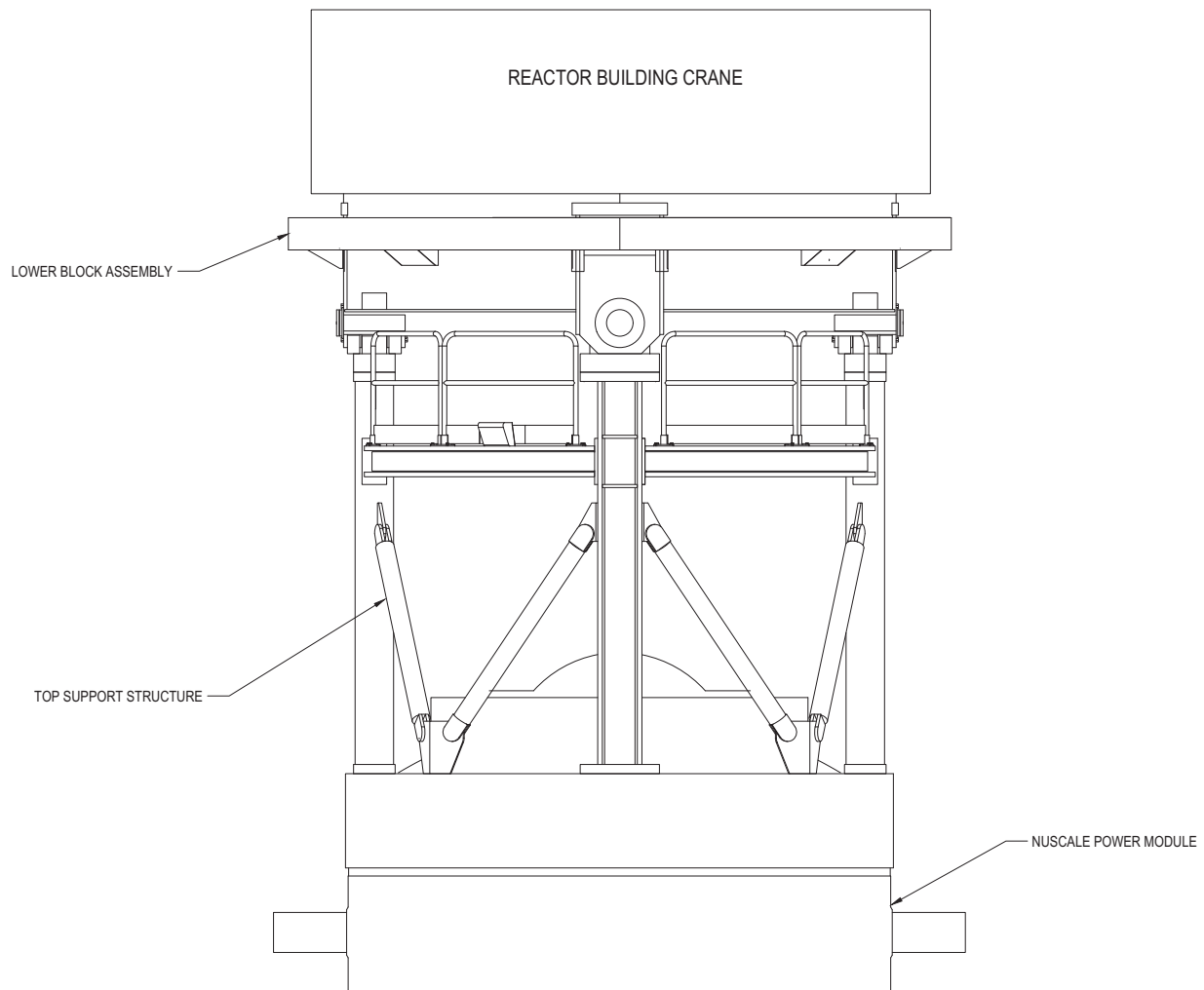
Figure 9.1.5-3: Reactor Building Crane Lower Block Assembly Connection to the Top Support Structure
