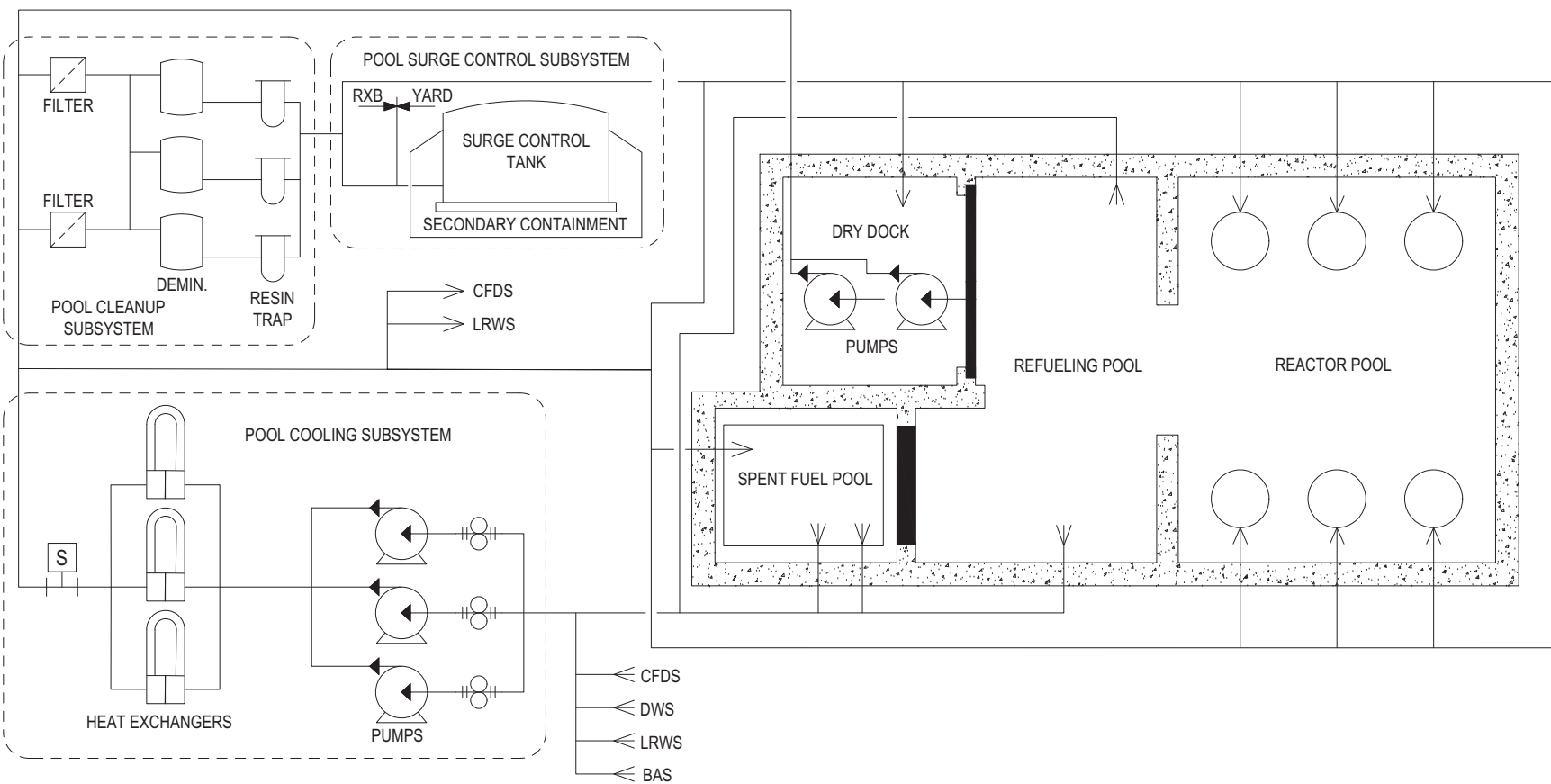
Figure 9.1.3-1: Pool Cooling and Cleanup System Diagram
