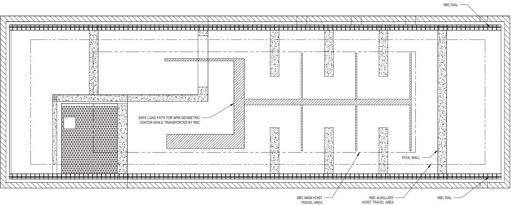
Figure 9.1.5-1: NuScale Power Module Safe Load Path
