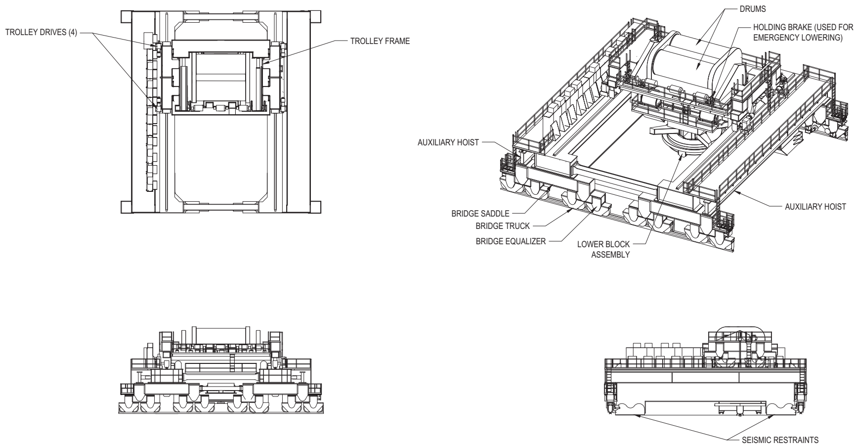
Figure 9.1.5-2: Reactor Building Crane
