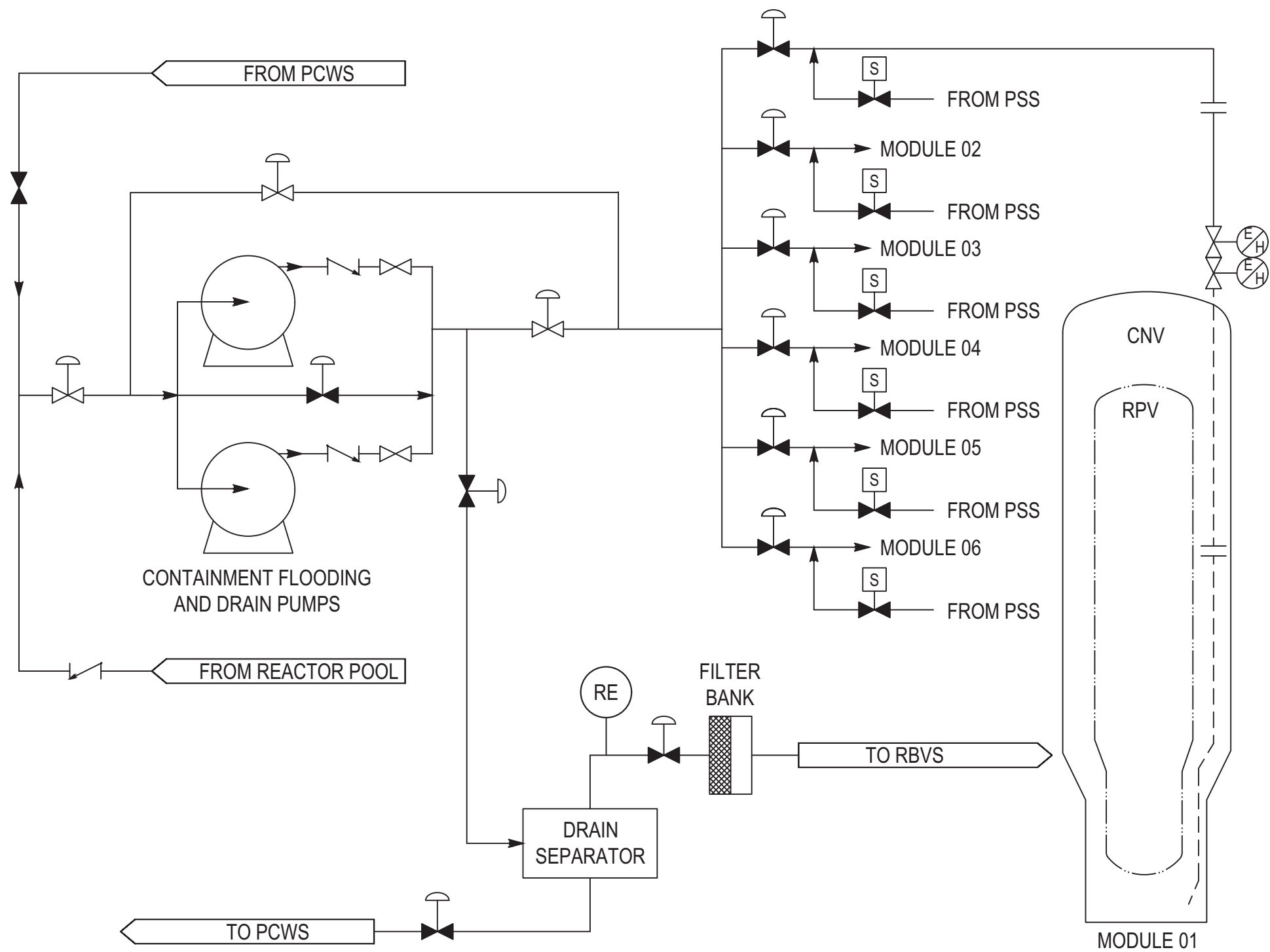
Figure 9.3.7-1: Containment Flooding and Drain System Diagram
