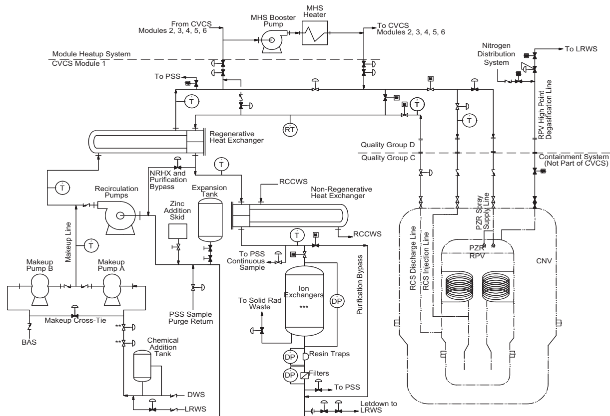
Figure 9.3.4-1: Chemical and Volume Control System Diagram (Chemical and Volume Control System Module 1 with Module Heatup System Shown)
