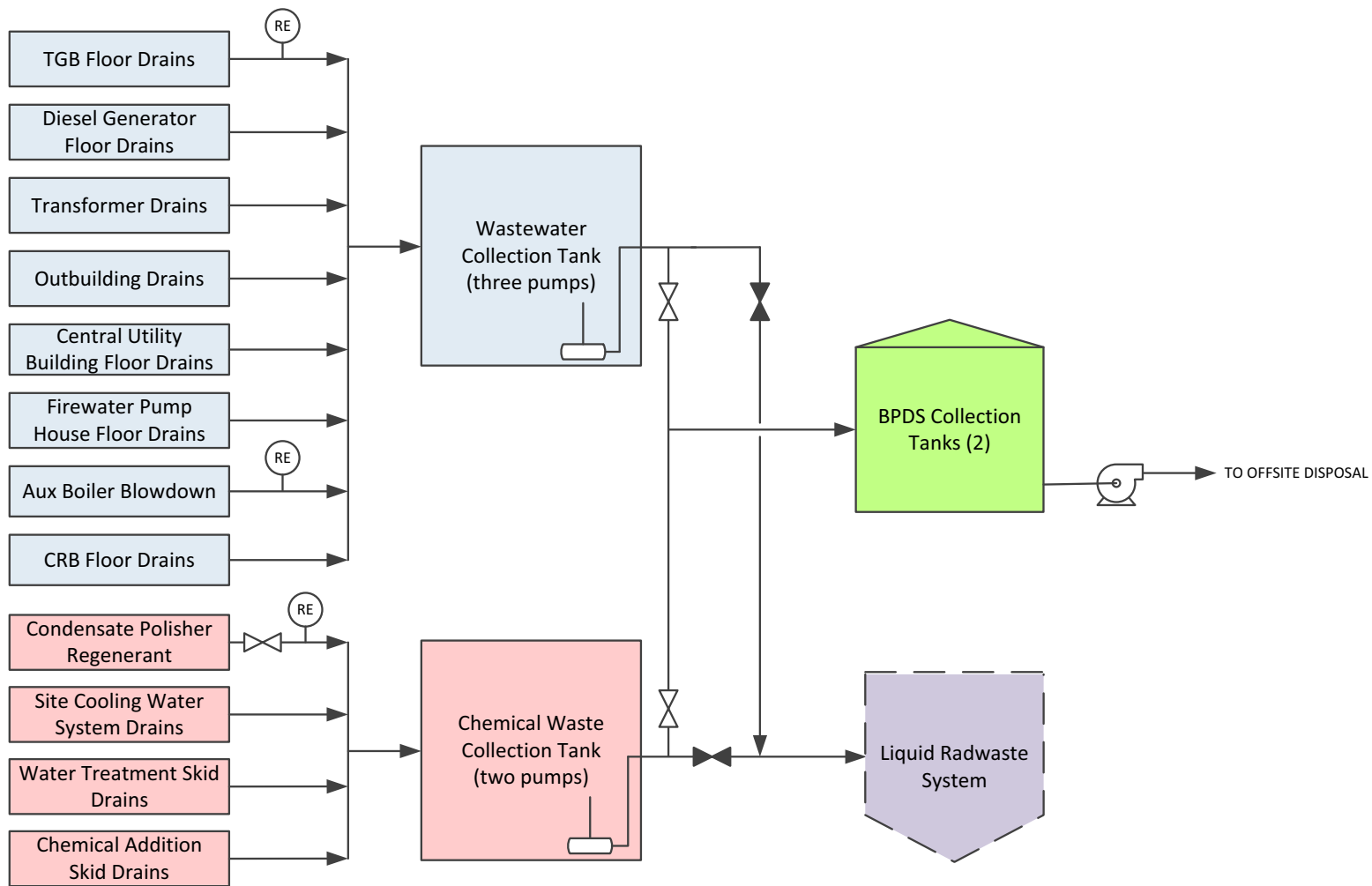
Figure 9.3.3-2: Balance-of-Plant Drain System Diagram
