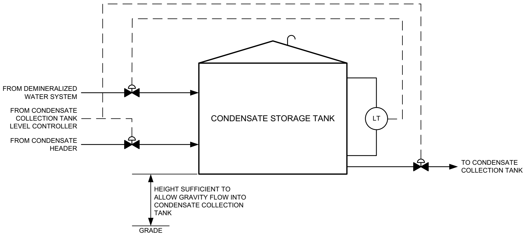
Figure 9.2.6-1: Condensate Storage Facility
