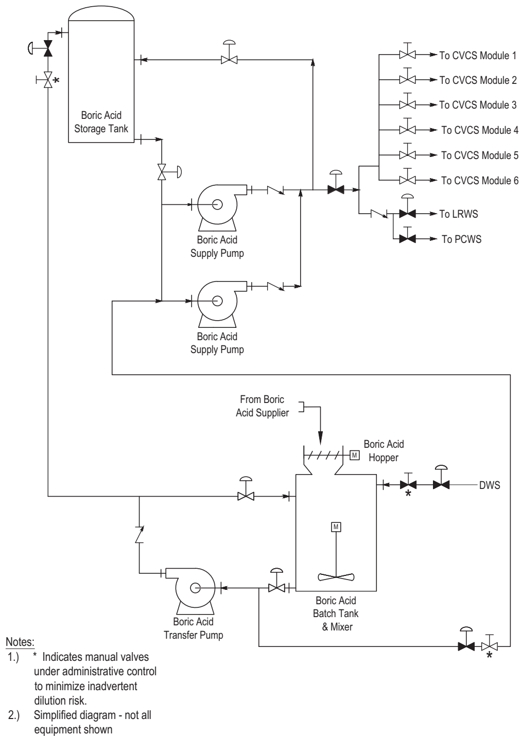
Figure 9.3.4-2: Boron Addition System Diagram
