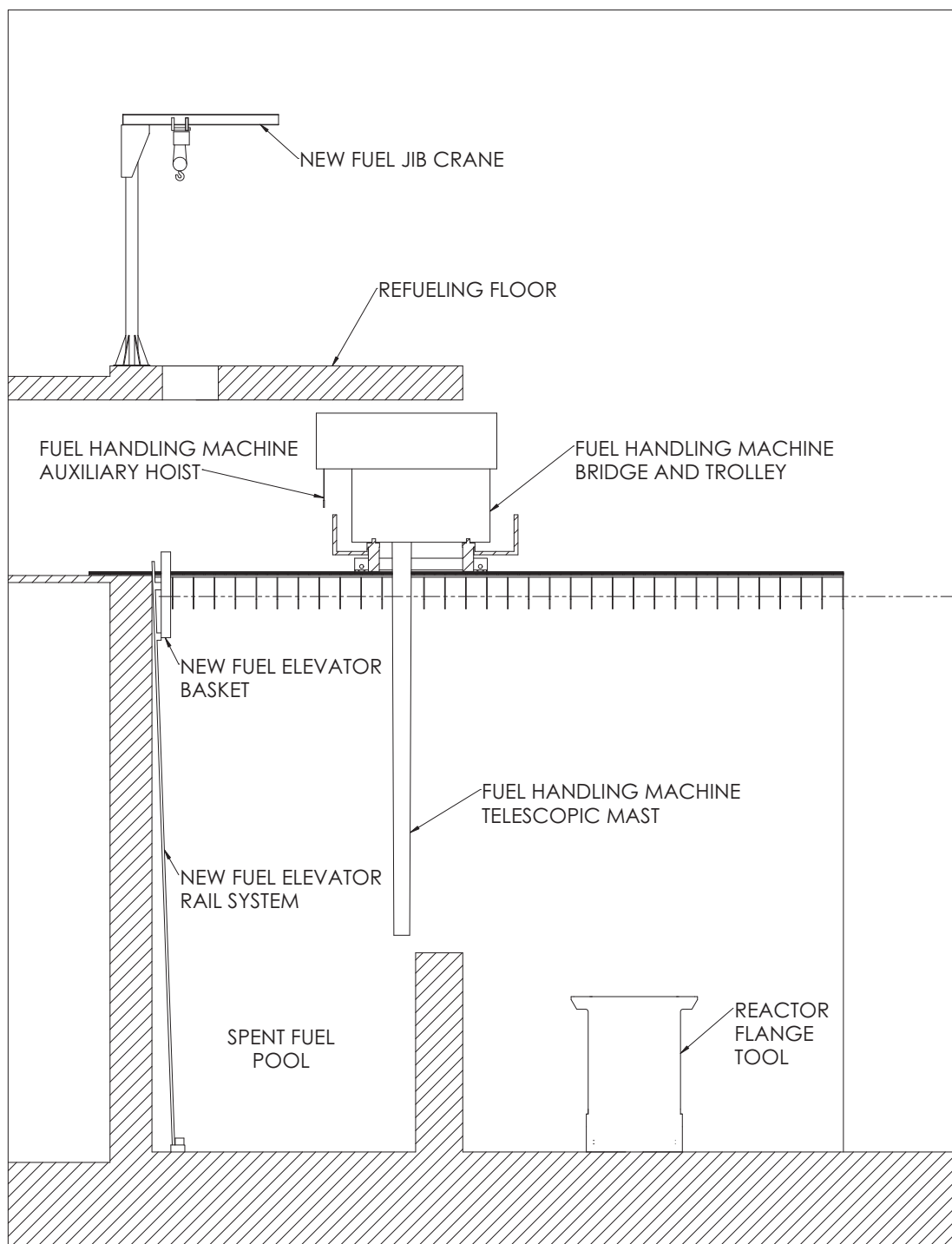
Figure 9.1.4-1: Refueling Floor Layout
