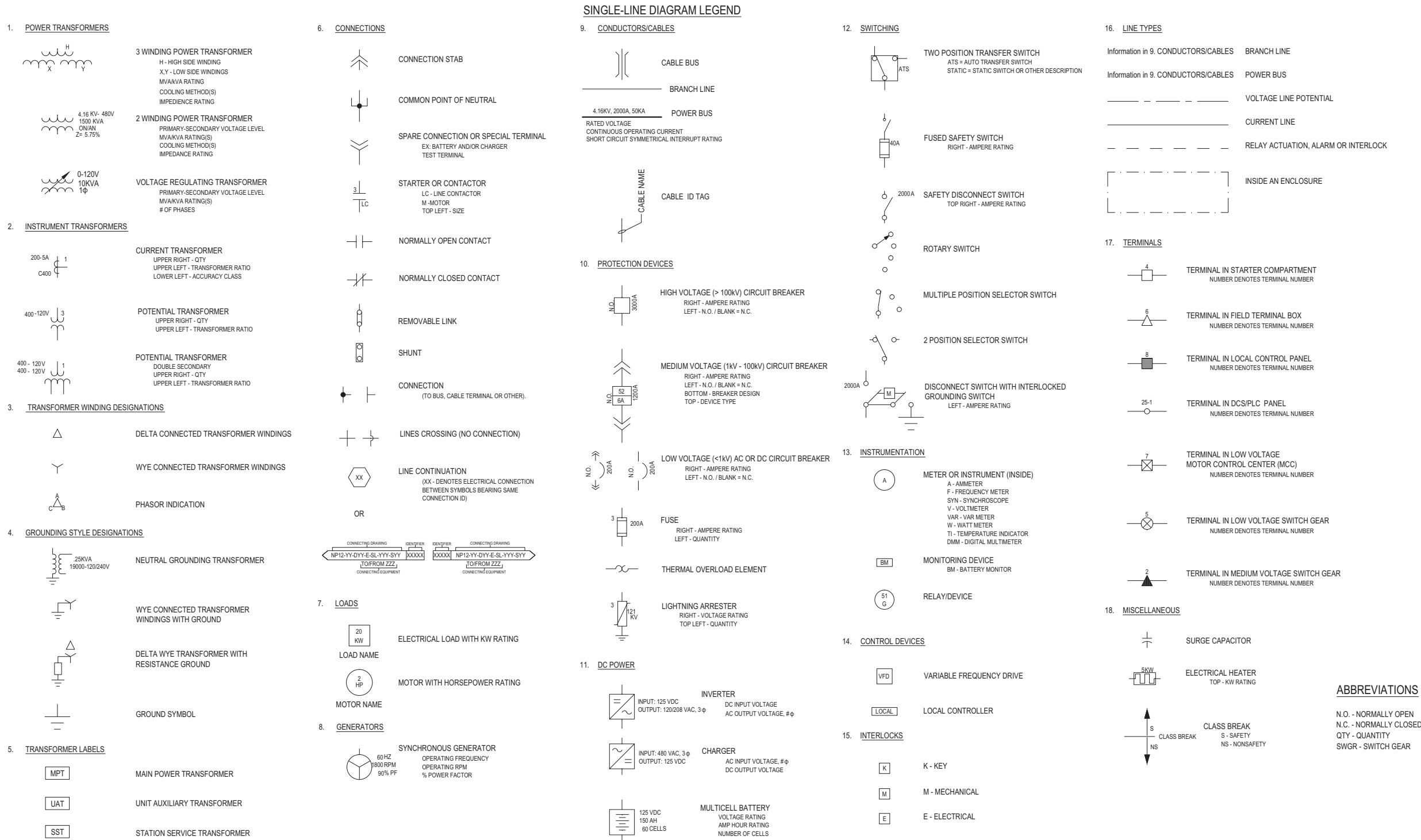
Figure 1.7-1a: Electrical Symbols
