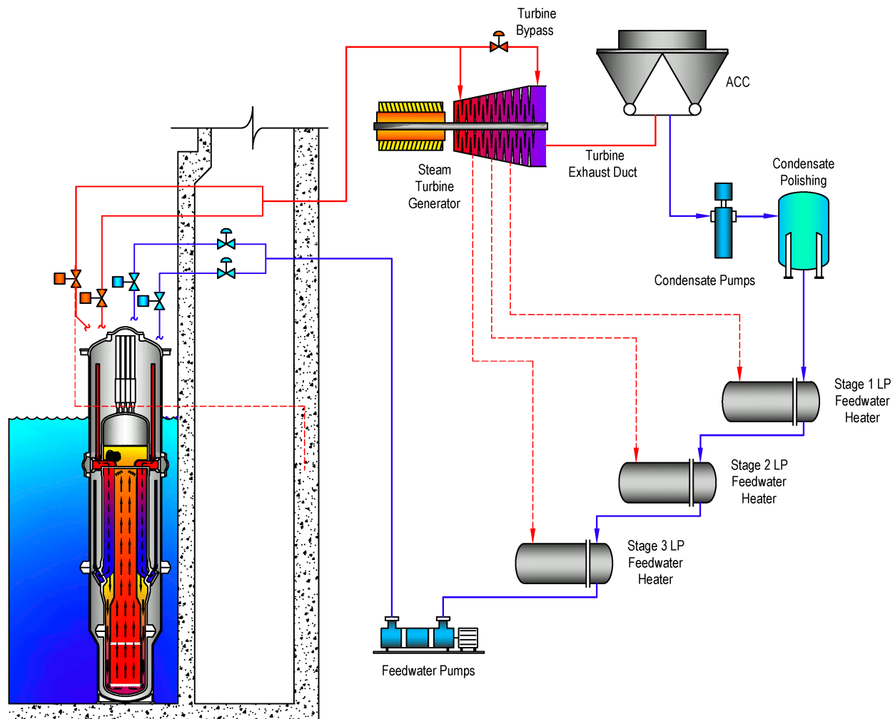
Figure 1.2-2: Schematic of a Single NuScale Power Module and Associated Secondary Equipment
