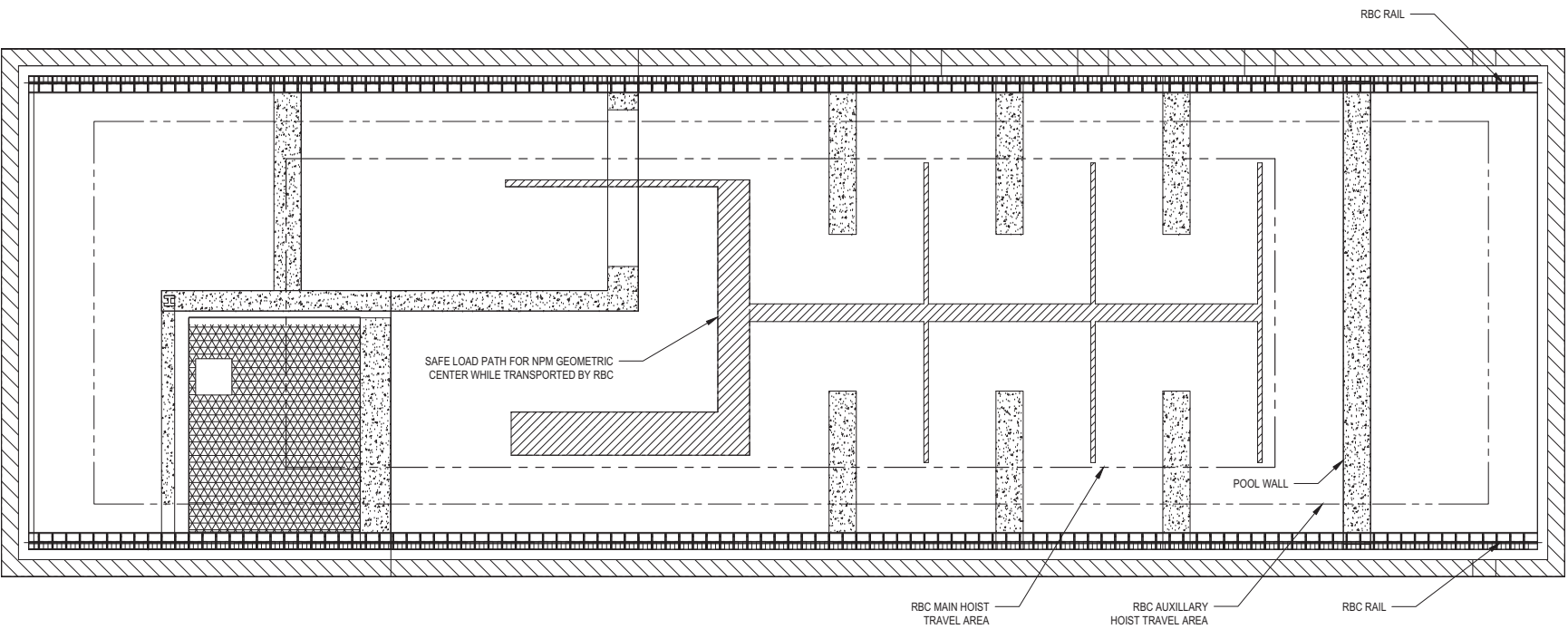
Figure 9.1.5-1: Reactor Building Crane Safe Load Path
