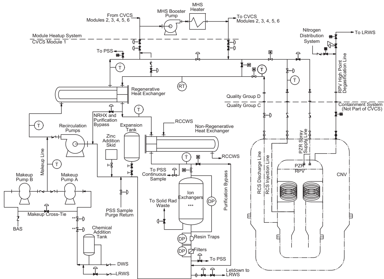
Figure 9.3.4-1: Chemical and Volume Control System Diagram (Chemical and Volume Control System Module 1 with Module Heatup System Shown)
