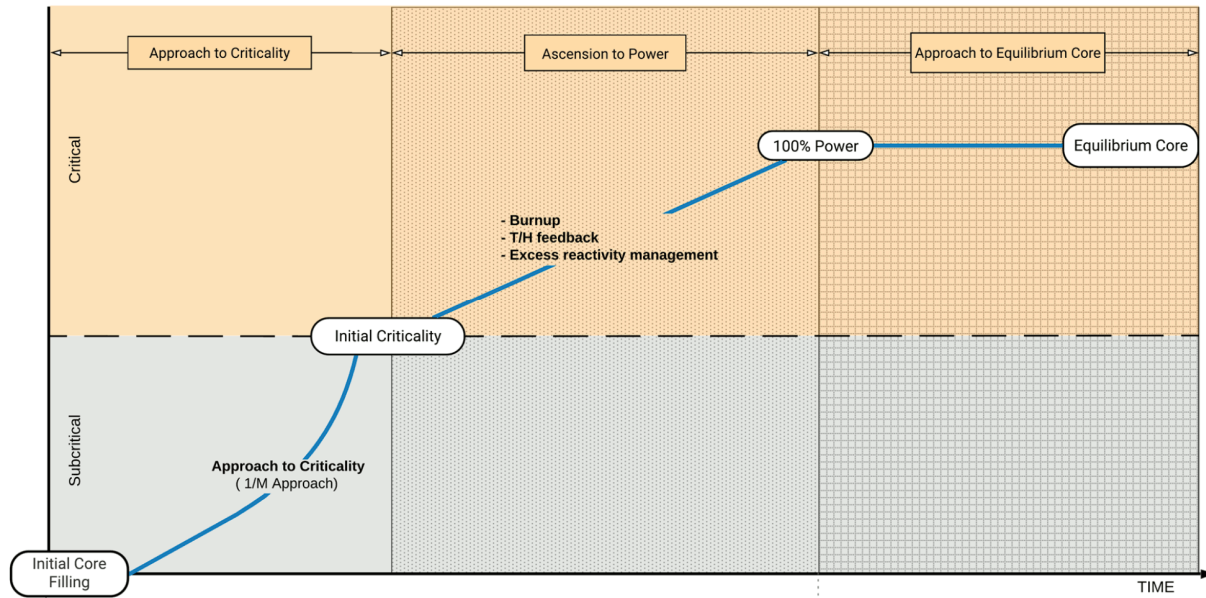
Figure 2-4. Reactor Core Operational Regimes of the KP-FHR
