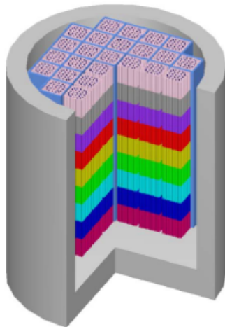
53 Figure 4.3 Cutaway view of the GBC-32 cask showing the cask bottom half with a quarter of the model removed.
