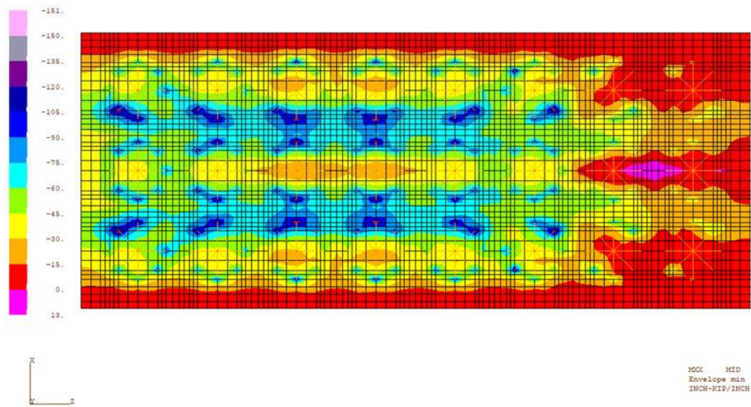
Figure 7-23 Enveloping Negative Moment Resultants (kip-in/in) About Global Z-Axis (local M_{xx} ) - Configuration 4
