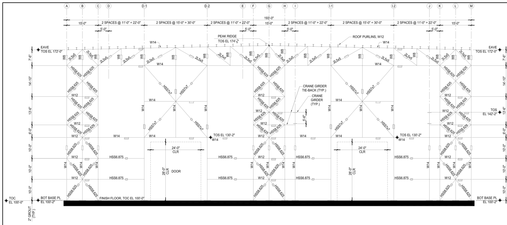
Figure 7-57 Cask Handling Building Structural Steel Framing Arrangement, Section at North Exterior Frame (Looking North)
