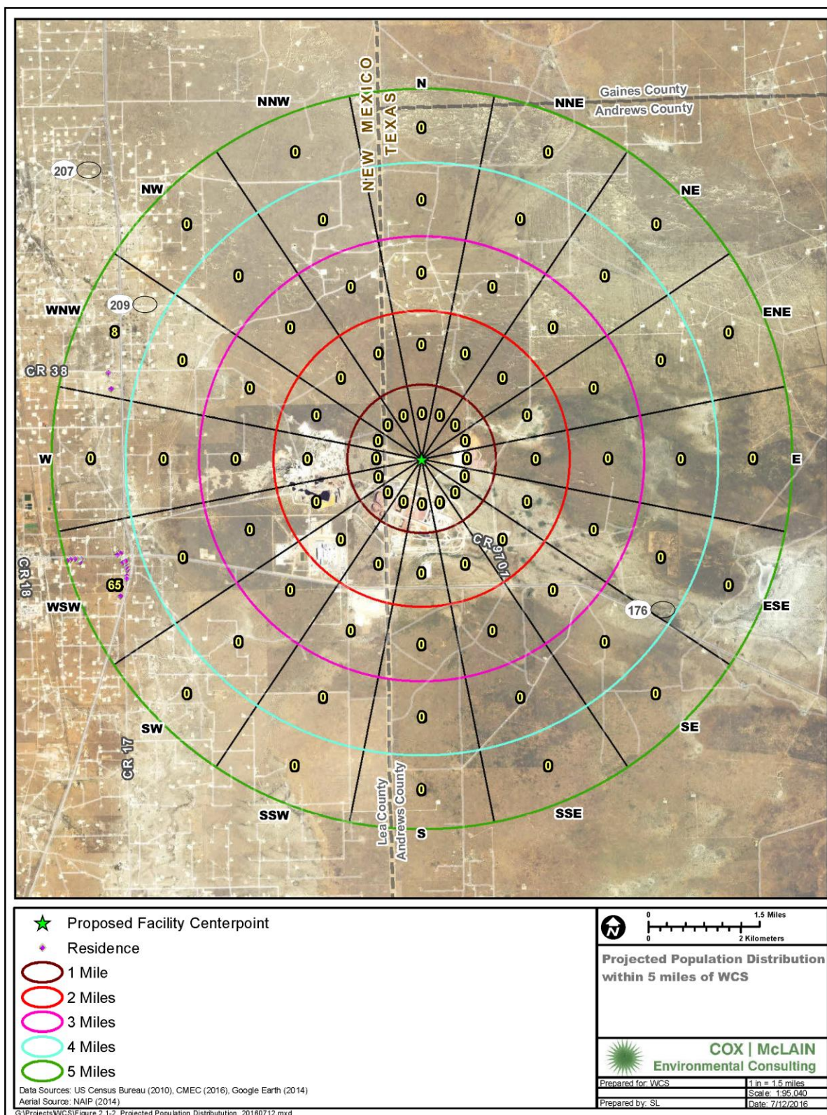
Figure 2-20 Projected Population Distribution within 5 Miles of the WCS CISF
