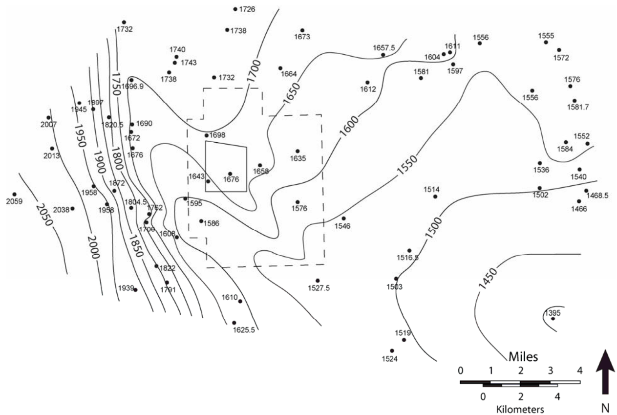
Figure 15 – Elevation (ft amsl) of the top of the Salado Formation.
