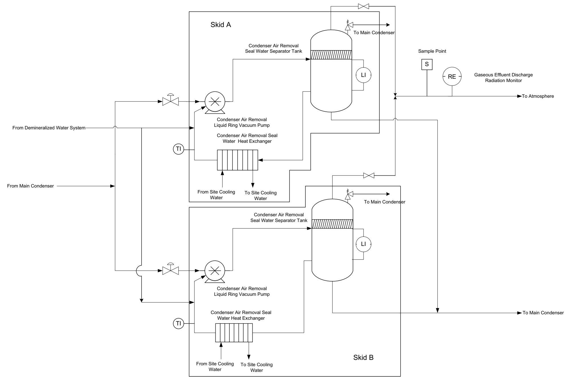
Figure 10.4-2: Condenser Air Removal System Piping and Instrumentation Diagram
