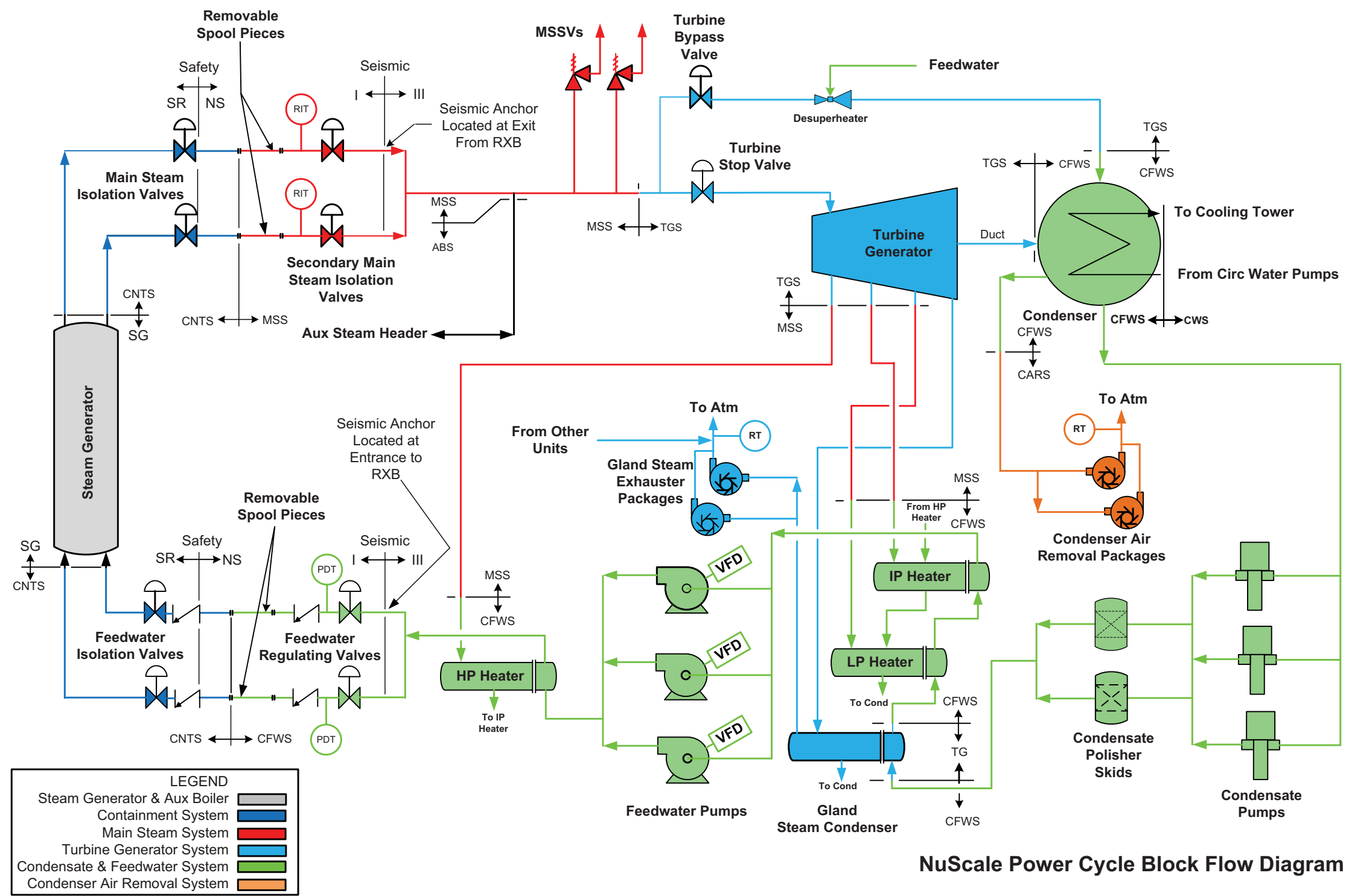
Figure 10.1-1: Power Conversion System Block Flow Diagram
