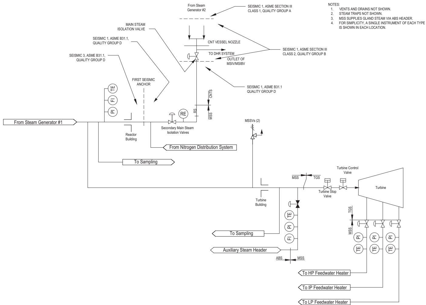
Figure 10.3-1: Main Steam System Piping and Instrumentation Diagram
