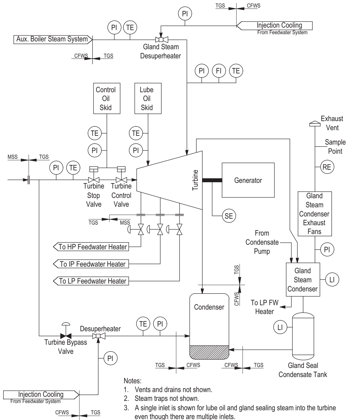
Figure 10.2-1: Turbine Generator System Piping and Instrumentation Diagram
