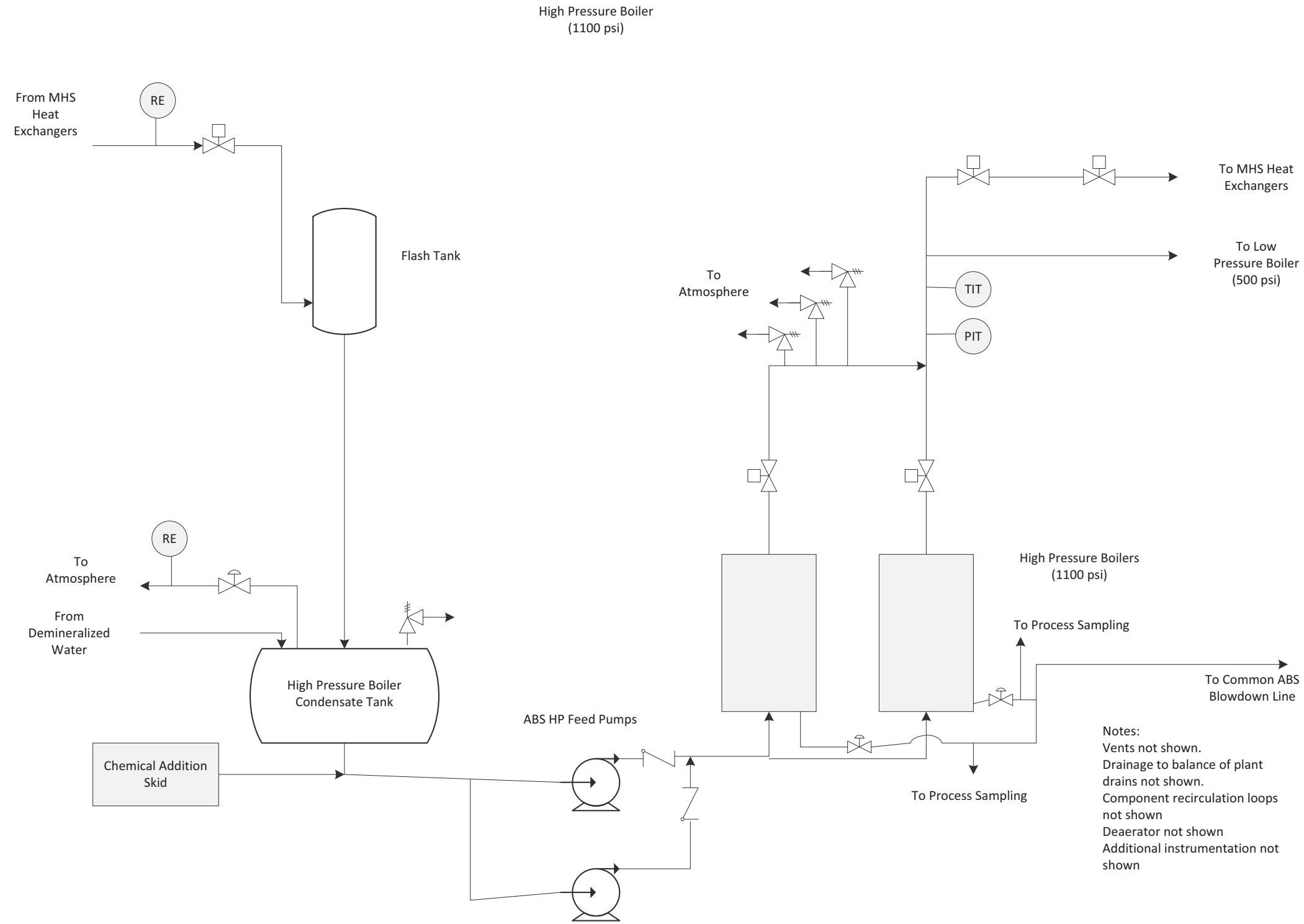
Figure 10.4-4a: Auxiliary Boiler System Piping and Instrumentation Diagram
