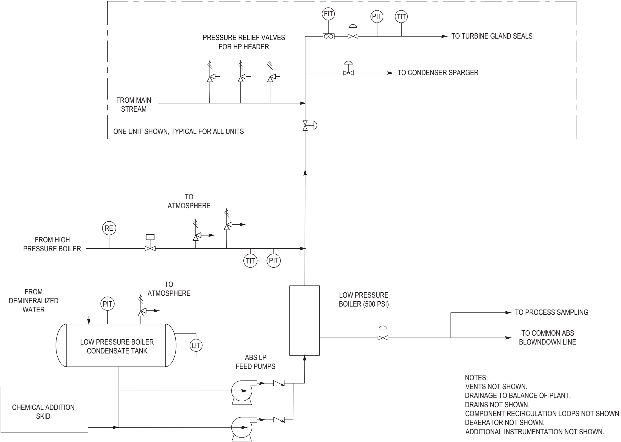
Figure 10.4-4b: Auxiliary Boiler System Piping and Instrumentation Diagram
