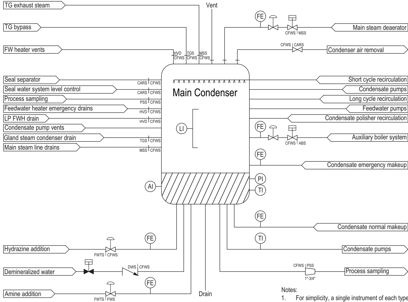
Figure 10.4-1: Main Condenser Piping and Instrumentation Diagram
