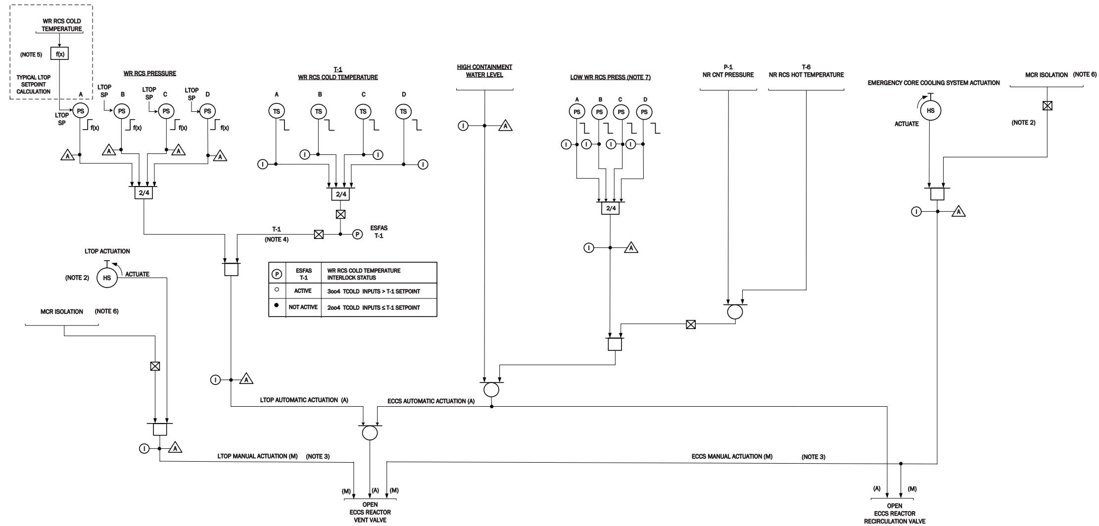
Figure 7.1-1n: ESFAS Emergency Core Cooling System Actuation, Low Temperature Overpressure Protection Actuation
