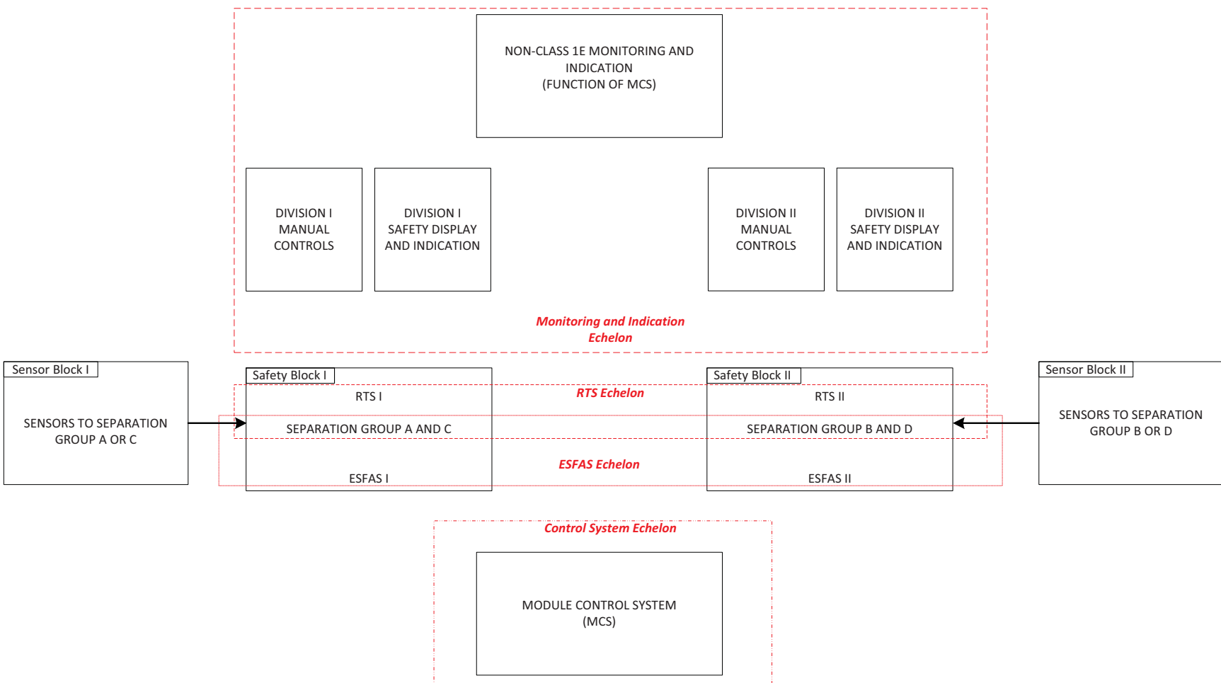
Figure 7.1-6: Four Echelons of Defense within Chosen Blocks
