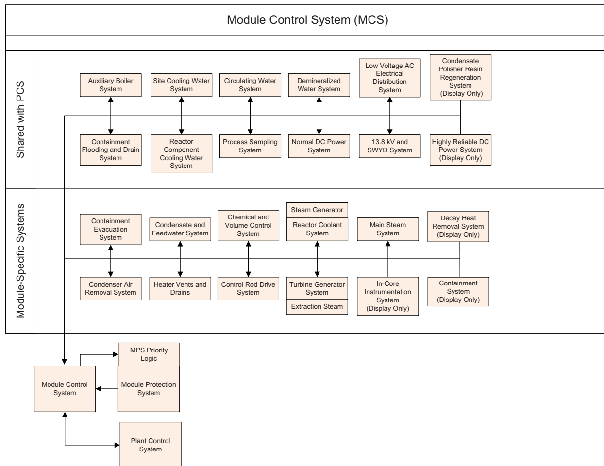
Figure 7.0-17: Module Control System Internal Functions and External Interfaces
