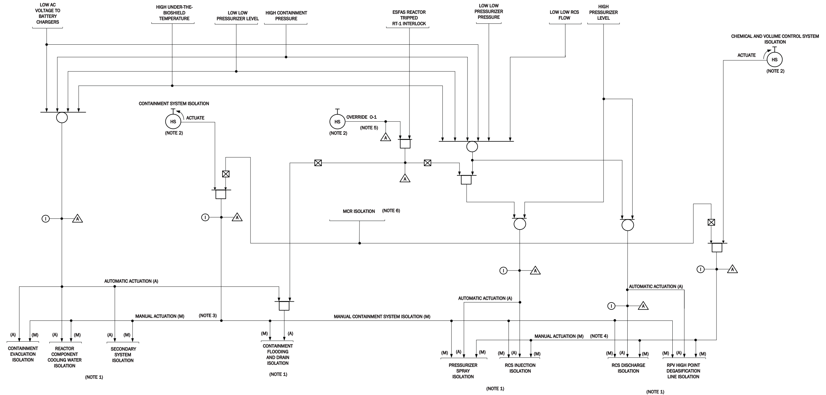
Figure 7.1-1k: ESFAS - Containment System Isolation and Chemical and Volume Control System Isolation Interlocks
