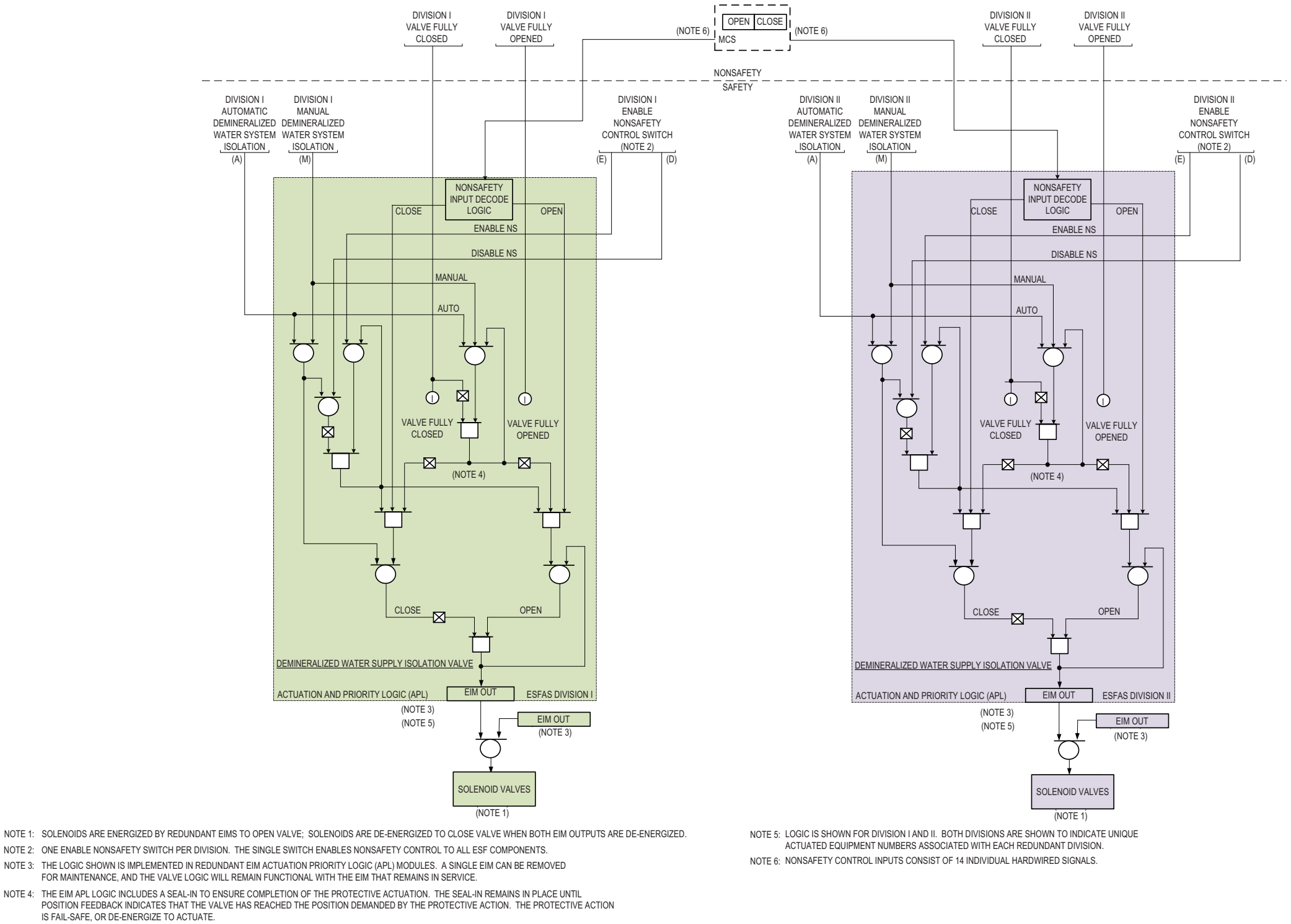
Figure 7.1-1z: Demineralized Water Supply Valve Actuation
