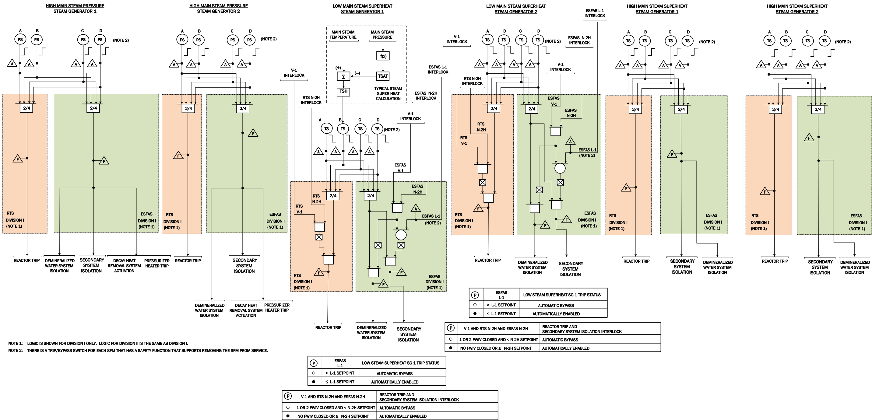
Figure 7.1-1i: High Main Steam Pressure and Steam Generator Low and High Steam Superheat Trips
