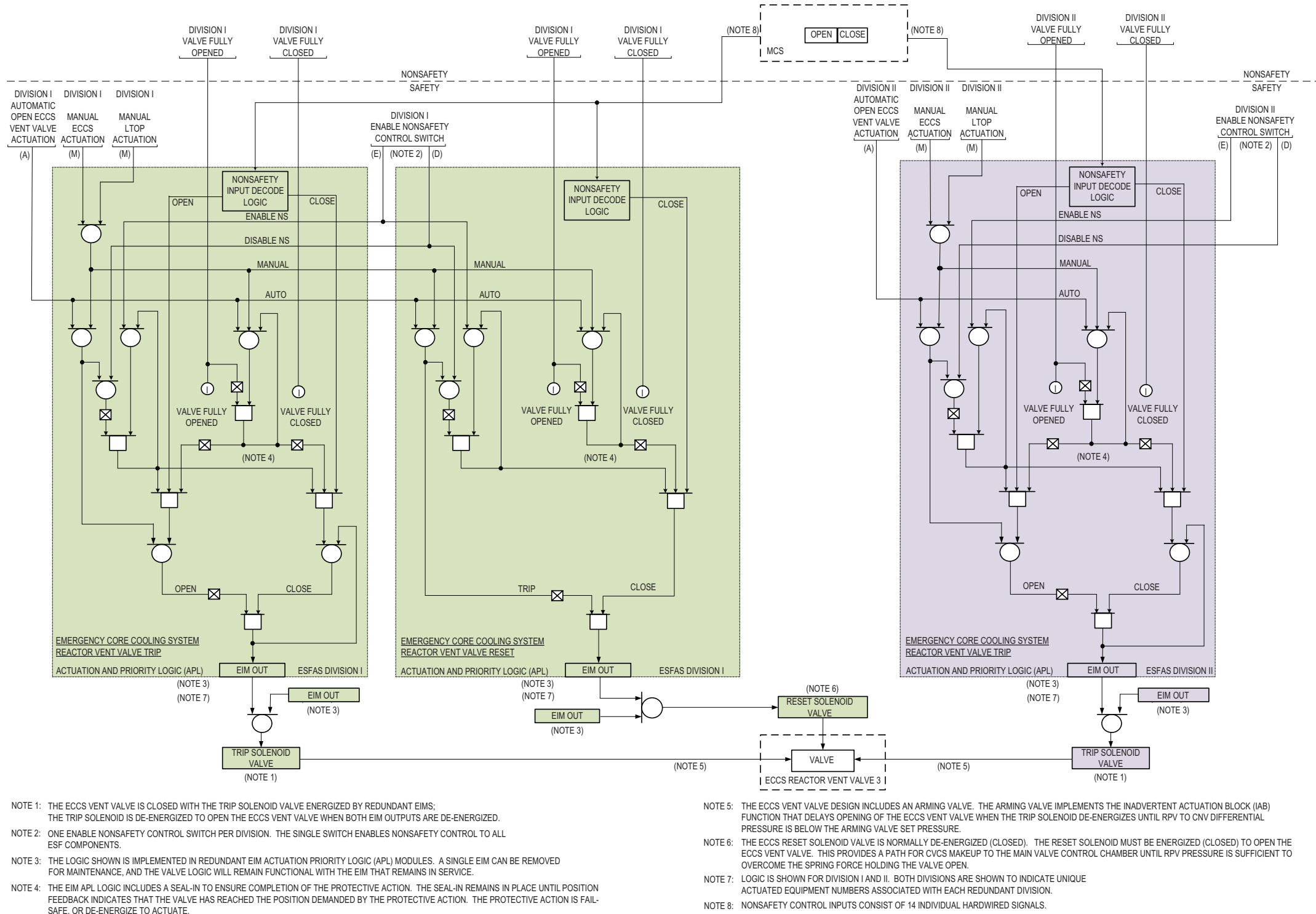
Figure 7.1-1ac: Emergency Core Cooling System Reactor Vent Valve 3 Actuation
