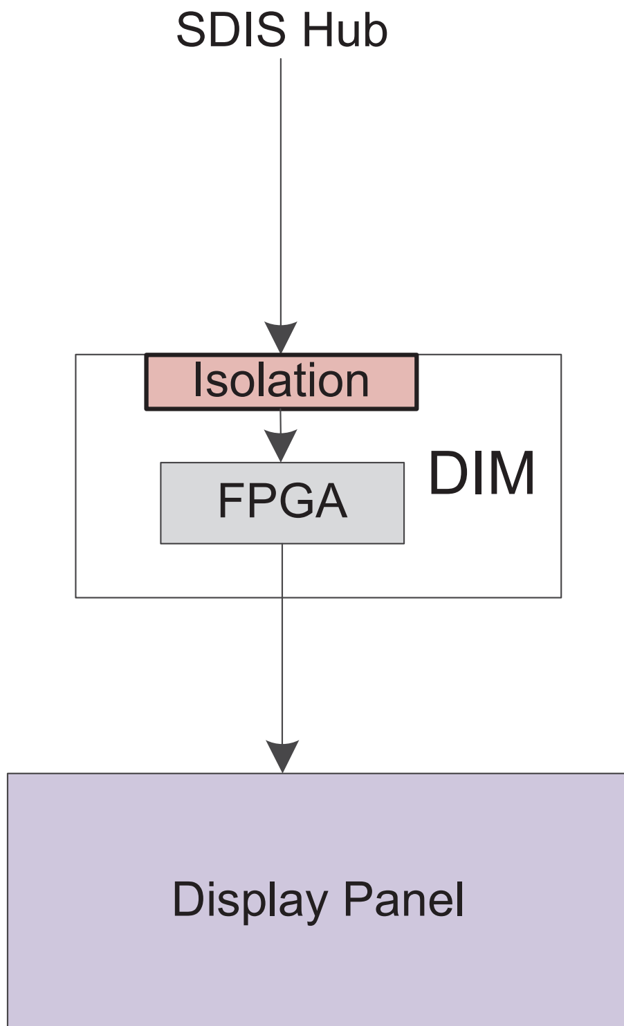
Figure 7.0-16: Display Interface Module
