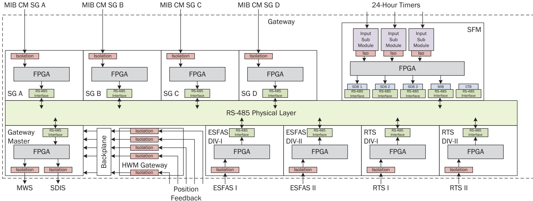
Figure 7.0-10: Module Protection System Gateway Diagram
