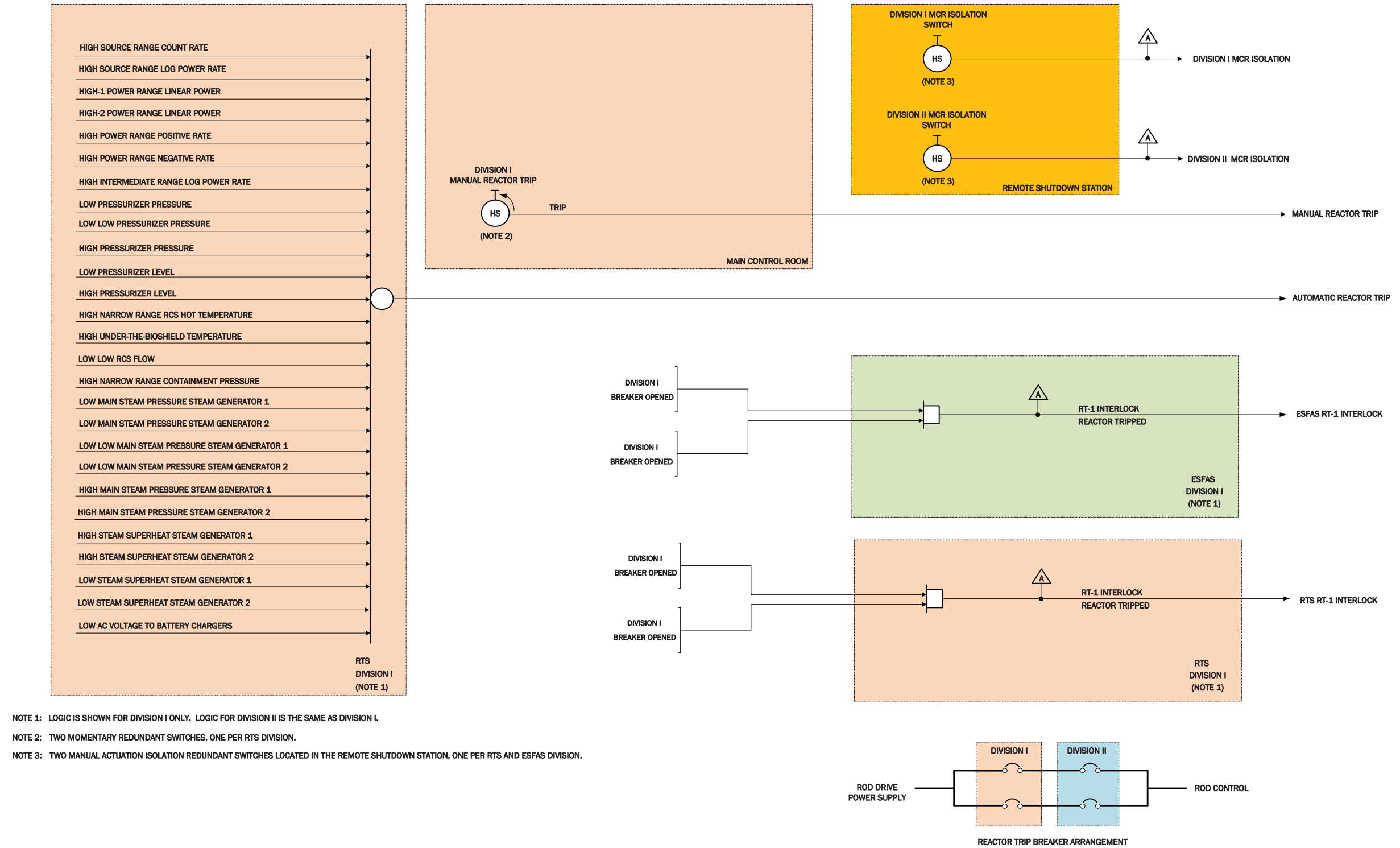
Figure 7.1-1j: Reactor Trip and Reactor Tripped Interlock RT-1
