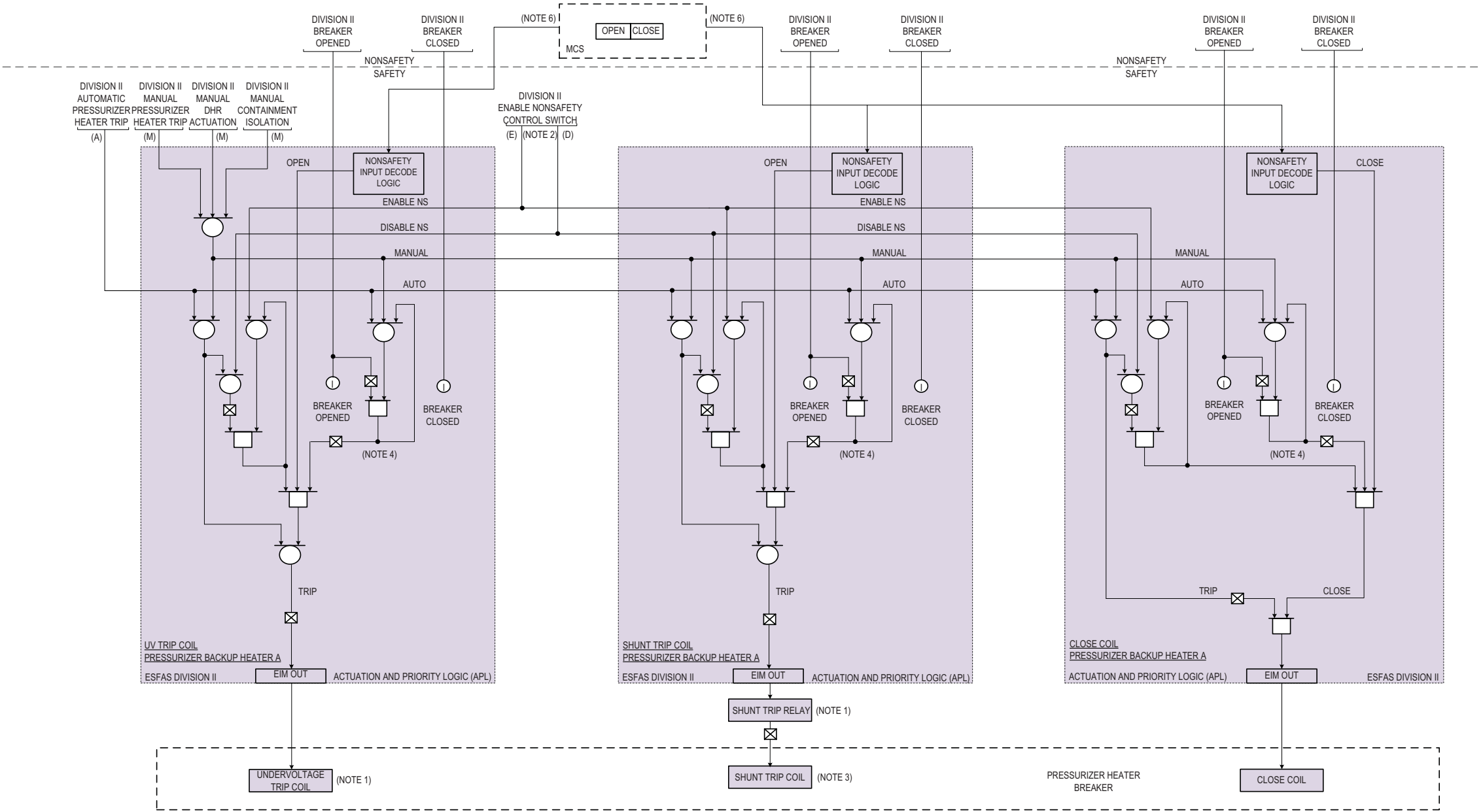
Figure 7.1-1am: Pressurizer Heater Trip Breaker Backup Heater A
