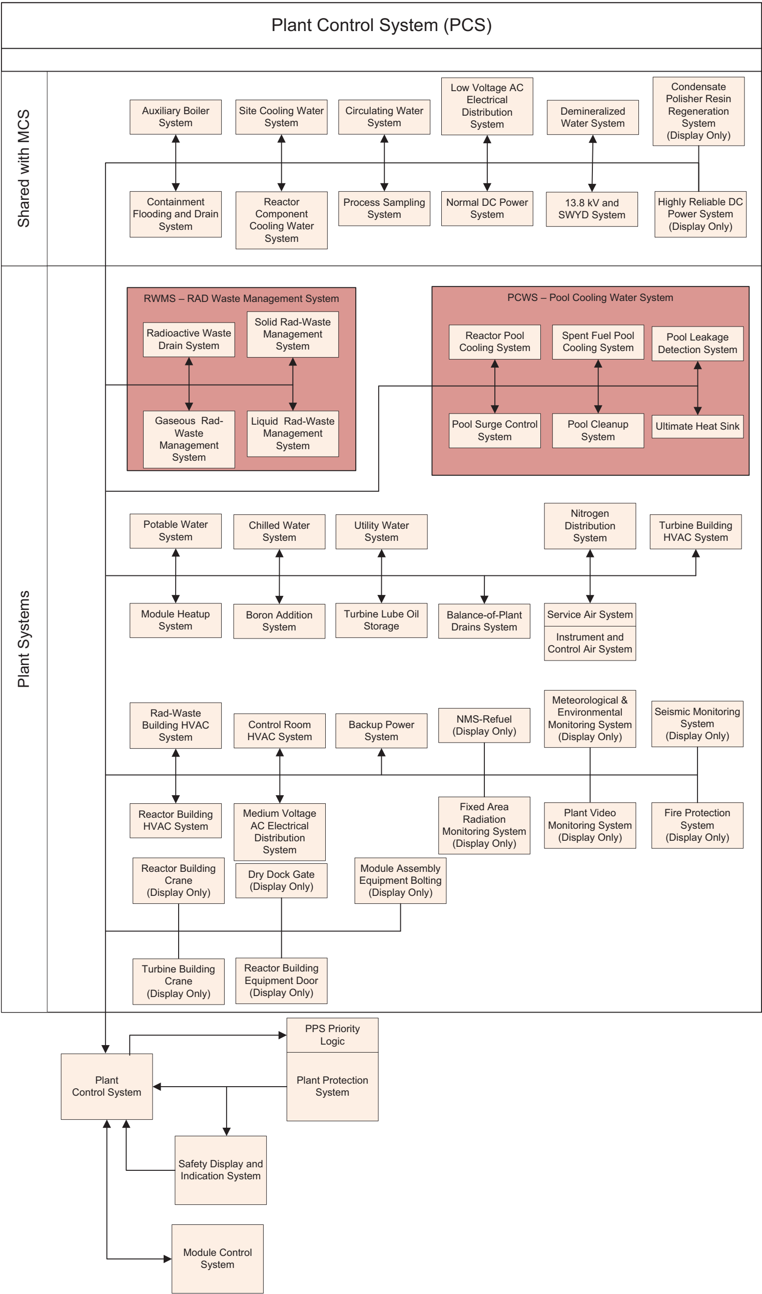
Figure 7.0-20: Plant Control System Internal Functions and External Interfaces
