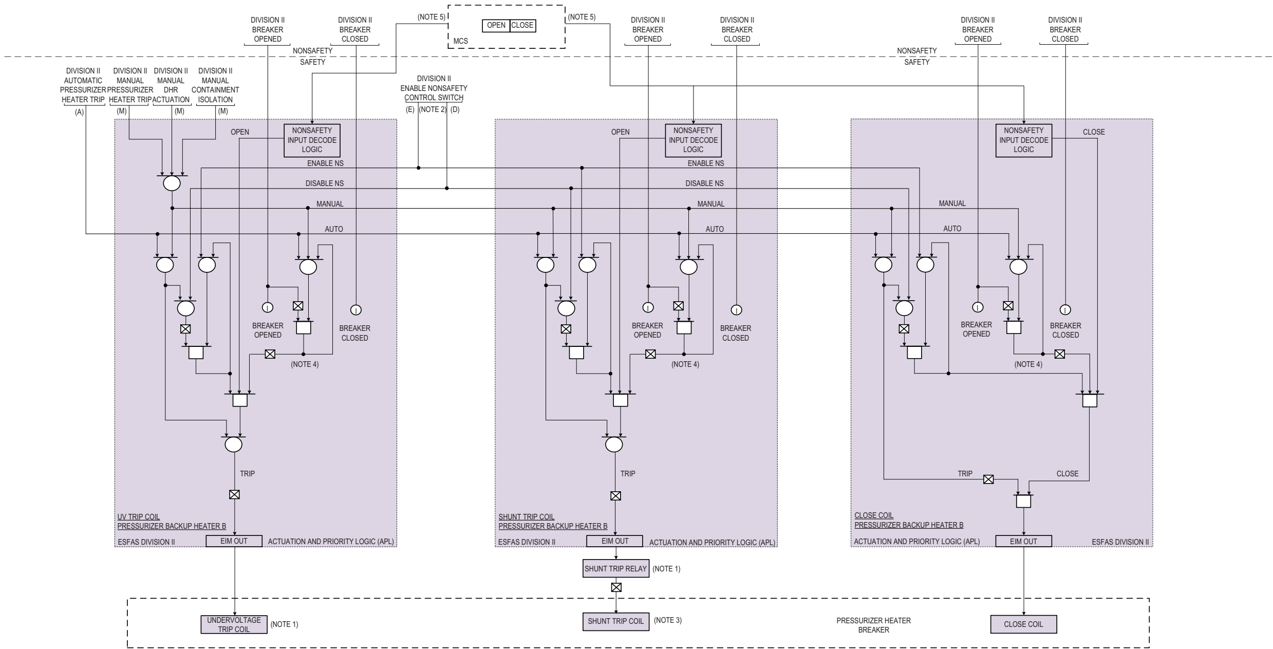
Figure 7.1-1an: Pressurizer Heater Trip Breaker Backup Heater B
