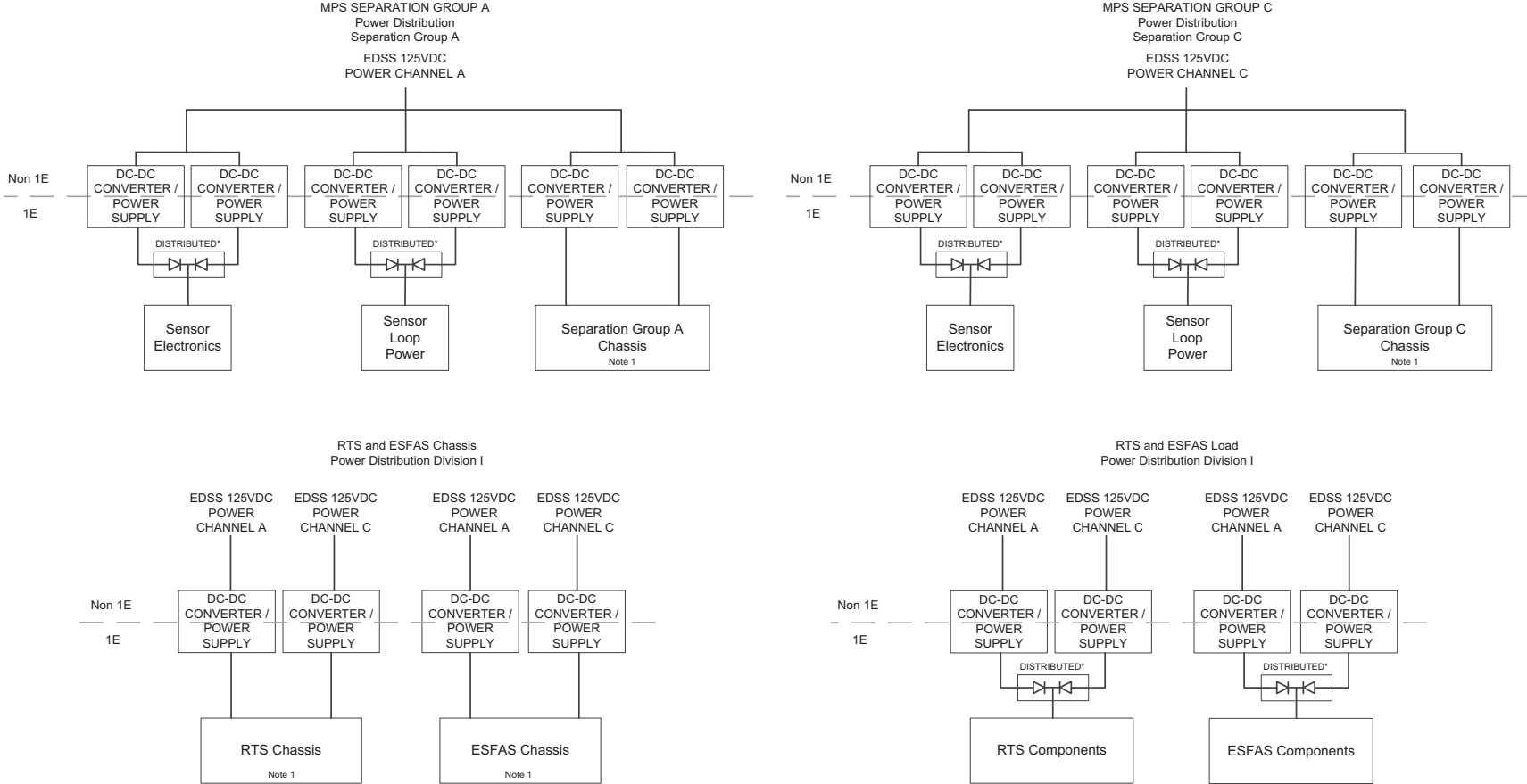
Figure 7.0-11a: Module Protection System Power Distribution
