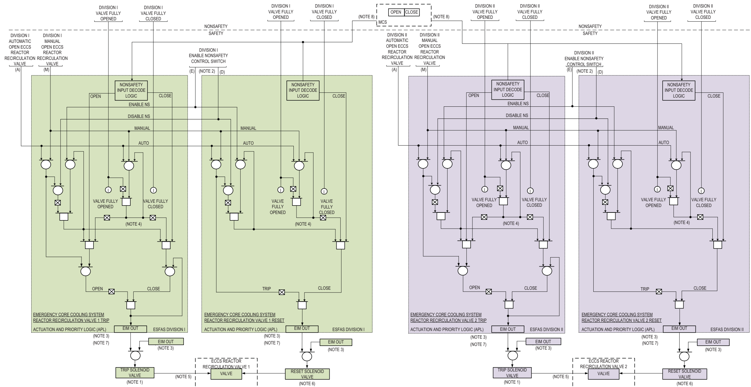
Figure 7.1-1ab: Emergency Core Cooling System Reactor Recirculation Valve Actuation
