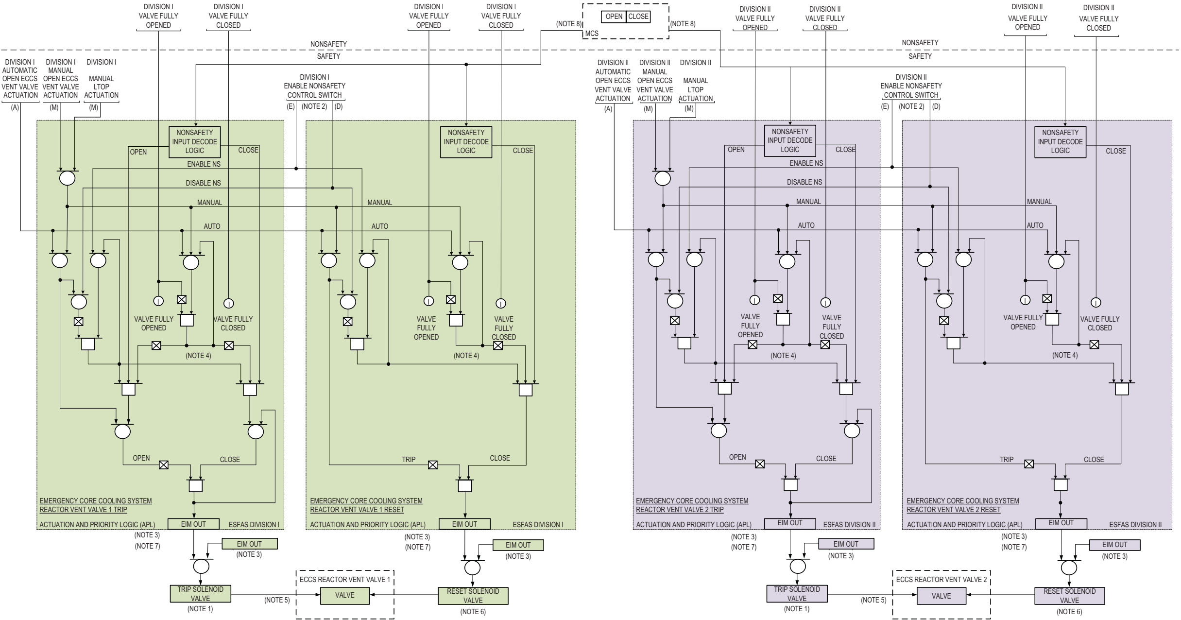
Figure 7.1-1aa: Emergency Core Cooling System Reactor Vent Valve 1 & 2 Actuation
