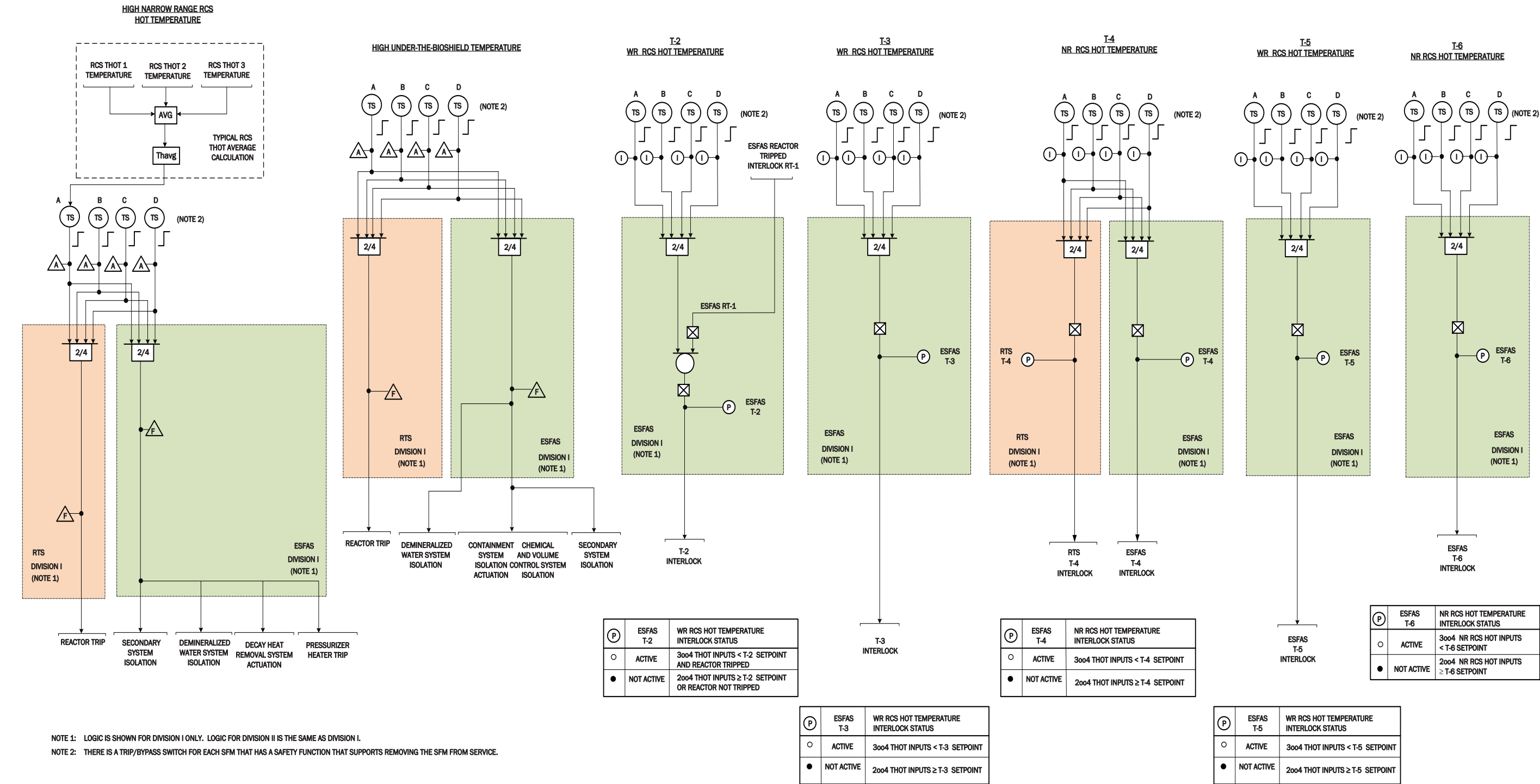
Figure 7.1-1f: Reactor Coolant System Hot Temperature Trip, Temperature Interlocks
