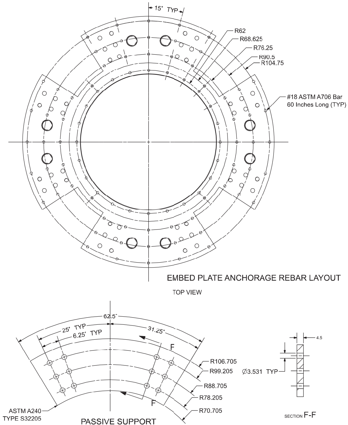
Figure 3B-50: Plan View of NPM Embed Plate Anchorage and Passive Plate
