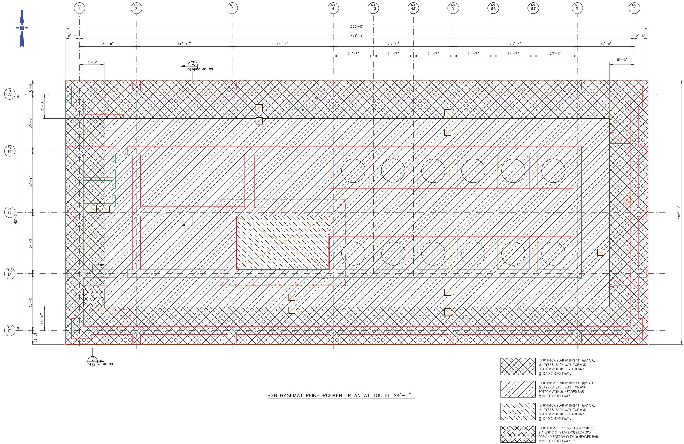
Figure 3B-88: Reactor Building Reinforcement Plan of Basemat Foundation
