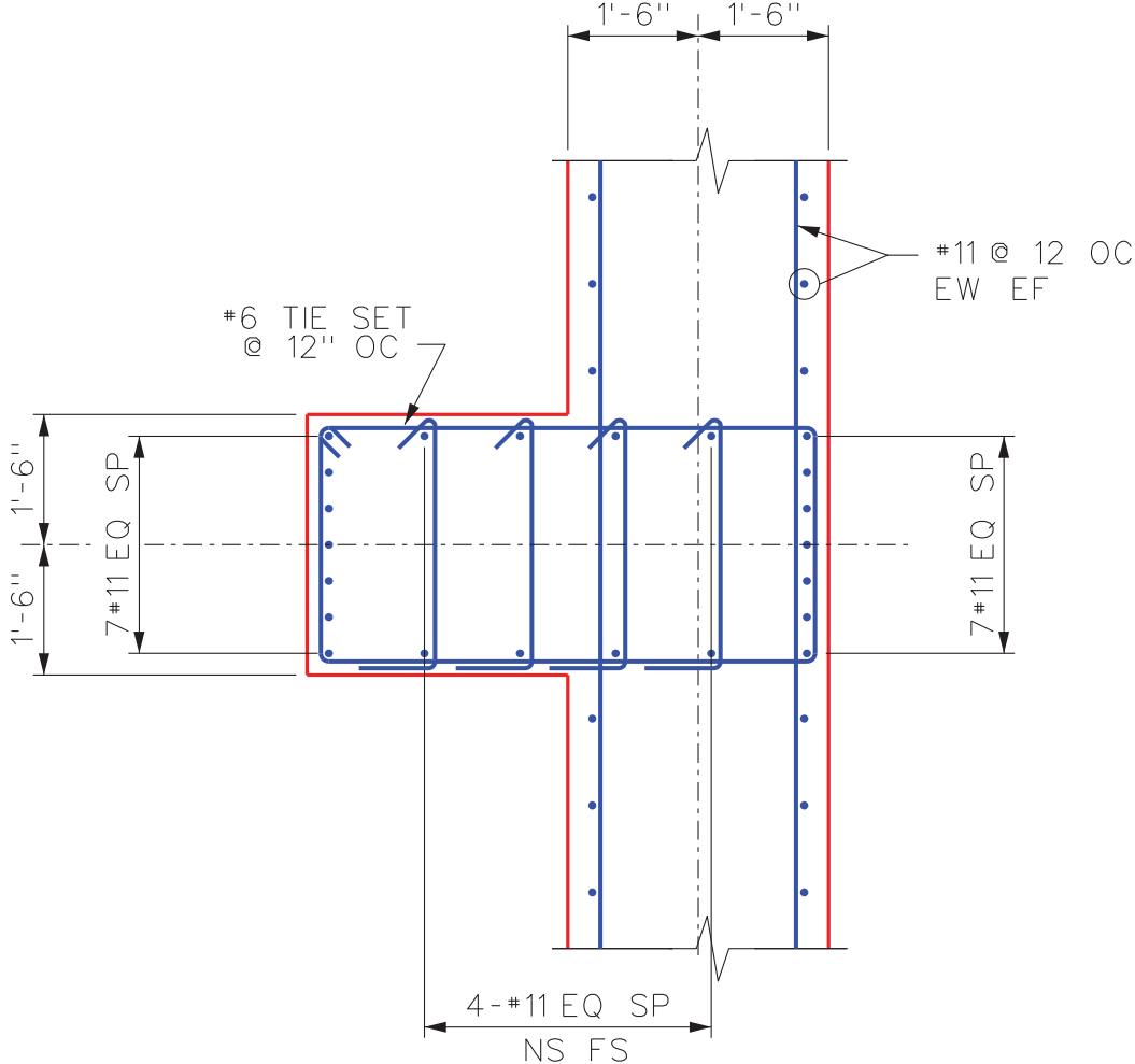
Figure 3B-81: CRB Reinforcement Detail for Pilaster Type 1
