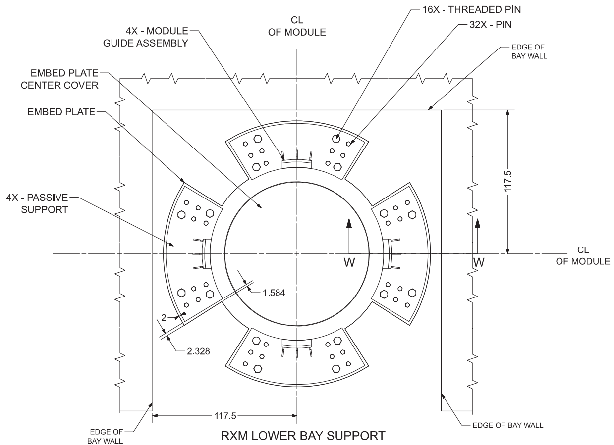
Figure 3B-48: NuScale Power Module Base Support Assembly at Reactor Building Pool Floor
