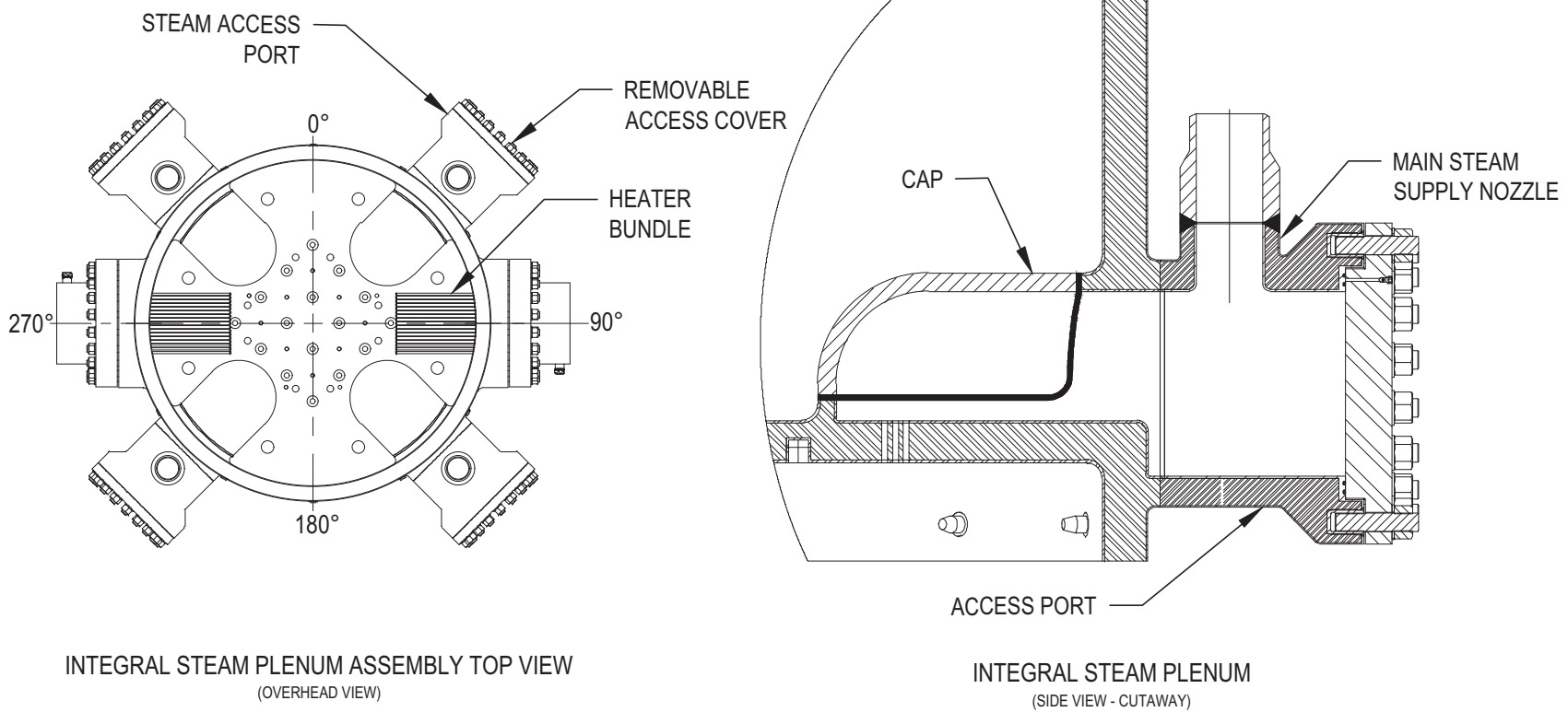
Figure 5.4-4: Integral Steam Plenum
