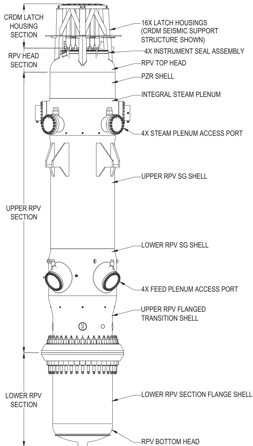
Figure 5.3-1: Reactor Vessel
