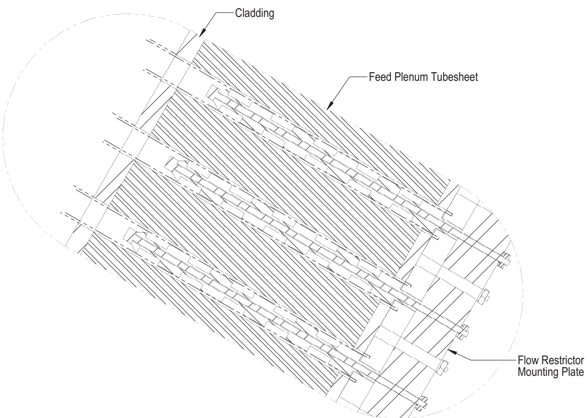
Flow Restrictor Mounting
