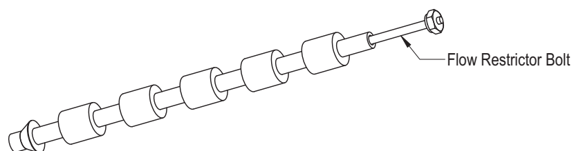
Figure 5.4-8: Steam Generator Flow Restrictor Assembly
