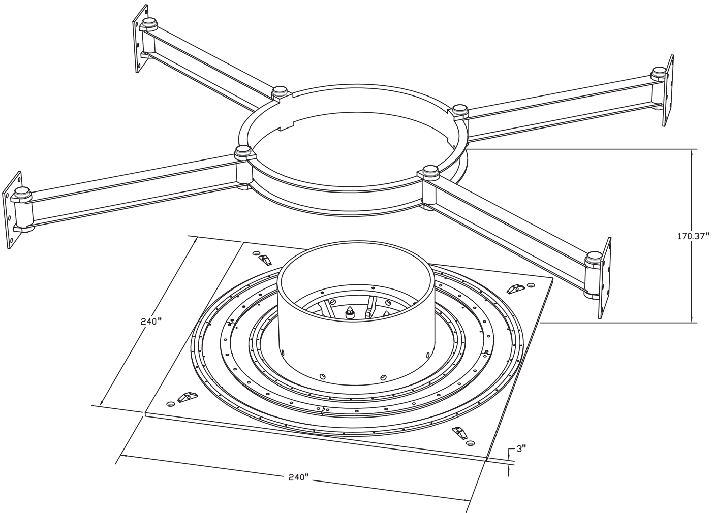
Figure 3.8.4-34: Reactor Flange Tool Support and Stand
