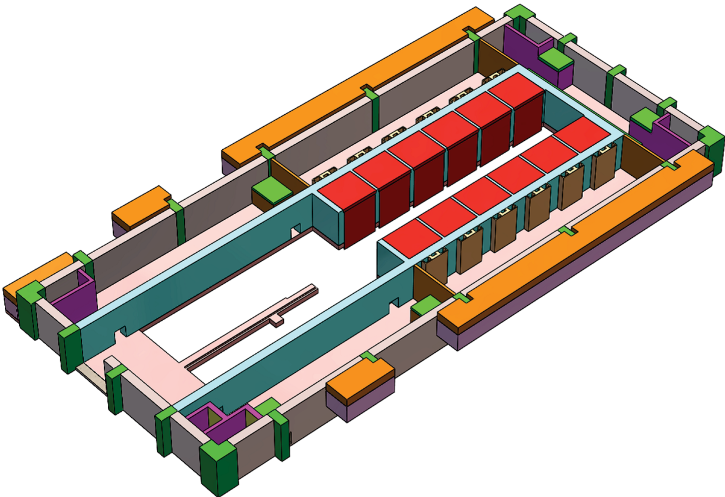
Figure 3.8.4-4: Reactor Building Concrete Structural Sections at Fourth Floor (EL. 100'-0")
