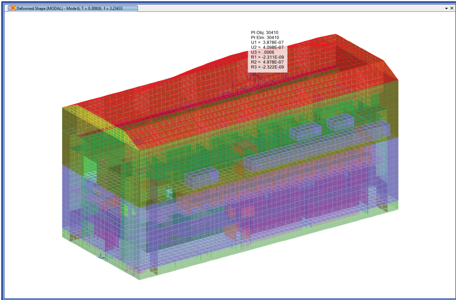
Figure 3.7.2-78: Reactor Building Cracked Model - Modal Shape - (Mode 6)
