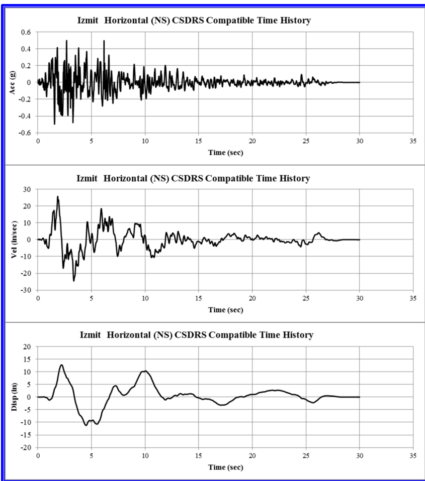
Figure 3.7.1-8d: CSDRS Compatible Time Histories for Izmit North-South
