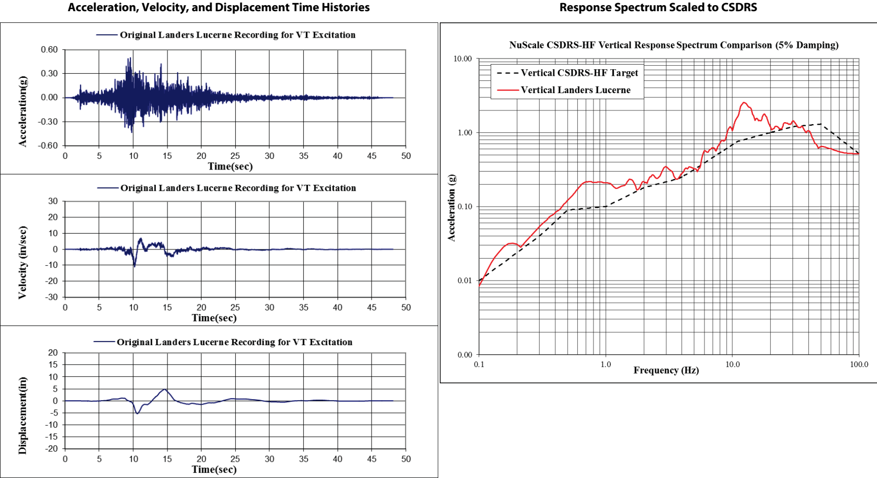
Figure 3.7.1-10e: Original Time Histories for Lucerne Vertical
