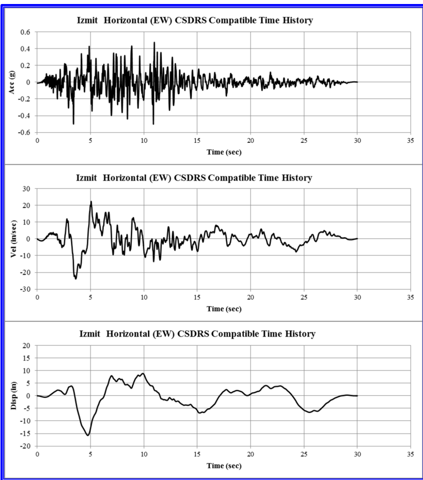
Figure 3.7.1-8b: CSDRS Compatible Time Histories for Izmit East-West
