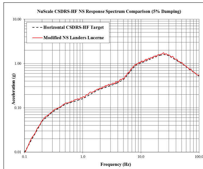
Figure 3.7.1-10d: CSDRS-HF Compatible Time Histories for Lucerne North-South
