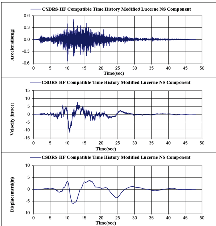
Figure 3.7.1-10d: CSDRS-HF Compatible Time Histories for Lucerne North-South
