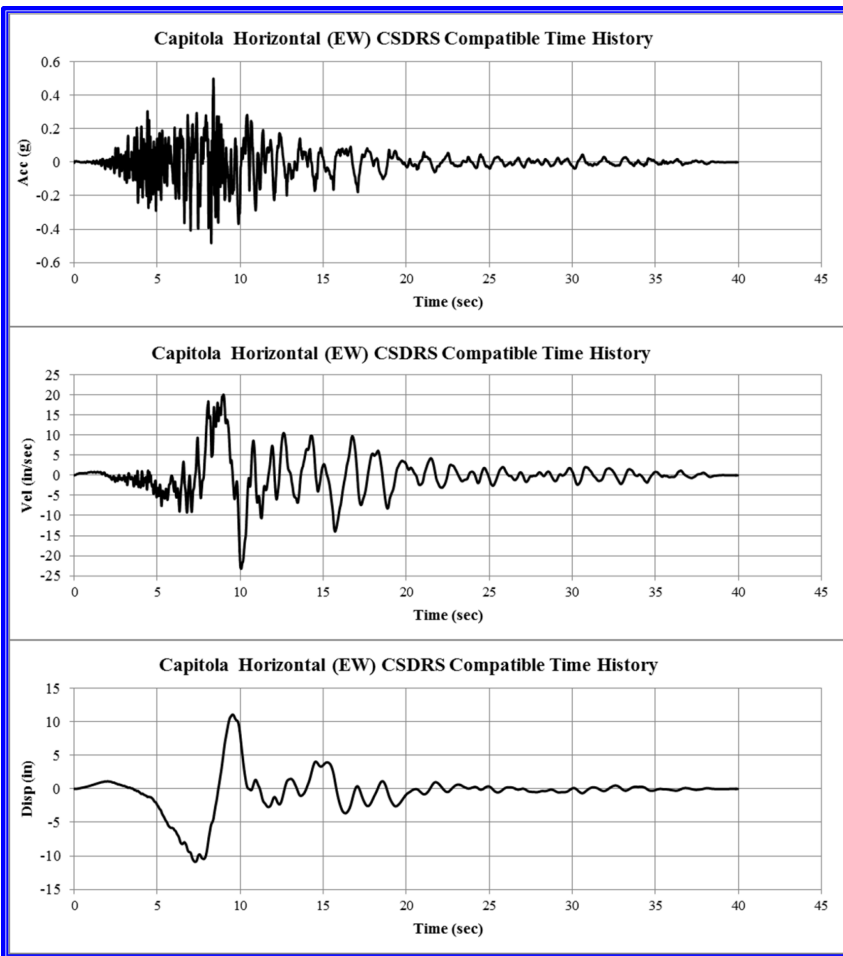
Figure 3.7.1-6b: CSDRS Compatible Time Histories for Capitola East-West
