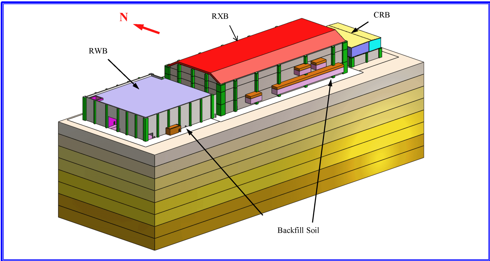
Figure 3.7.2-1: Control Building, Reactor Building, and Radioactive Waste Building in Soil (Looking Northeast)
