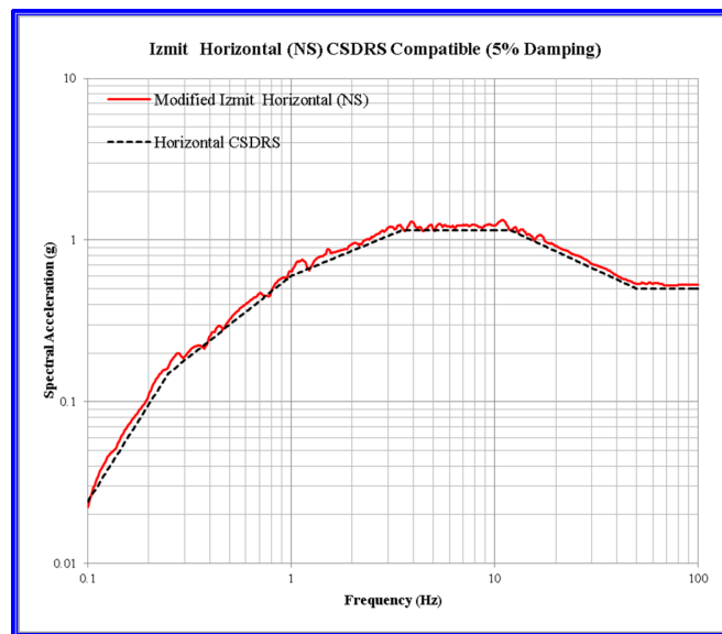
Figure 3.7.1-8d: CSDRS Compatible Time Histories for Izmit North-South
