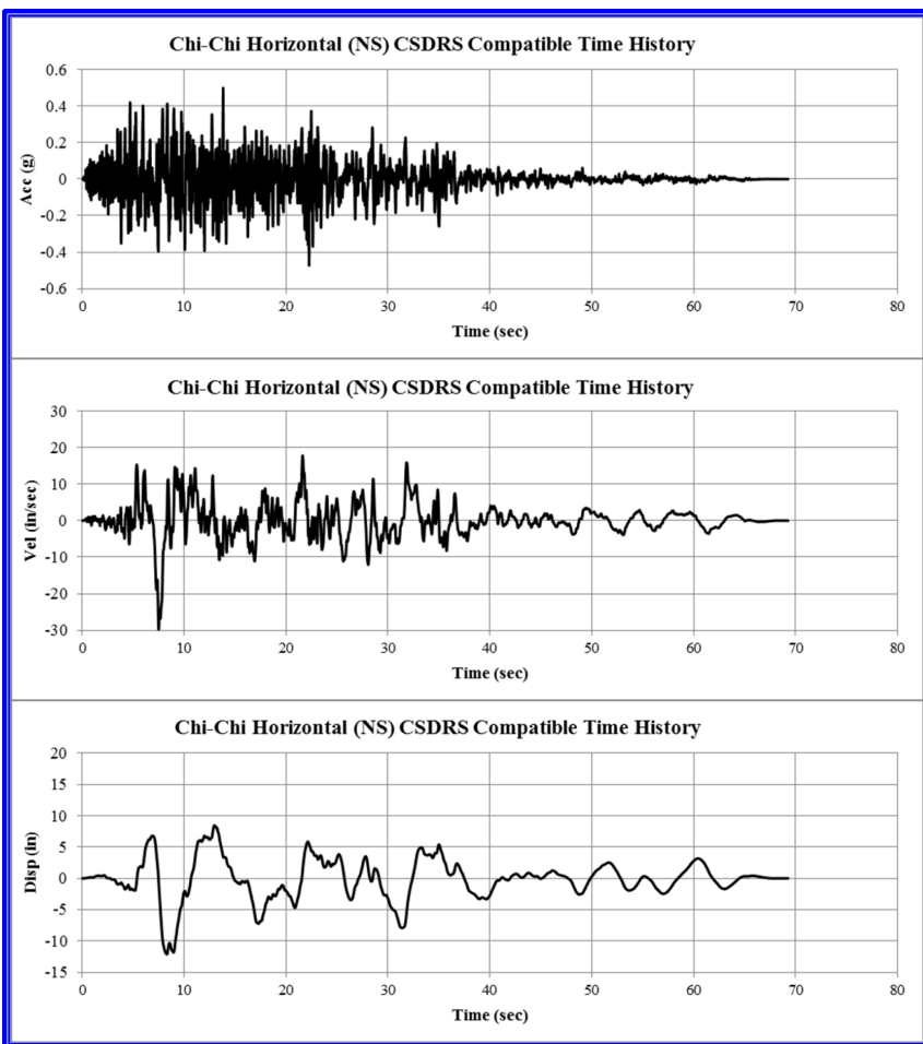
Figure 3.7.1-7d: CSDRS Compatible Time Histories for Chi-Chi North-South
