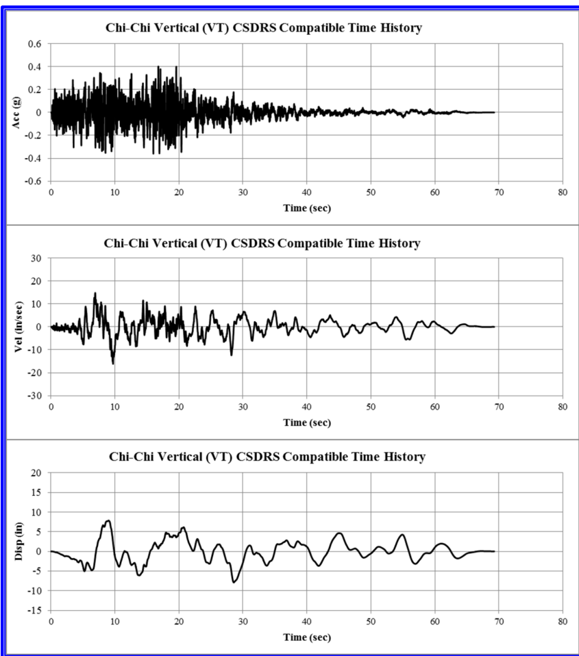
Figure 3.7.1-7f: CSDRS Compatible Time Histories for Chi-Chi Vertical
