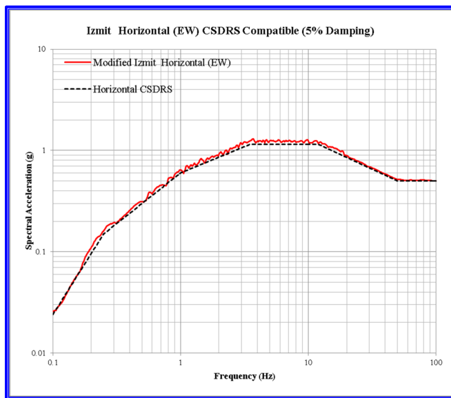
Figure 3.7.1-8b: CSDRS Compatible Time Histories for Izmit East-West
