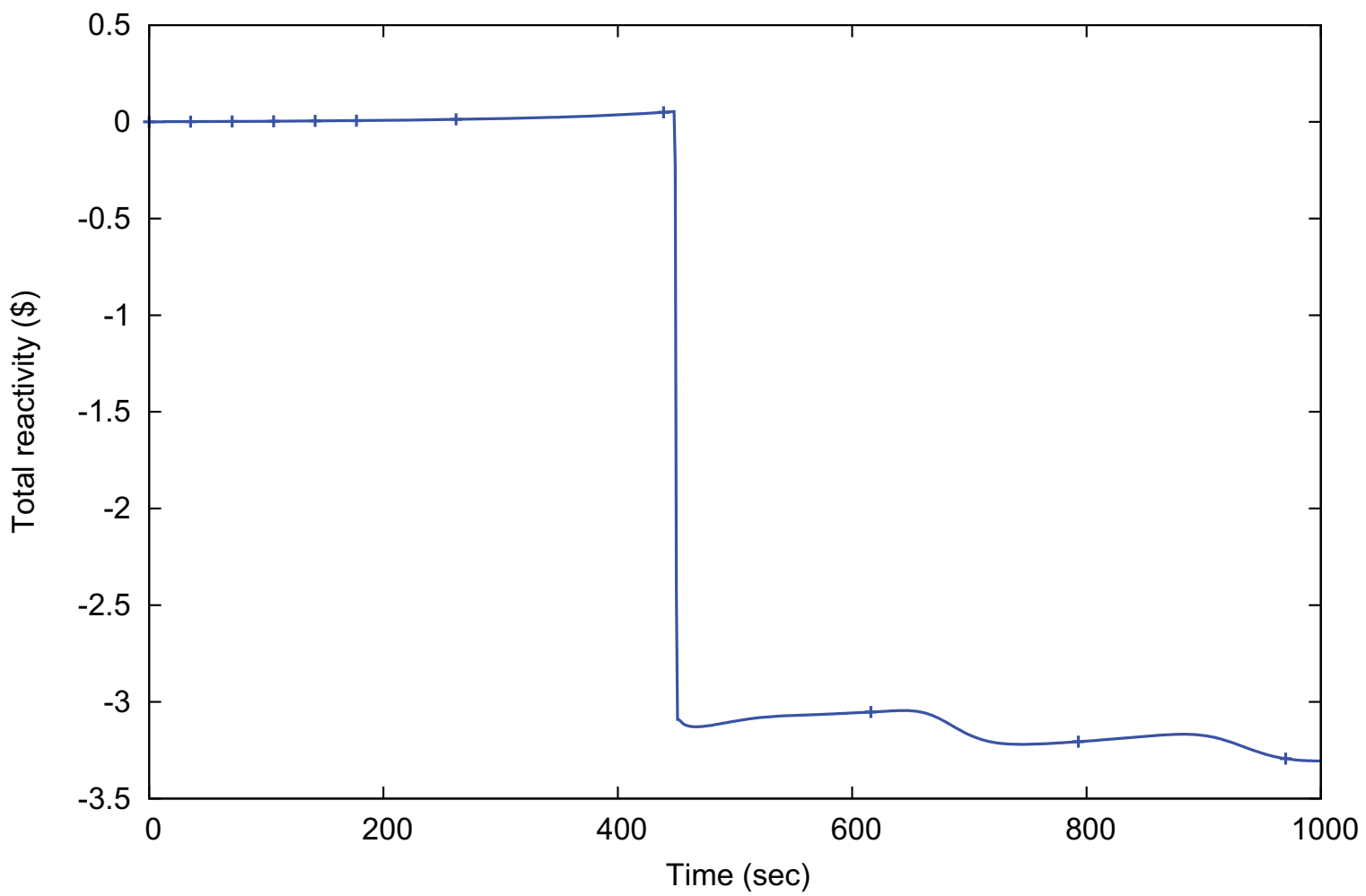
Figure 15.4-2: Net Reactivity (15.4.1 Uncontrolled Control Rod Assembly Withdrawal from a Subcritical or Low Power Condition)
