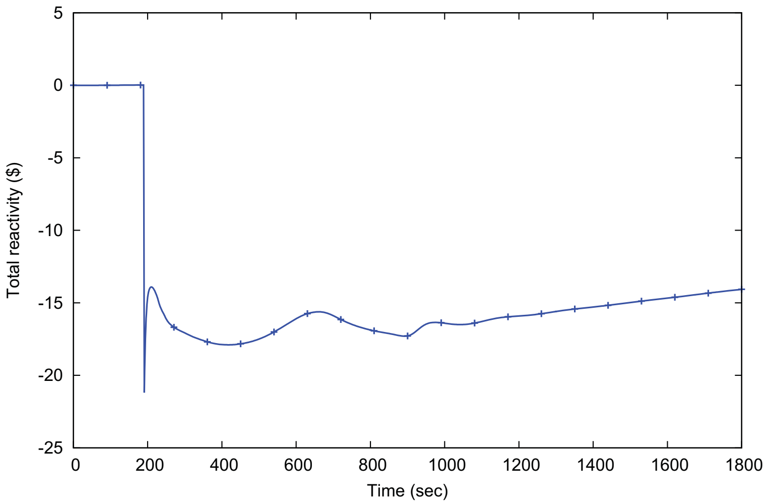
Figure 15.1-4: Total Reactivity - Entire Transient (15.1.1 Decrease in Feedwater Temperature)
