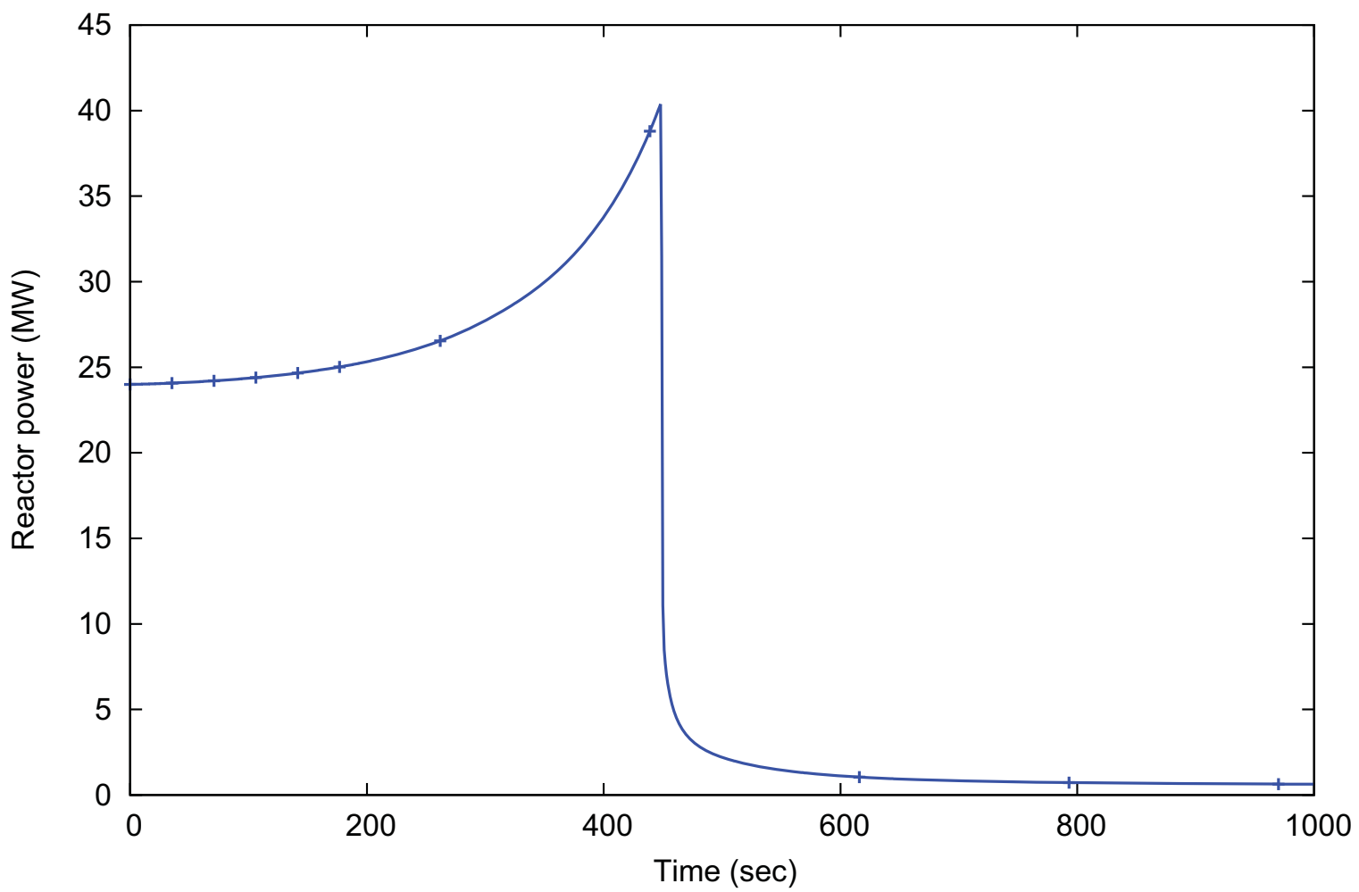
Figure 15.4-1: Reactor Power (15.4.1 Uncontrolled Control Rod Assembly Withdrawal from a Subcritical or Low Power Condition)
