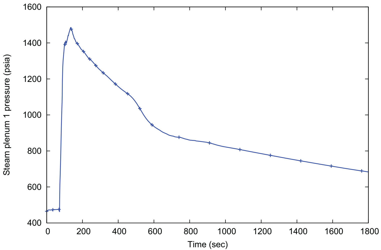
Figure 15.1-56: Steam Generator Pressure - Maximum SGS Pressure Case (15.1.2 Increase in Feedwater Flow)
