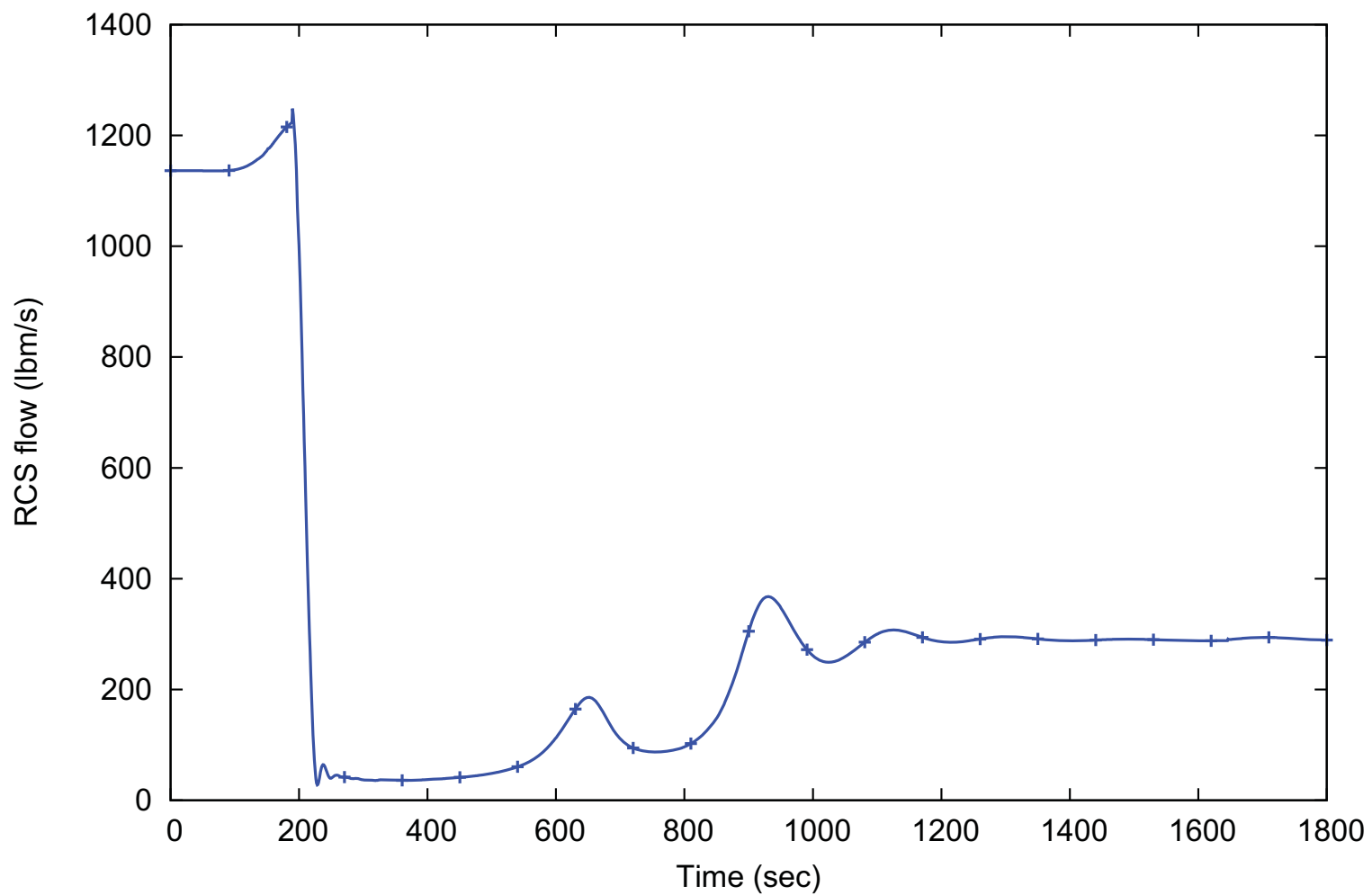
Figure 15.1-10: Reactor Coolant System Flow Rate (15.1.1 Decrease in Feedwater Temperature)
