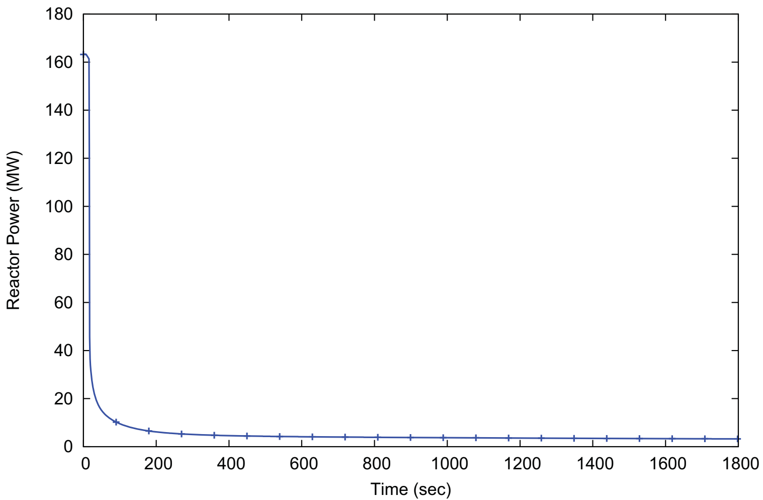
Figure 15.6-5: Failure of Lines Carrying Primary Coolant Outside Containment - Maximum Reactor Pressure Vessel Pressure Scenario - Reactor Power
