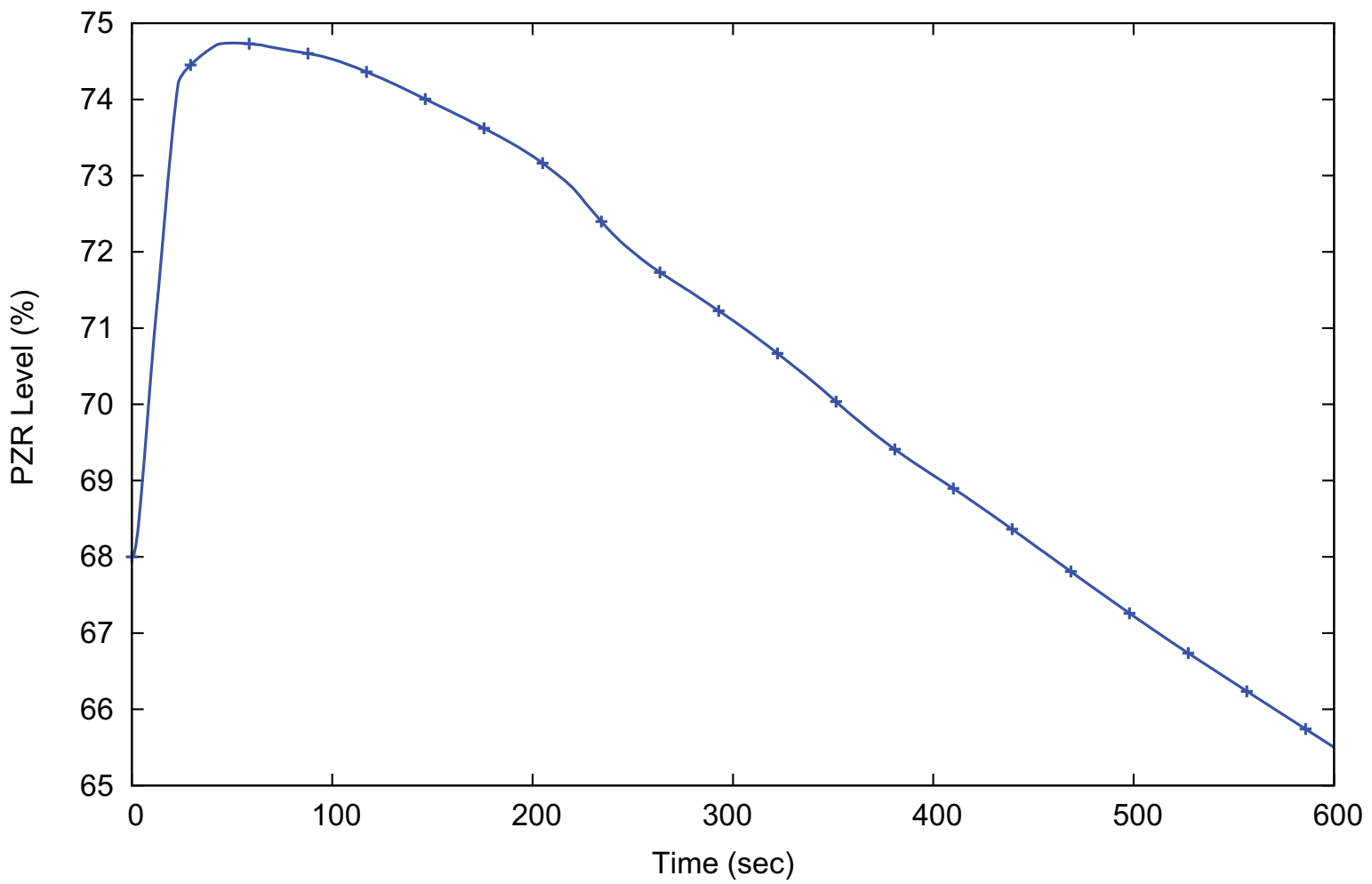
Figure 15.2-1: Pressurizer Level - Peak RCS Pressure Case (15.2.1-15.2.3 LOEL-TT-LOCV)
