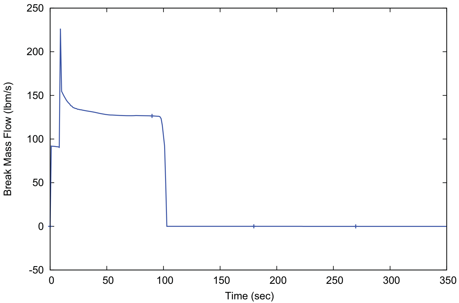
Figure 15.6-1: Failure of Lines Carrying Primary Coolant Outside Containment - Maximum Mass Release Scenario Break Mass Flow
