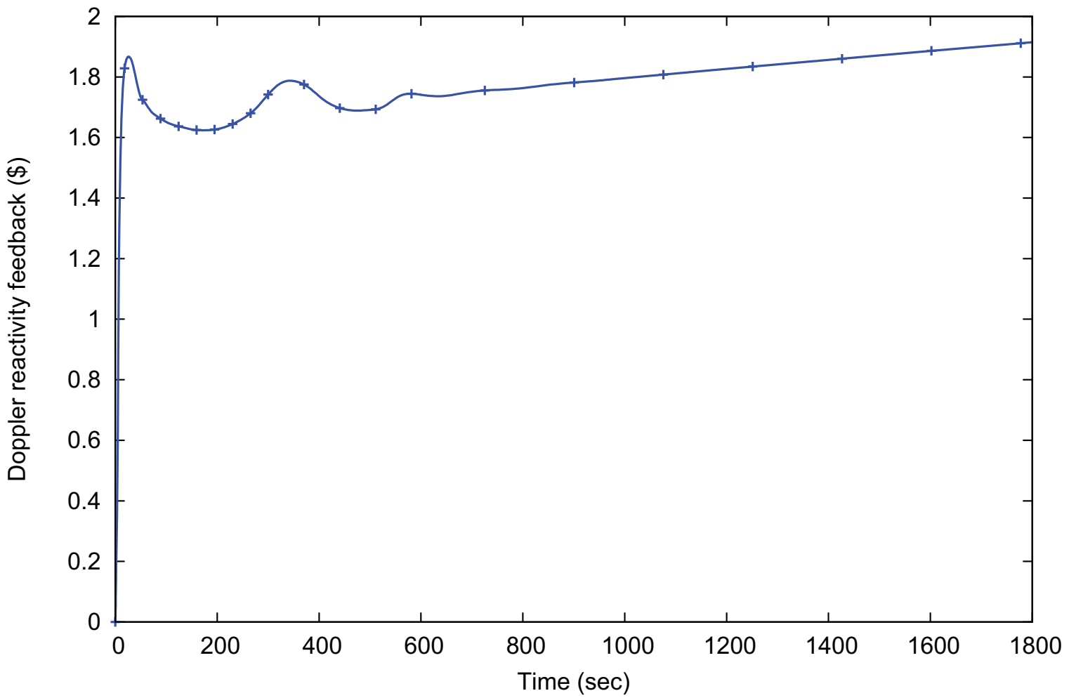
Figure 15.4-27: Doppler Reactivity (15.4.3 Control Rod Misoperation, Control Rod Assembly drop)
