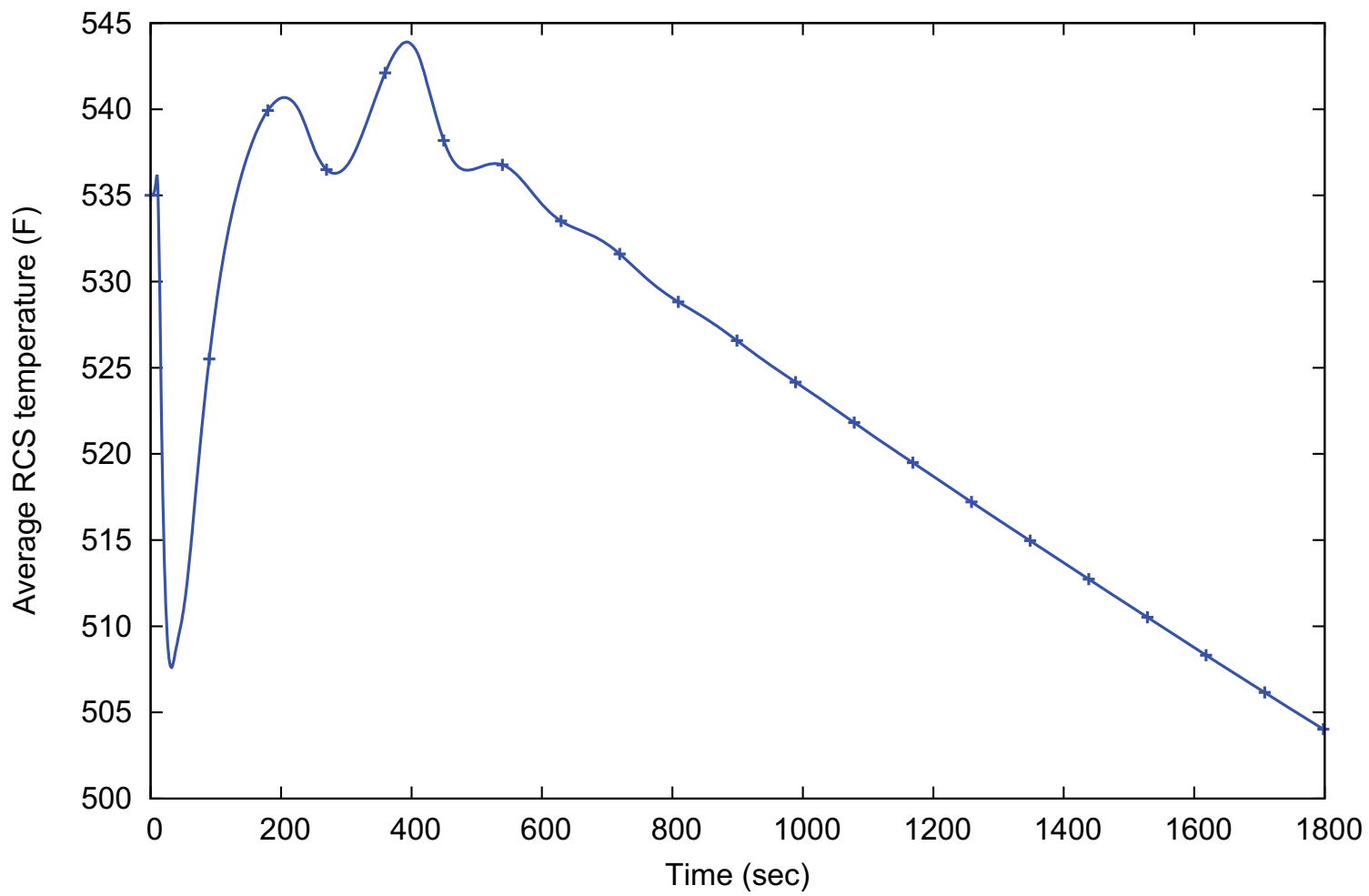
Figure 15.2-24: Reactor Coolant System Average Temperature - Peak RCS Pressure Case (15.2.6 Loss of AC Power)
