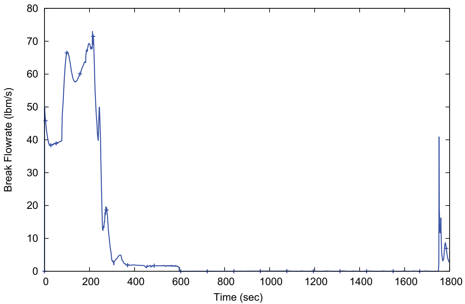
Figure 15.1-45: Break Flow Rate (15.1.5 Steam Piping Failure, Limiting Radiological)
