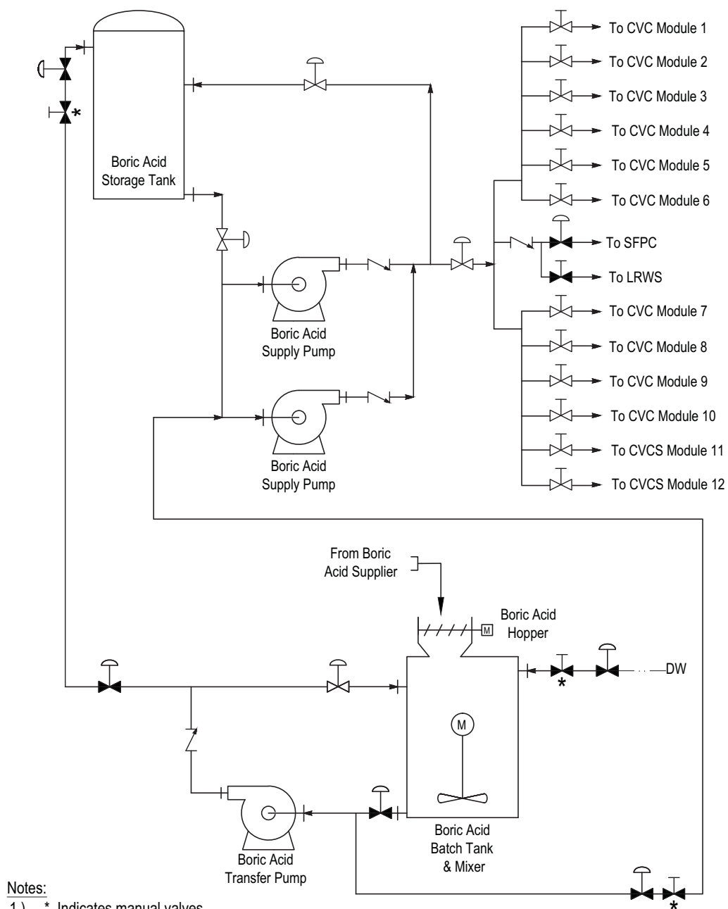
Figure 9.3.4-2: Boron Addition System Diagram
