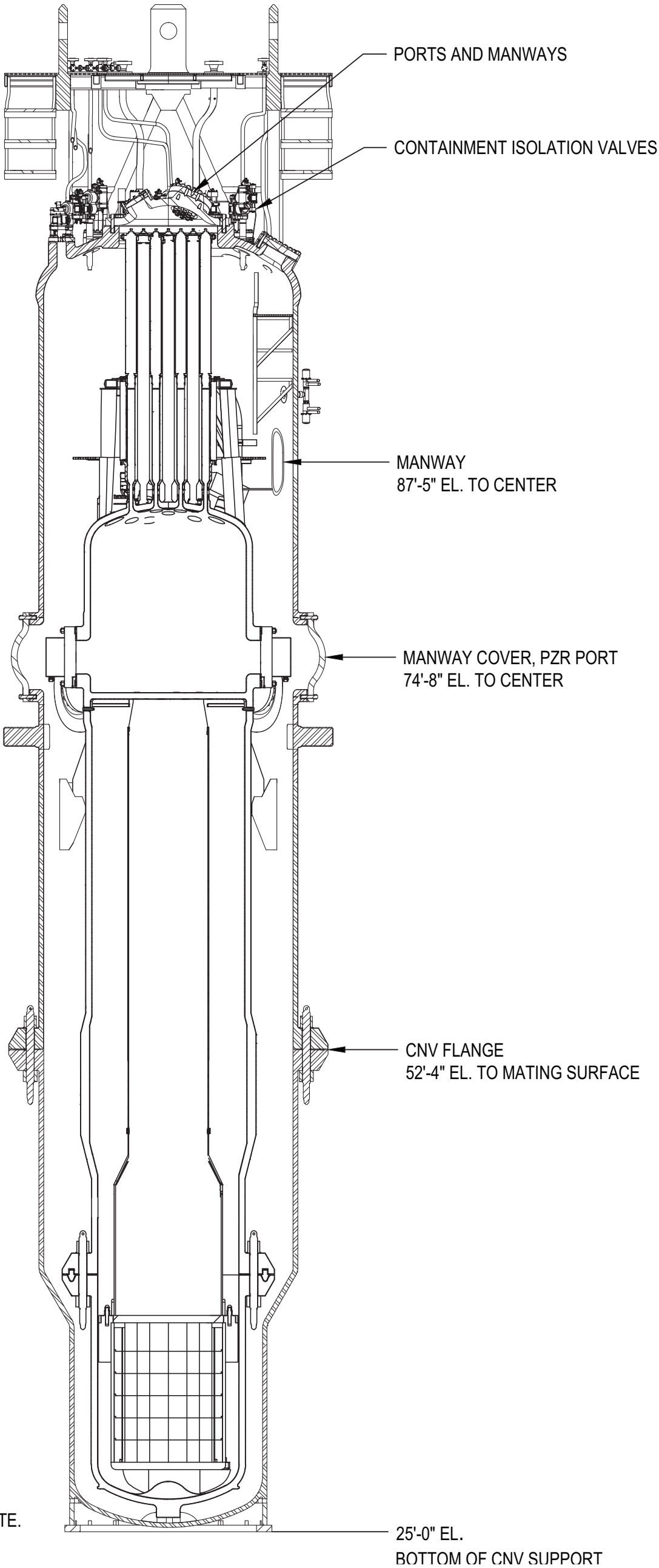
Figure 6.2-1: Containment System
