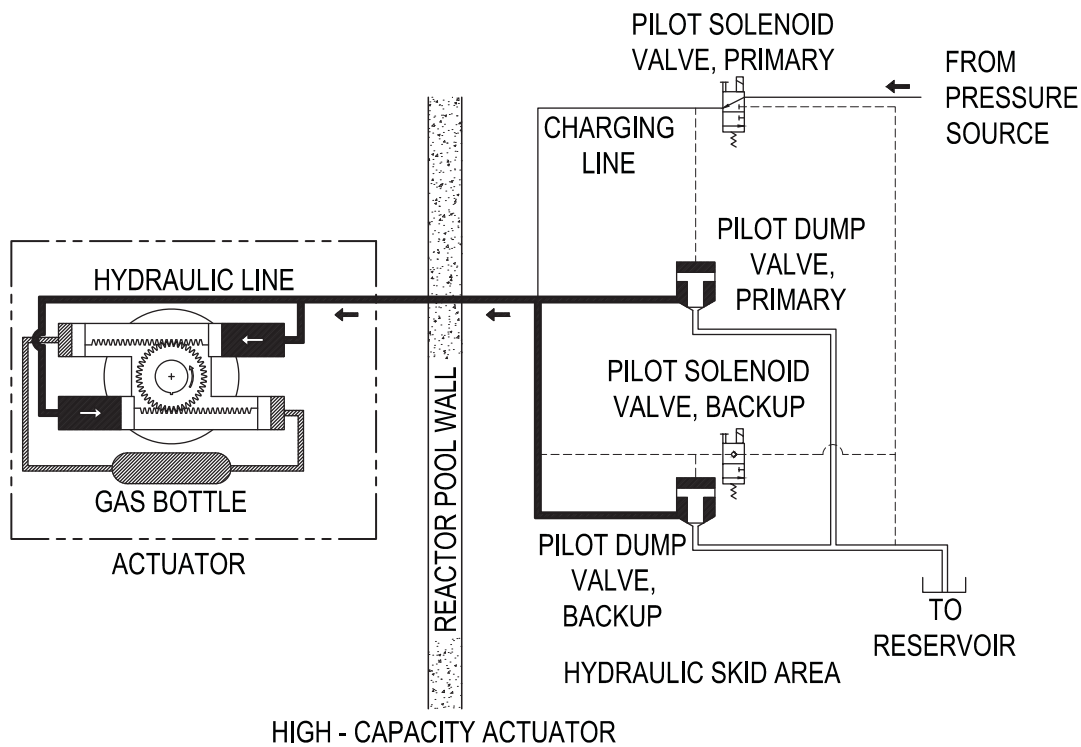
Figure 6.2-7: Containment Isolation Valve Actuator Hydraulic Schematic
