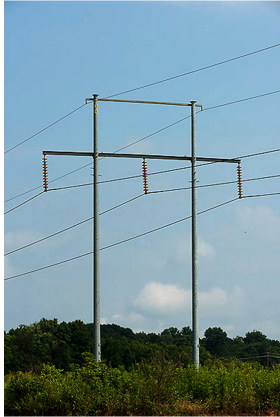
Double-Pole Single-Circuit 161 kV Transmission H-frame Structure
