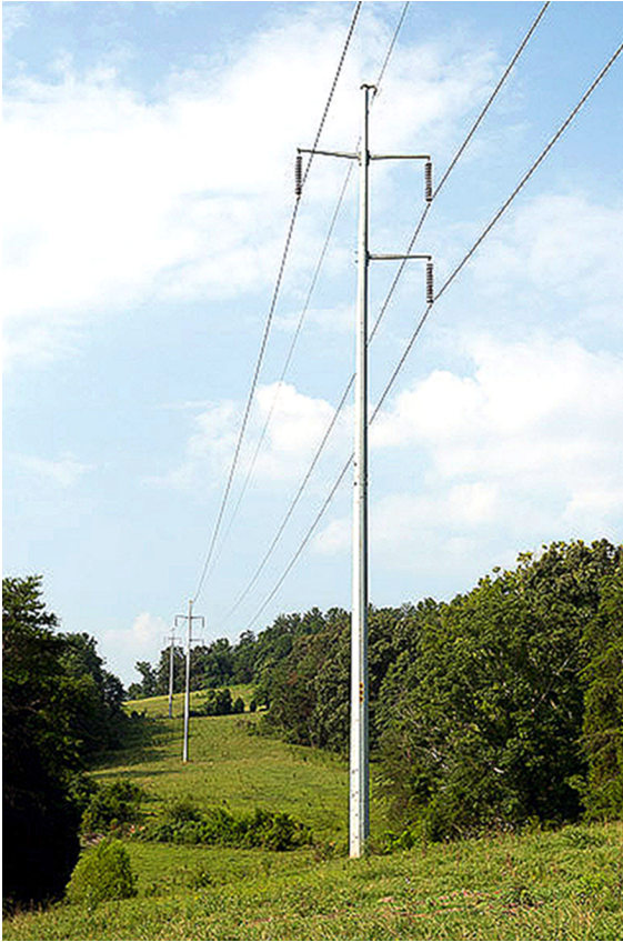
Single-Pole 161 kV Transmission Structure
