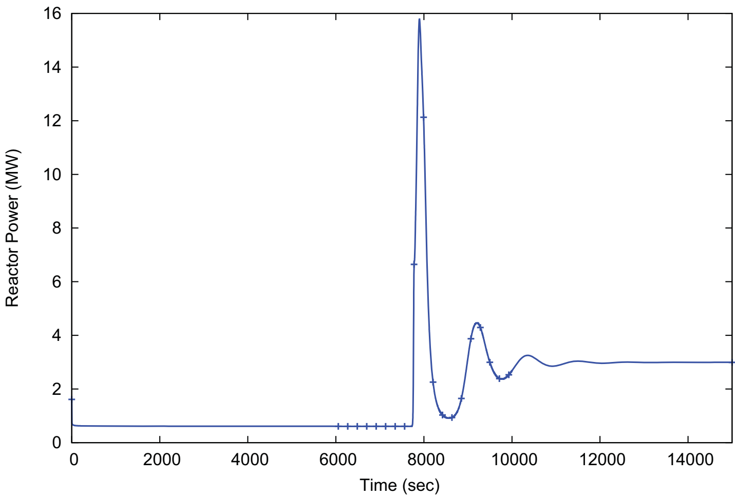
Figure 15.0-18: Reactor Power EDSS Available - Peak Power Case
