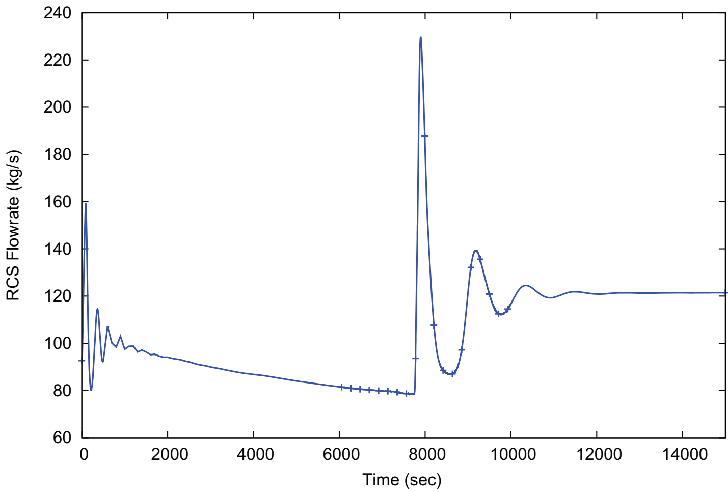
Figure 15.0-19: RCS Flowrate (Peak Power Case EDSS Available)
