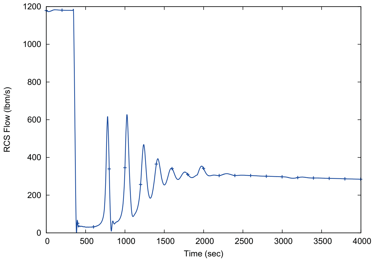
Figure 15.5-6: Reactor Coolant System Flow - Increase in RCS Inventory (No PZR Spray)
