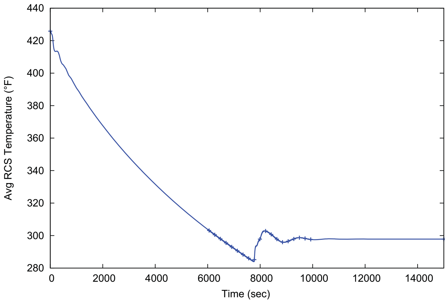
Figure 15.0-11: Return to Power – Average Reactor Coolant System Temperature (Peak Power Case)
