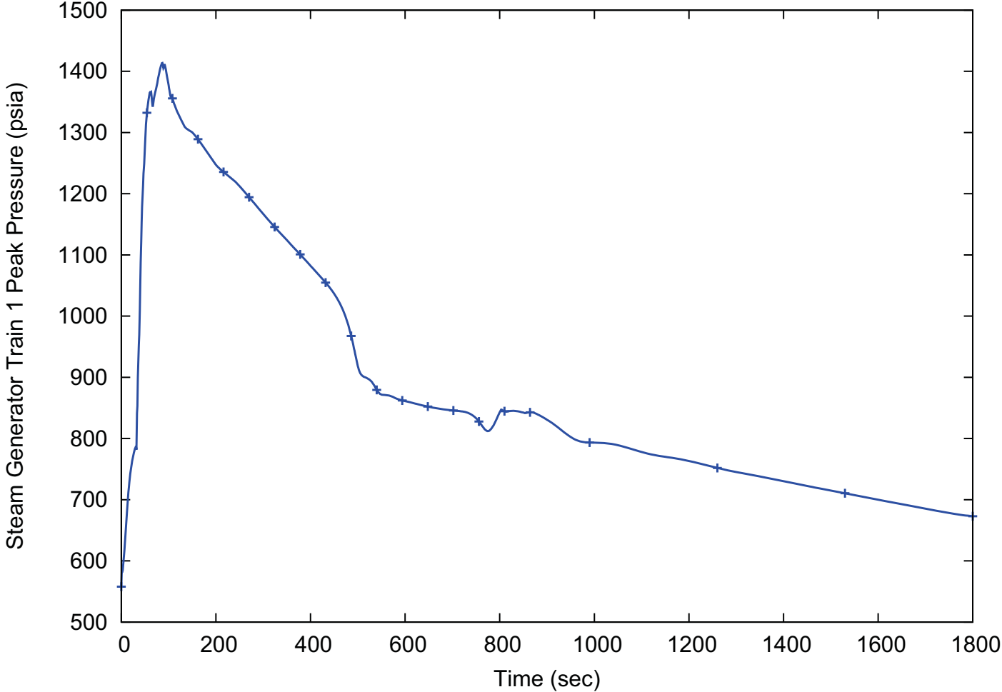
Figure 15.1-18: Main Steam System Pressure (15.1.2 Increase in Feedwater Flow)
