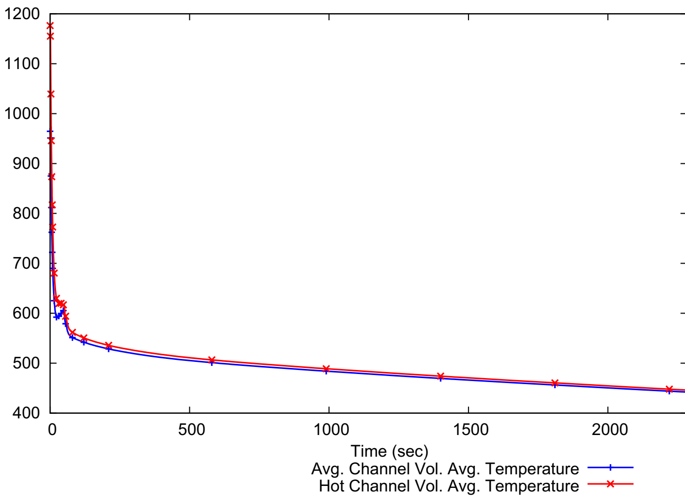
Figure 15.6-65: Inadvertent Operation of an Emergency Core Cooling System Valve – Fuel Volume Average Temperature
