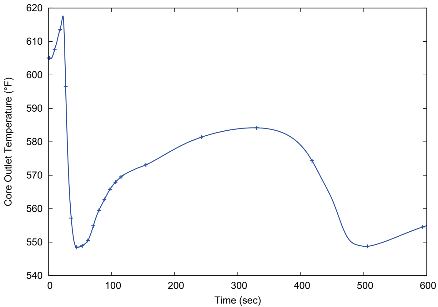
Figure 15.1-35: Core Outlet Temperature (15.1.5 Steam Piping Failure, Limiting Reactor Coolant System Pressure)
