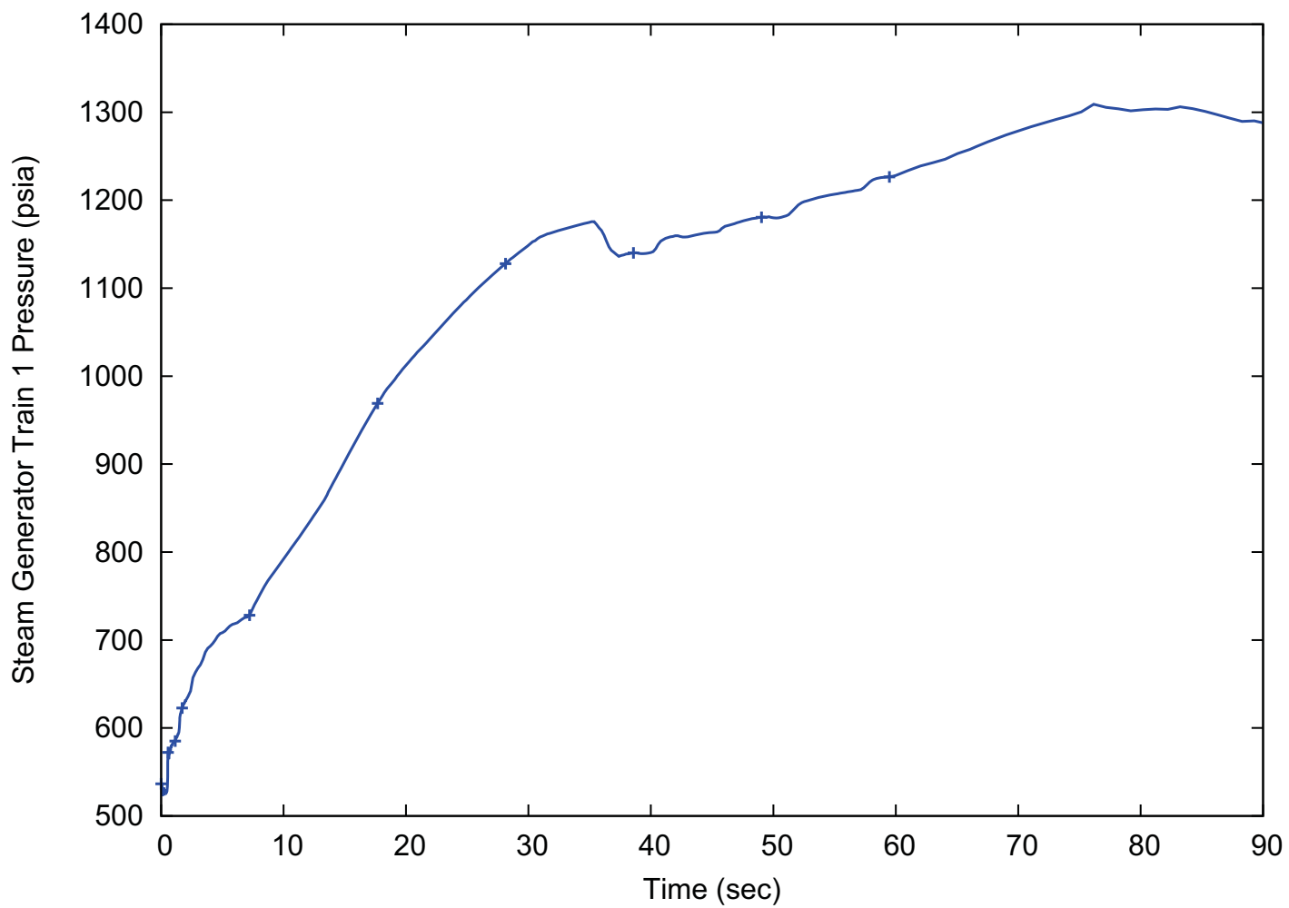
Figure 15.2-37: Steam Generator Train 1 Pressure - Peak RCS Pressure Case (15.2.8 Feedwater Line Break)
