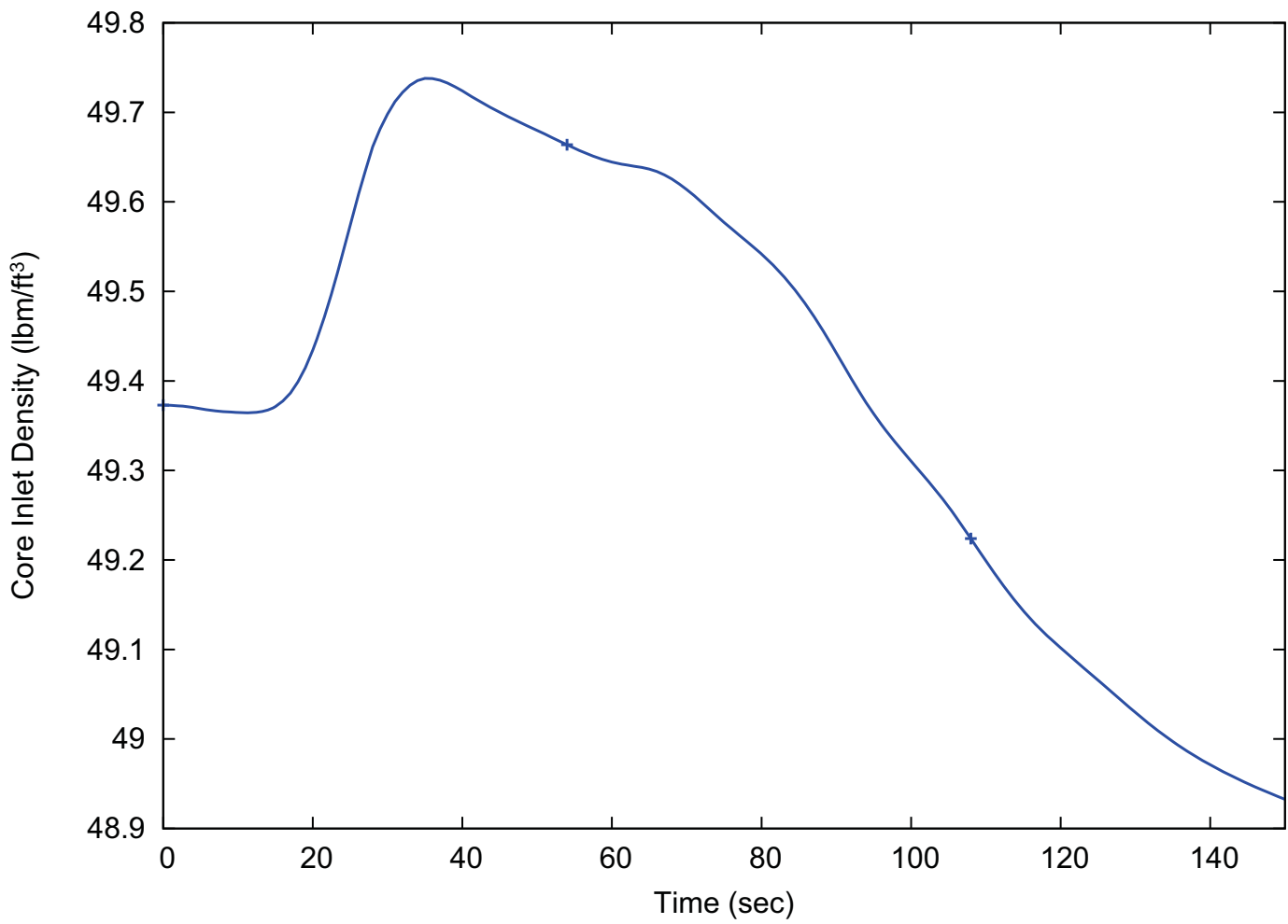
Figure 15.1-13: Core Inlet Density (15.1.2 Increase in Feedwater Flow)
