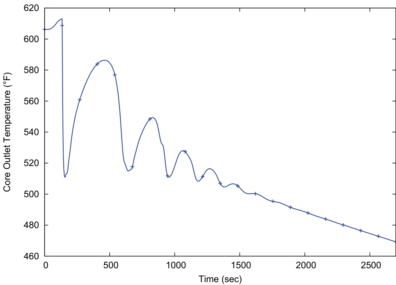
Figure 15.1-54: Core Outlet Temperature (15.1.1 Decrease in Feedwater Temperature)
