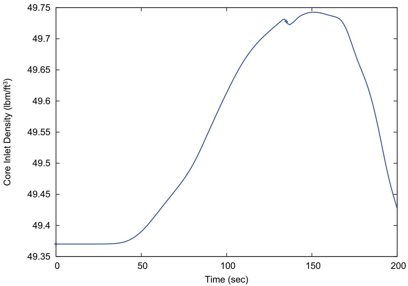
Figure 15.1-3: Core Inlet Density (15.1.1 Decrease in Feedwater Temperature)
