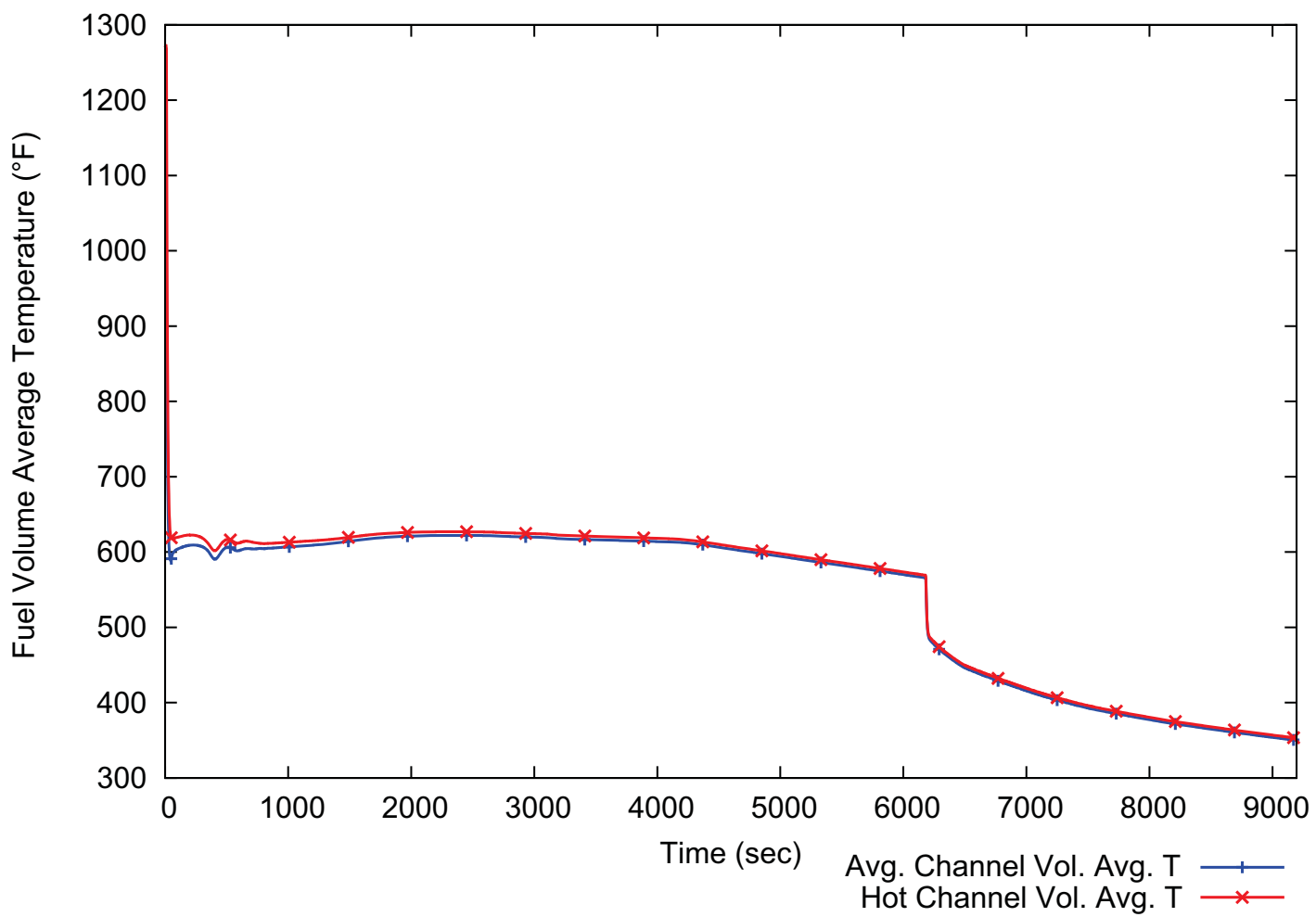
Figure 15.6-54: Loss of Coolant Accident – Fuel Volume Average Temperature
