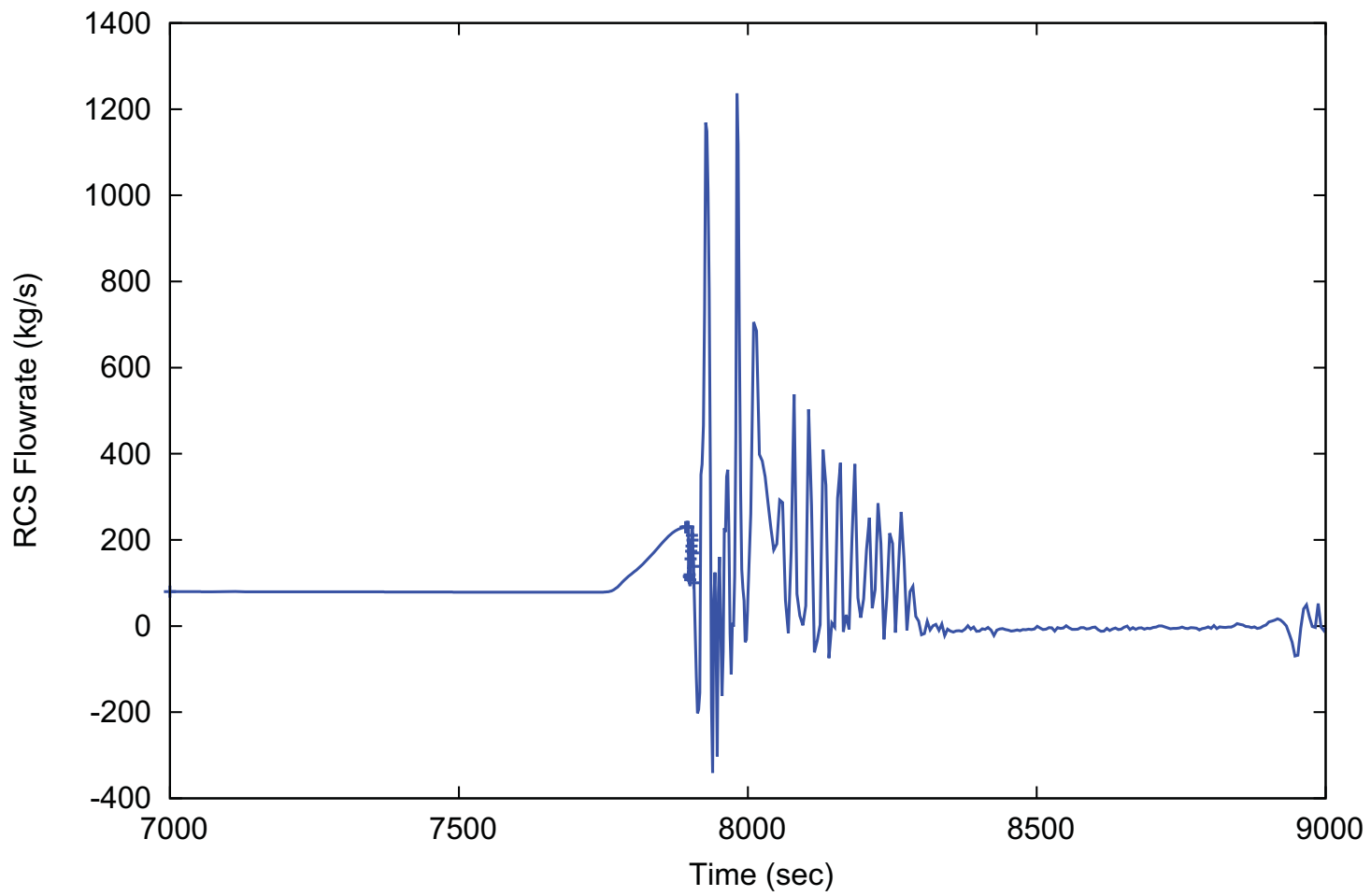
Figure 15.0-16: Return to Power ECCS Transition Case – RCS Flowrate (MCHFR Case)
