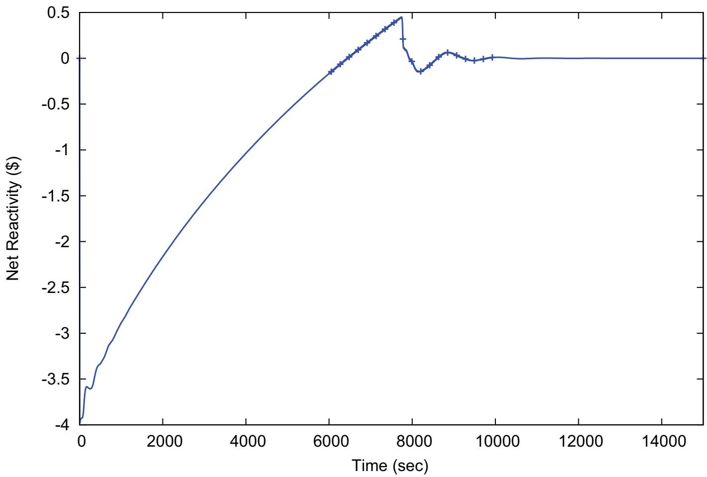
Figure 15.0-10: Return to Power - Net Reactivity (Peak Power Case)
