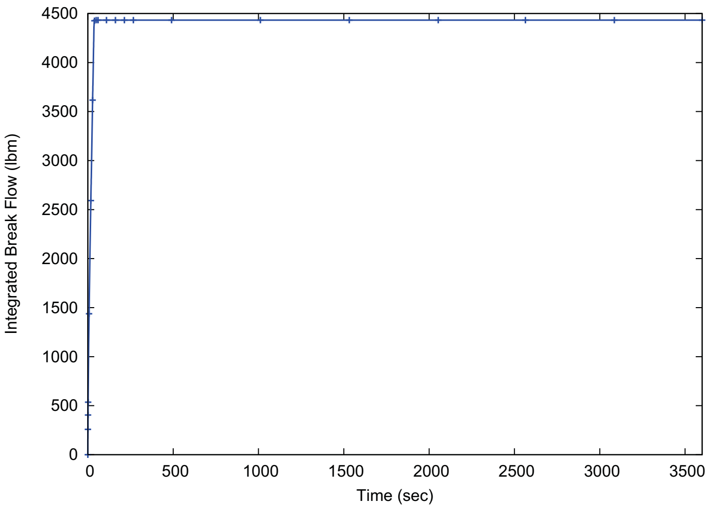
Figure 15.2-41: Integrated Break Flow - Peak RCS Pressure Case (15.2.8 Feedwater Line Break)
