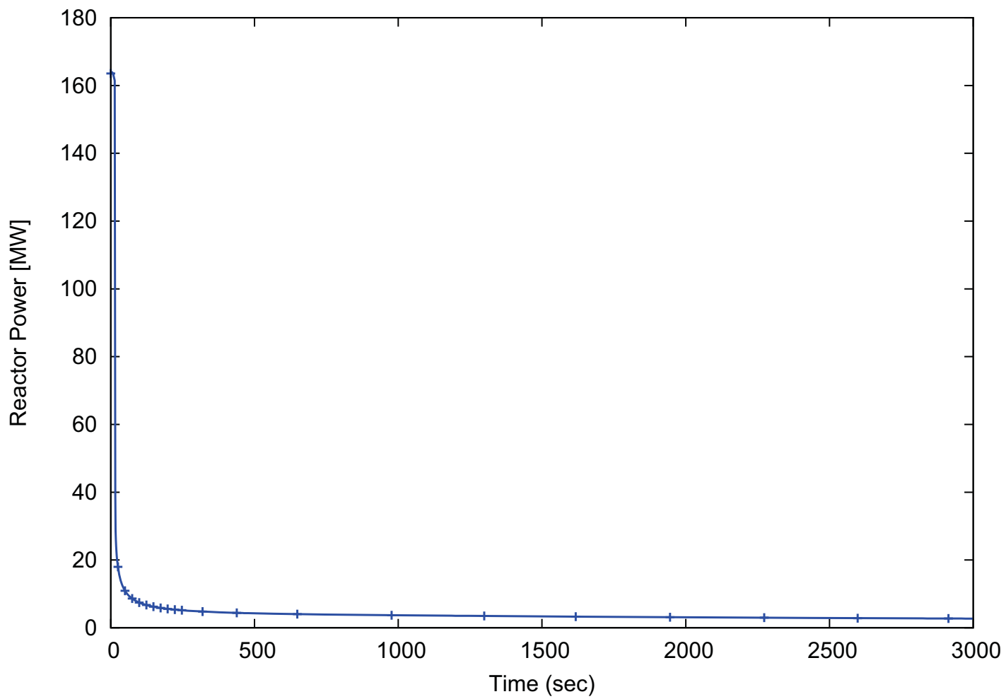
Figure 15.6-5: Failure of Lines Carrying Primary Coolant Outside Containment - Maximum Reactor Pressure Vessel Pressure Scenario - Reactor Power
