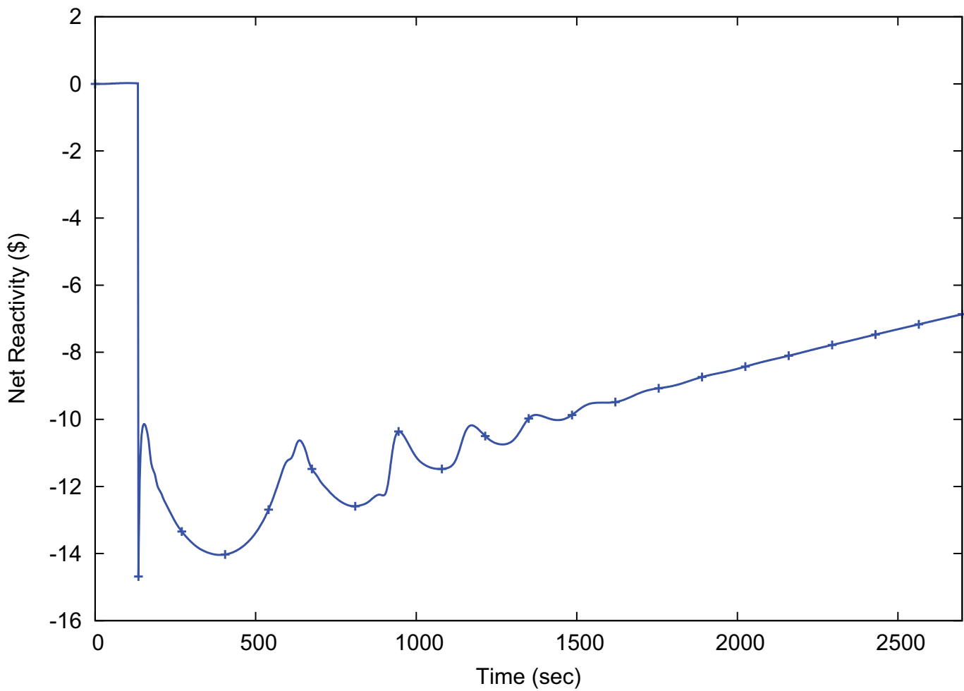
Figure 15.1-55: Core Reactivity – Entire Transient (15.1.1 Decrease in Feedwater Temperature)
