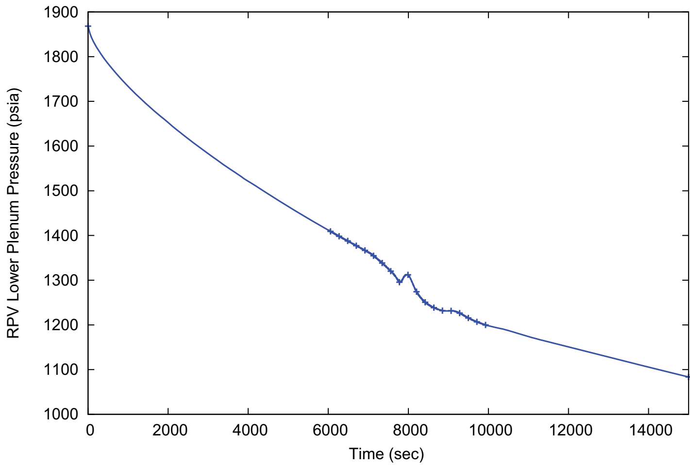
Figure 15.0-13: Return to Power – Reactor Pressure Vessel Lower Plenum Pressure (Peak Power Case)
