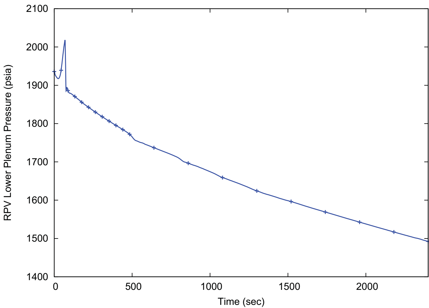
Figure 15.1-60: Reactor Coolant Pressure – Entire Transient (15.1.3 Increase in Steam Flow)
