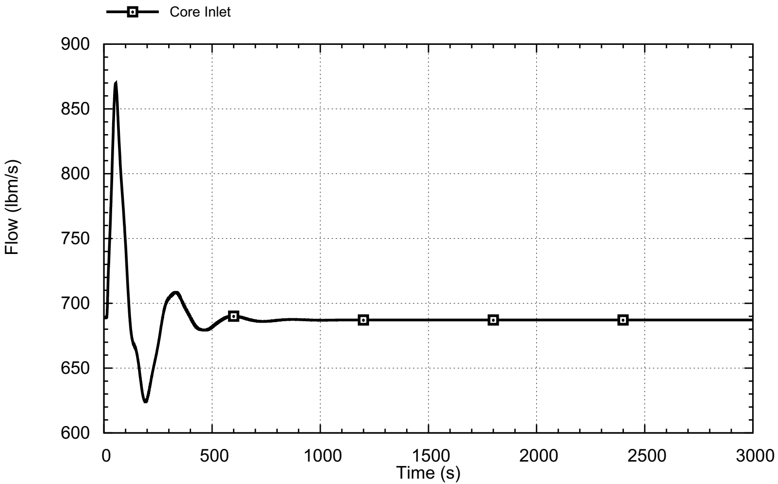
Figure 15.9-12: Time Trace of Primary Coolant Flow Response to Reactivity and Power Distribution Anomalies at 20 Percent of Rated Power and End of Cycle Reactivity
