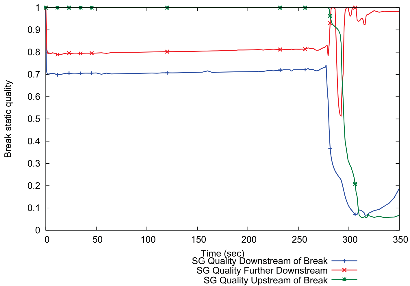
Figure 15.6-21: Steam Generator Tube Failure - Limiting Mass Release Scenario - Break Static Quality
