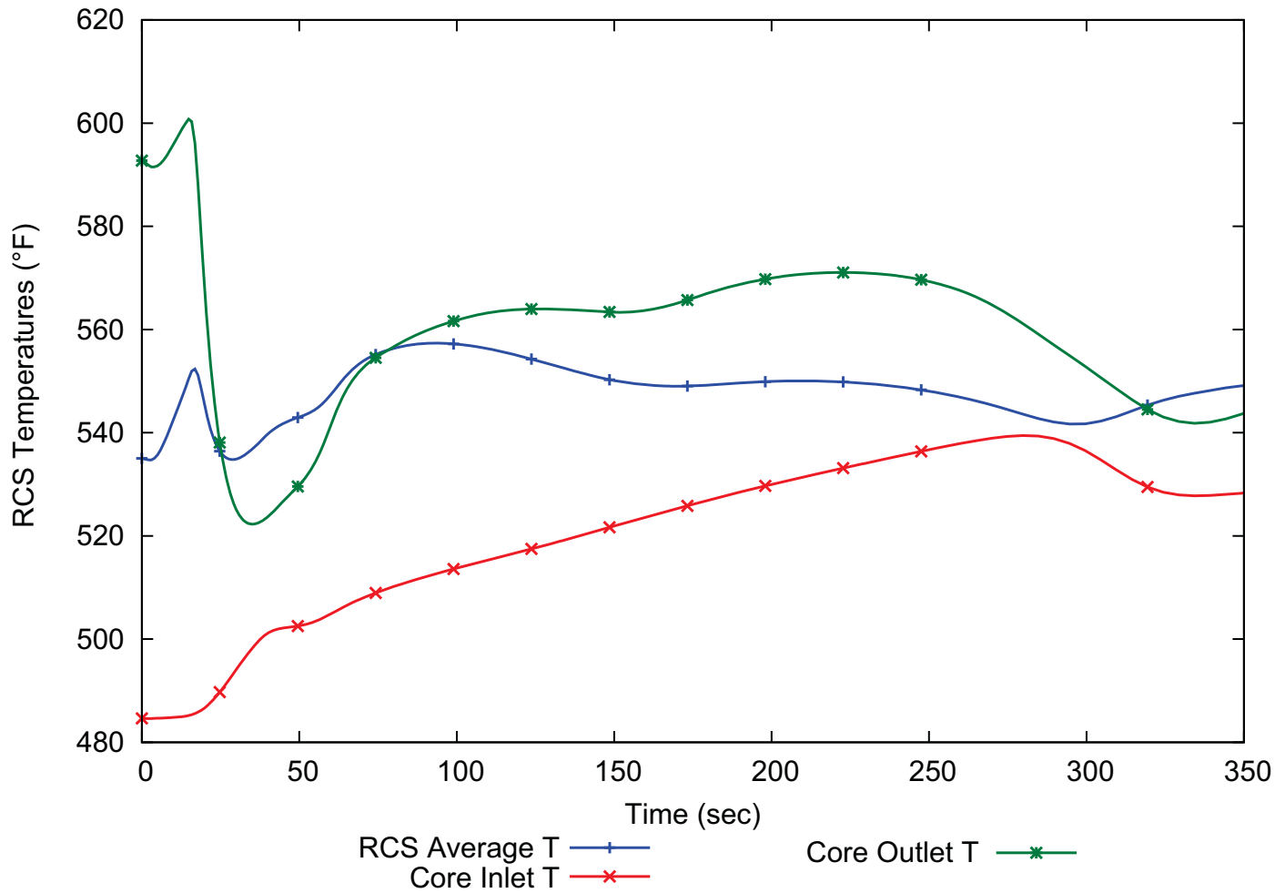
Figure 15.6-7: Failure of Lines Carrying Primary Coolant Outside Containment - Maximum Reactor Pressure Vessel Pressure Scenario - Reactor Coolant System Temperatures
