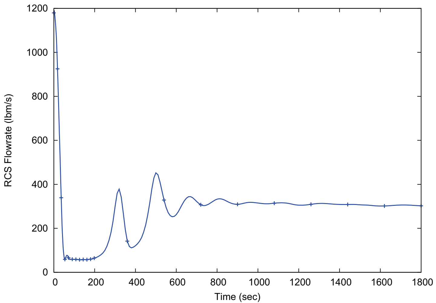
Figure 15.2-23: Reactor Coolant System Flowrate - Peak RCS Pressure Case (15.2.6 Loss of AC Power)
