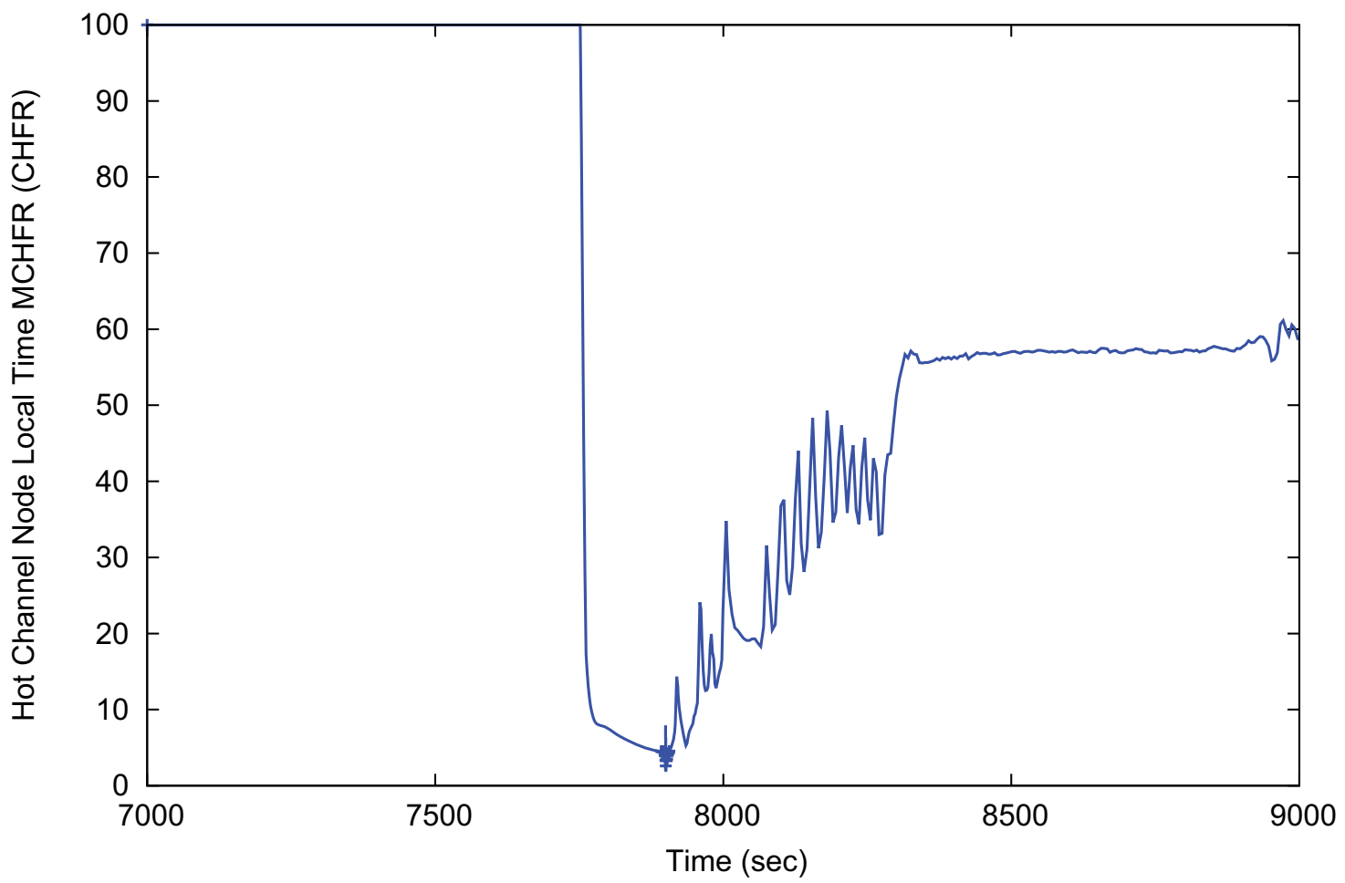
Figure 15.0-14: Return to Power ECCS Transition Case – Critical Heat Flux Ratio (MCHFR Case)
