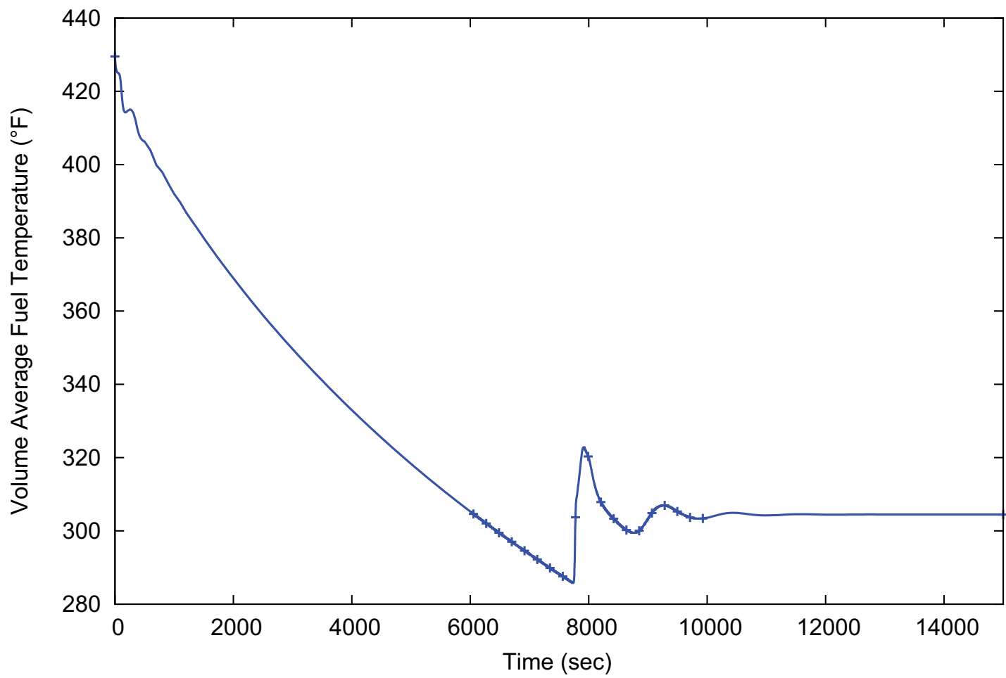
Figure 15.0-12: Return to Power – Volume Average Fuel Temperature (Peak Power Case)
