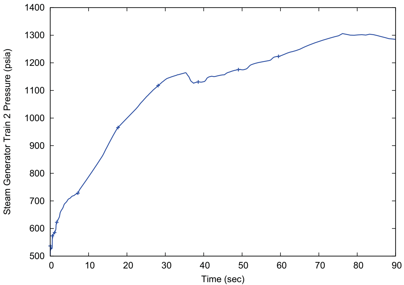
Figure 15.2-38: Steam Generator Train 2 Pressure - Peak RCS Pressure Case (15.2.8 Feedwater Line Break)
