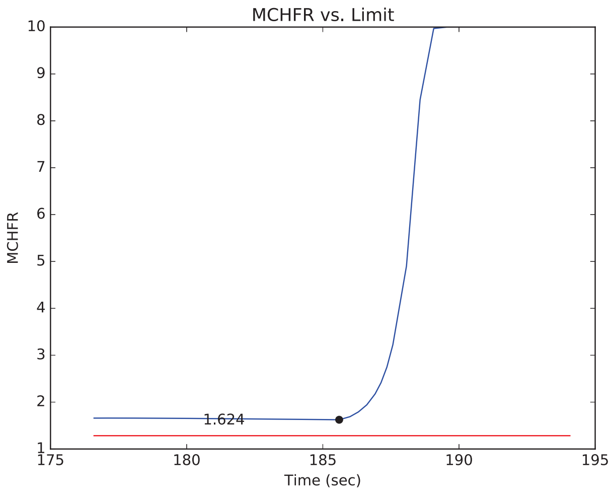
Figure 15.4-11: Critical Heat Flux Ratio (15.4.2 Uncontrolled Control Rod Assembly Withdrawal at Power)
