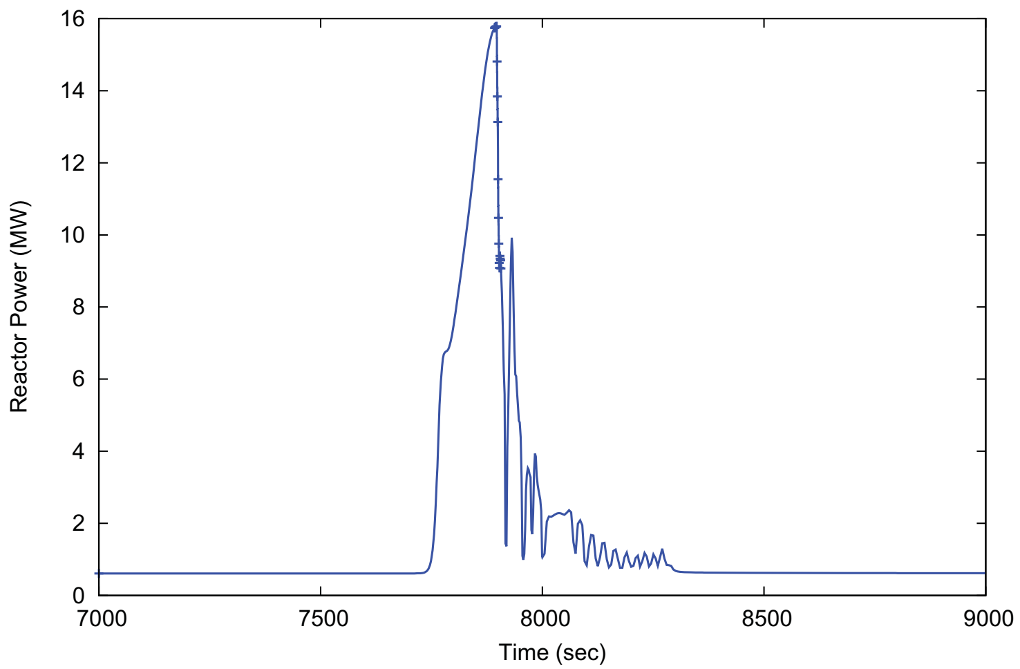
Figure 15.0-15: Return to Power ECCS Transition Case – Reactor Power (MCHFRC Case)
