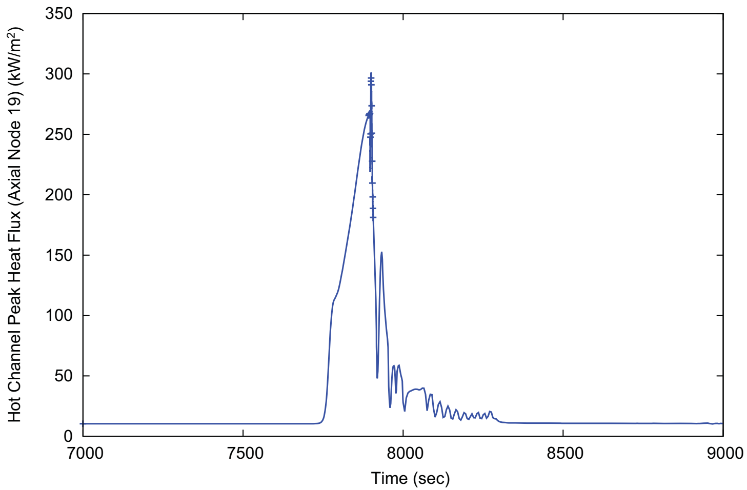
Figure 15.0-17: Return to Power ECCS Transition Case – Hot Channel Heat Flux (MCHFR Case)
