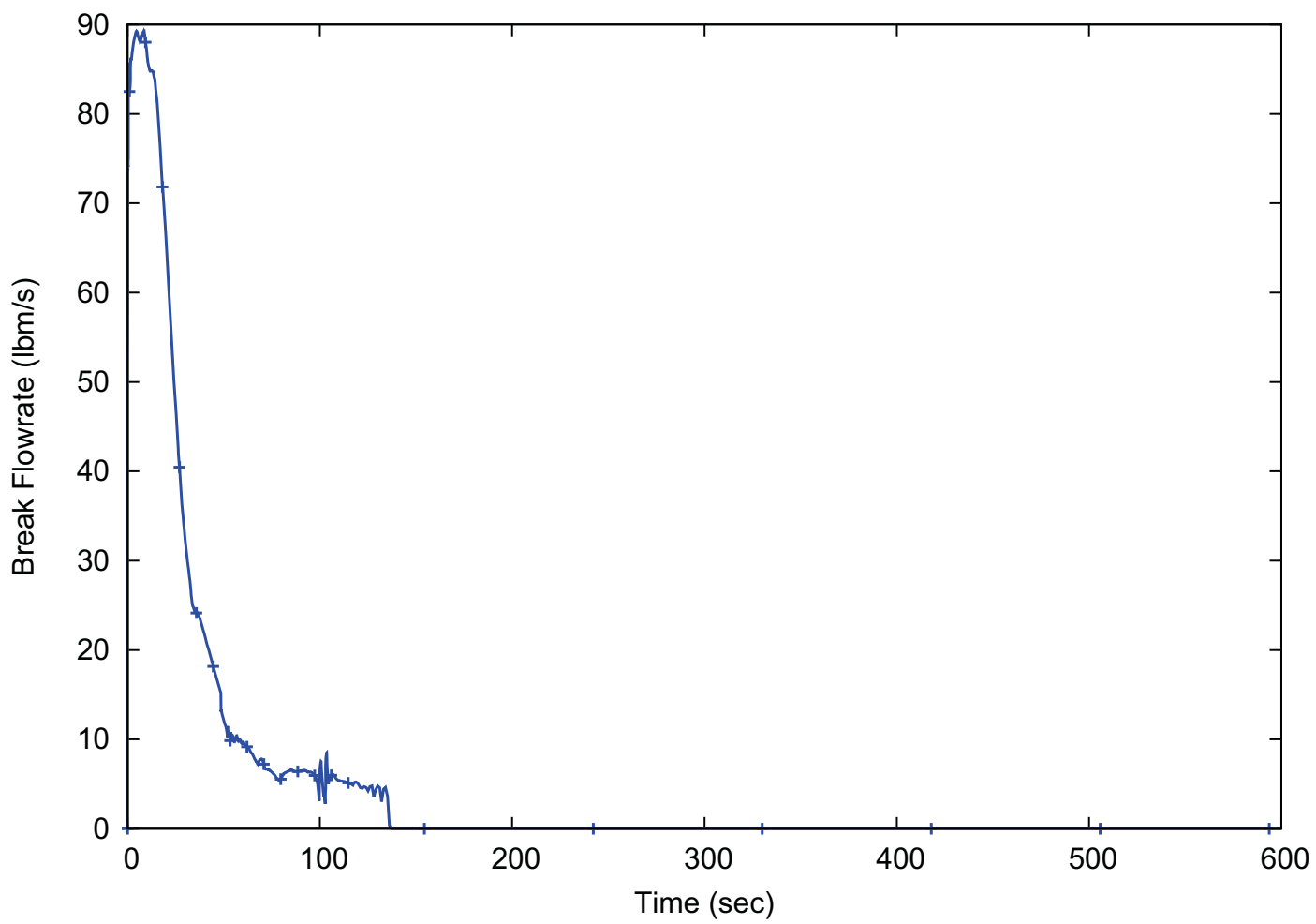
Figure 15.1-32: Break Flow Rate (15.1.5 Steam Piping Failure, Limiting Reactor Coolant System Pressure)
