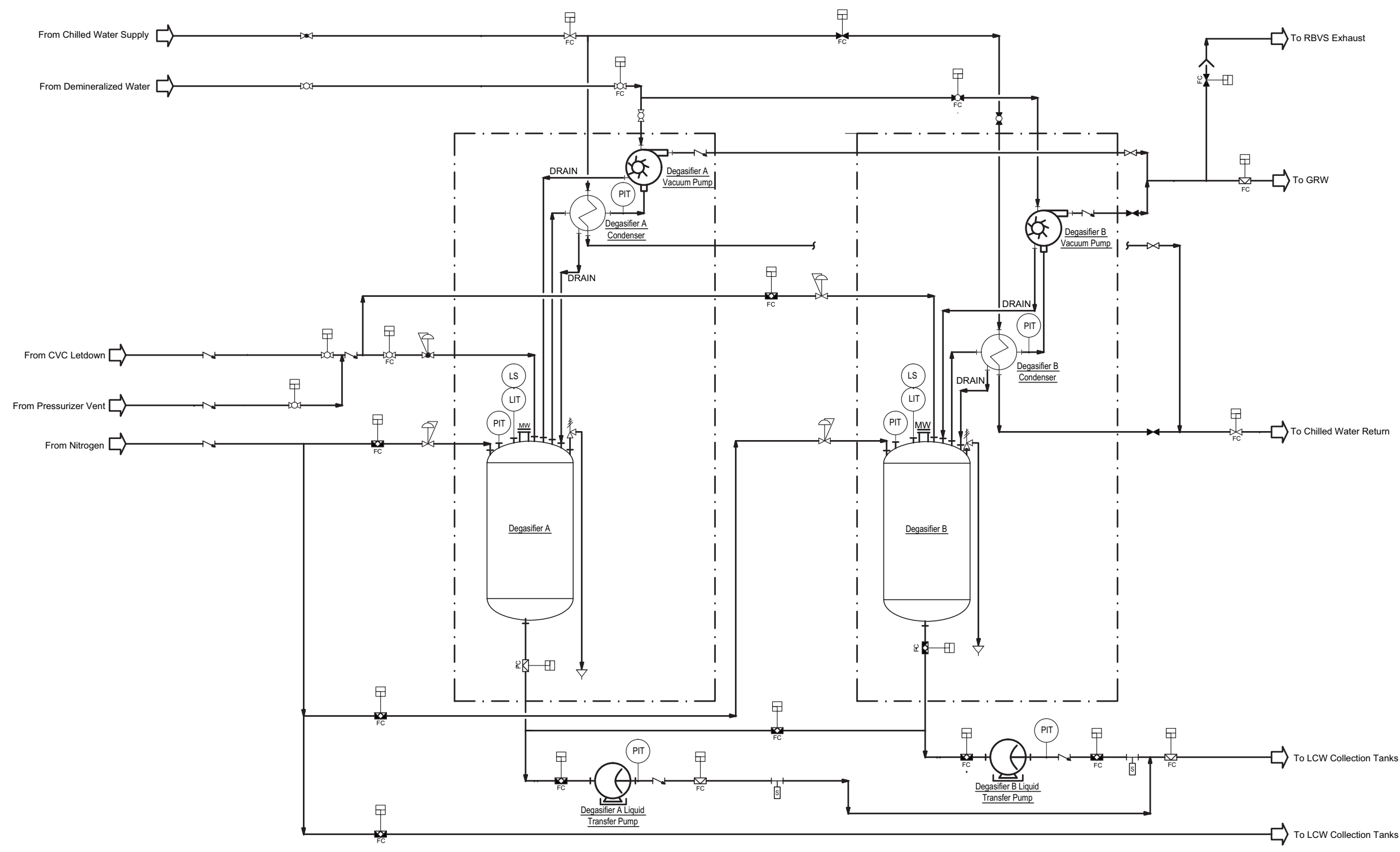
Figure 11.2-1a: Liquid Radioactive Waste System Diagram
