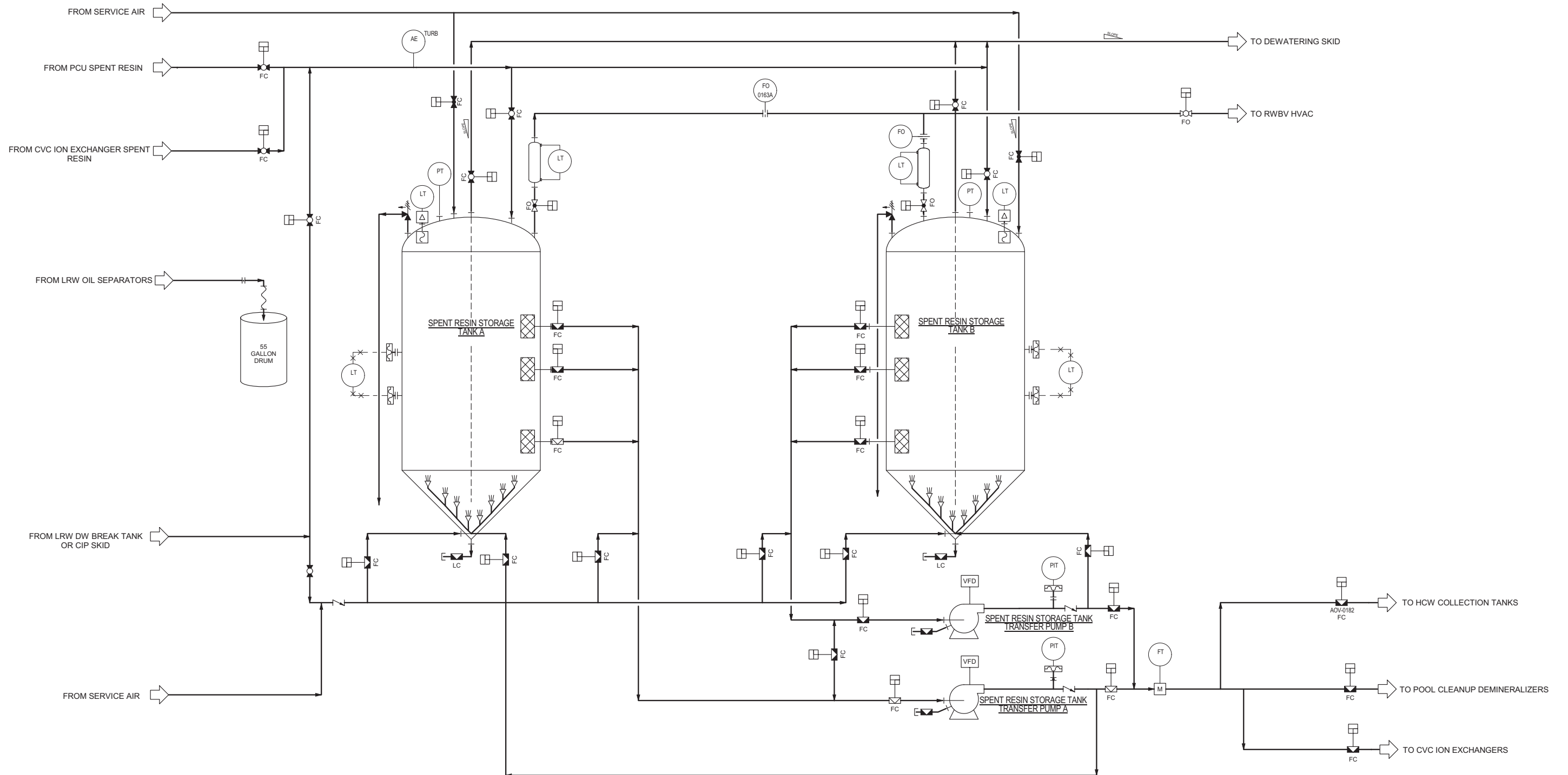
Figure 11.4-2b: Solid Radioactive Waste System Diagram
