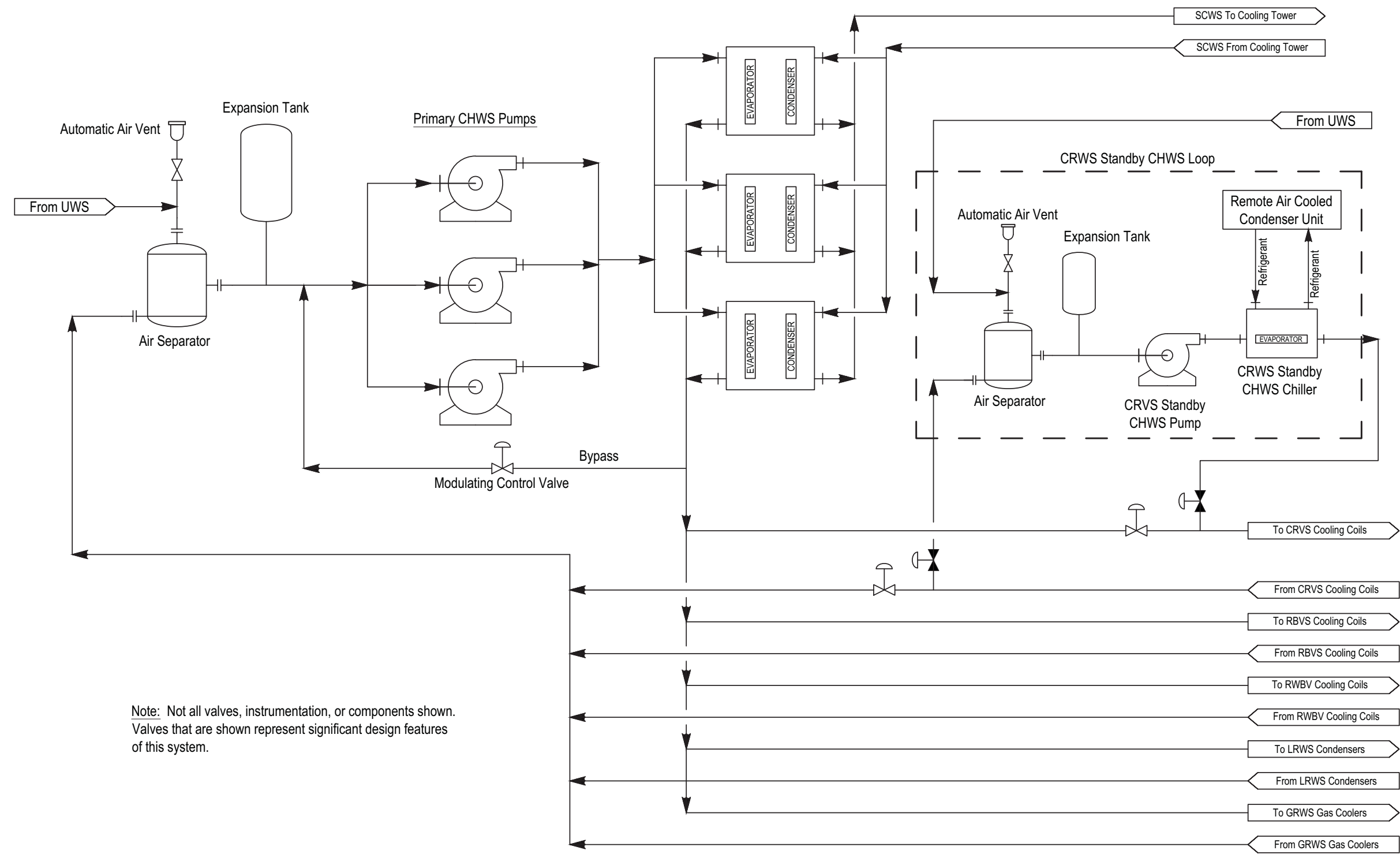
Figure 9.2.8-1: Chilled Water System Diagram
