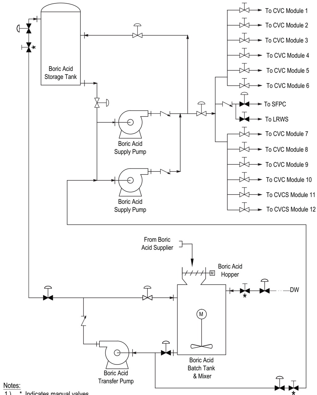
Figure 9.3.4-2: Boron Addition System Diagram
