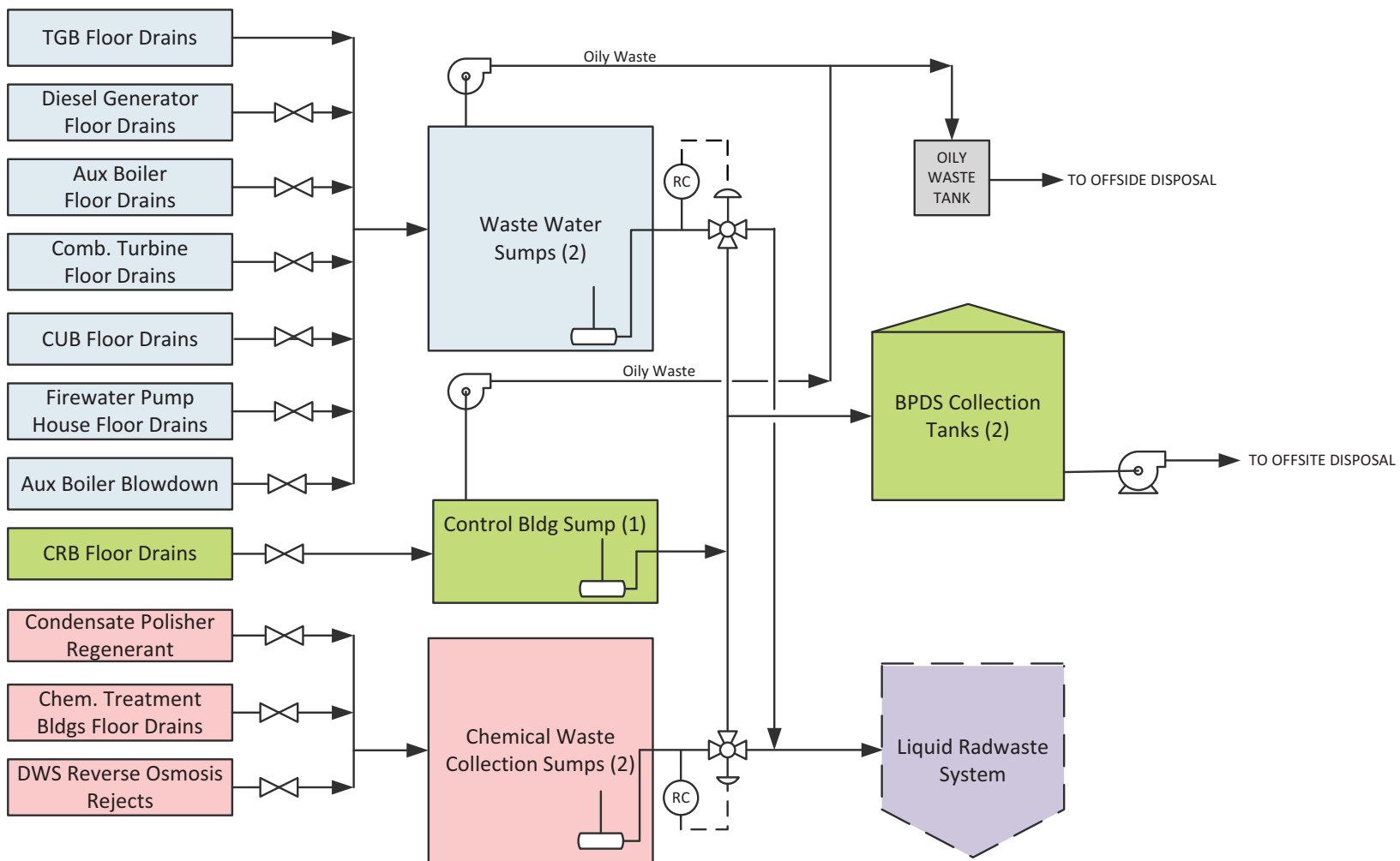
Figure 9.3.3-2: Balance-of-Plant Drain System Diagram
