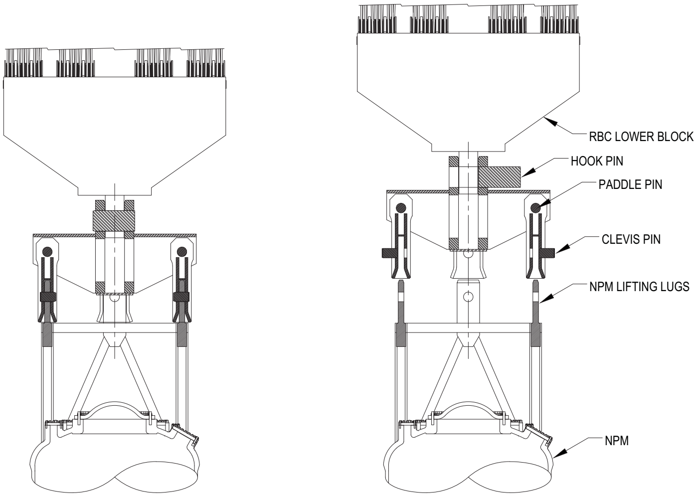
Figure 9.1.5-4: Module Lifting Adapter
