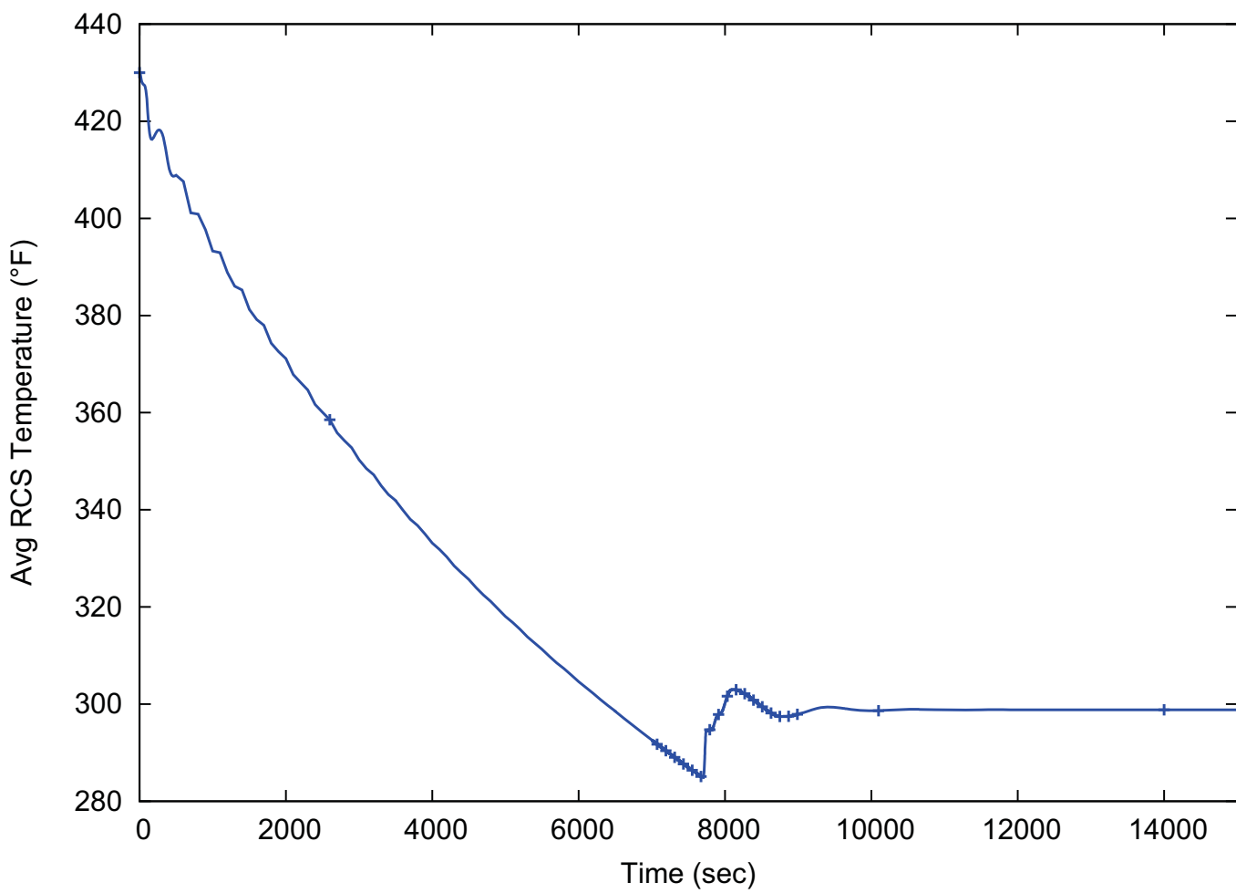
Figure 15.0-11: Return to Power – Average Reactor Coolant System Temperature (Peak Power Case)
