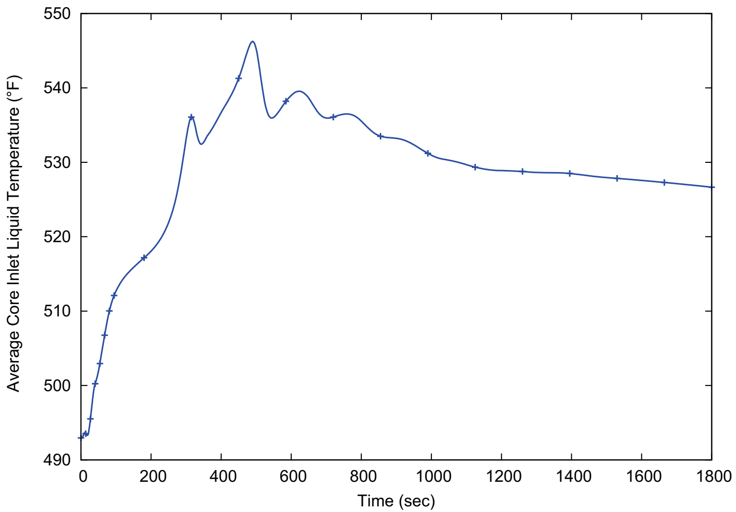
Figure 15.2-50: Average Core Inlet Temperature - Peak RCS Pressure Case (15.2.9 Inadvertent Operation of DHR5)
