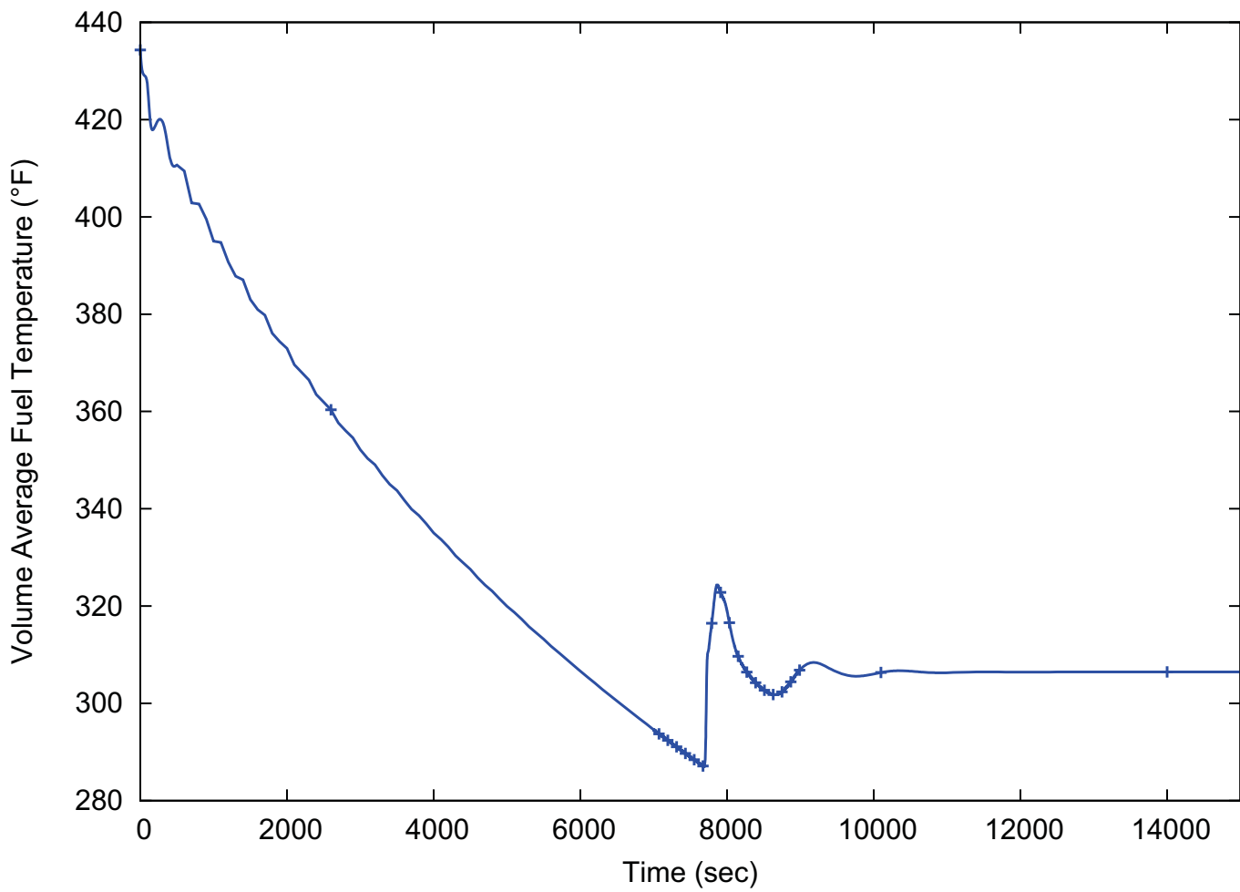
Figure 15.0-12: Return to Power – Volume Average Fuel Temperature (Peak Power Case)
