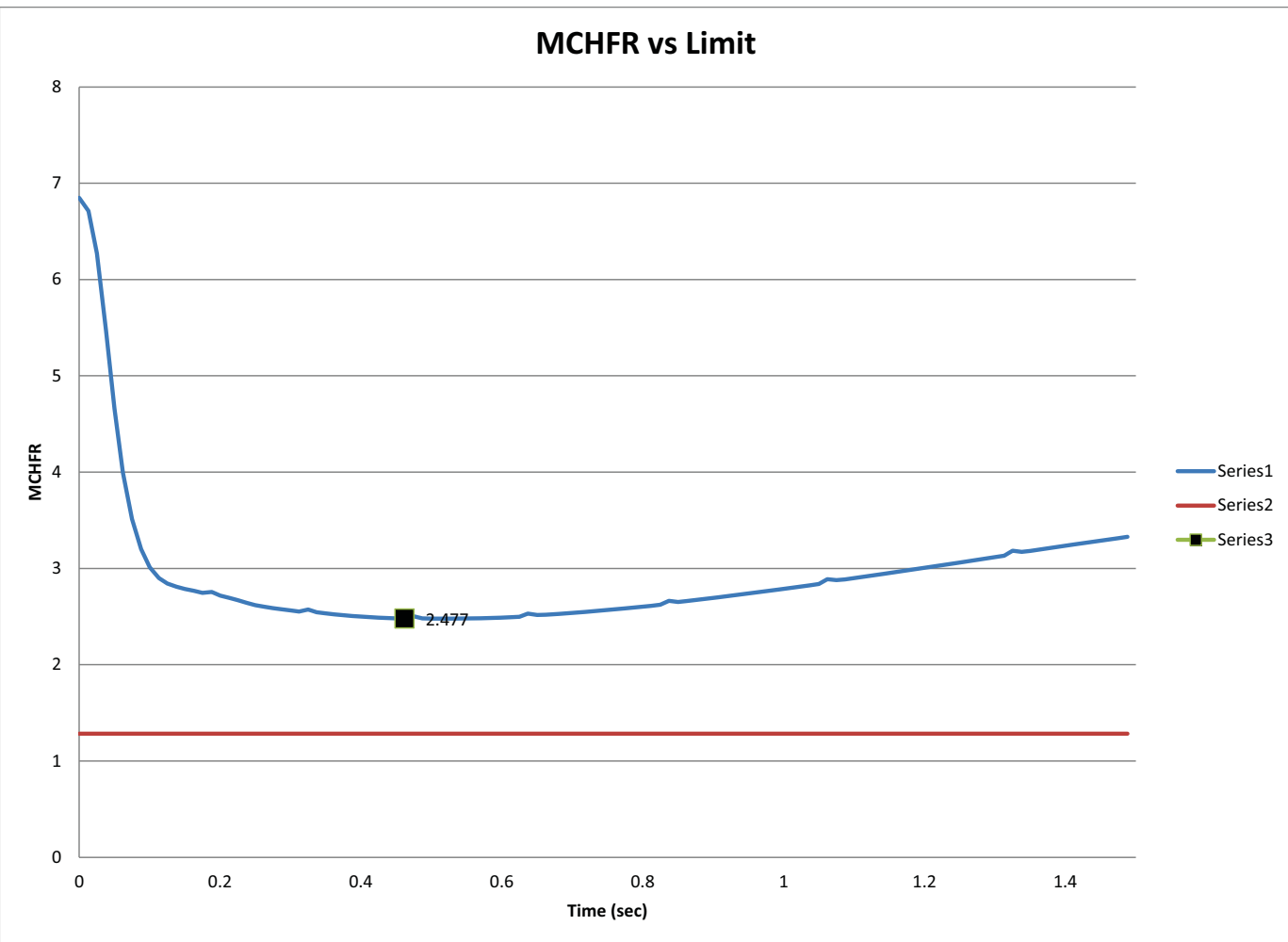
Figure 15.4-37: Critical Heat Flux Ratio (15.4.8 Rod Ejection Accident)
