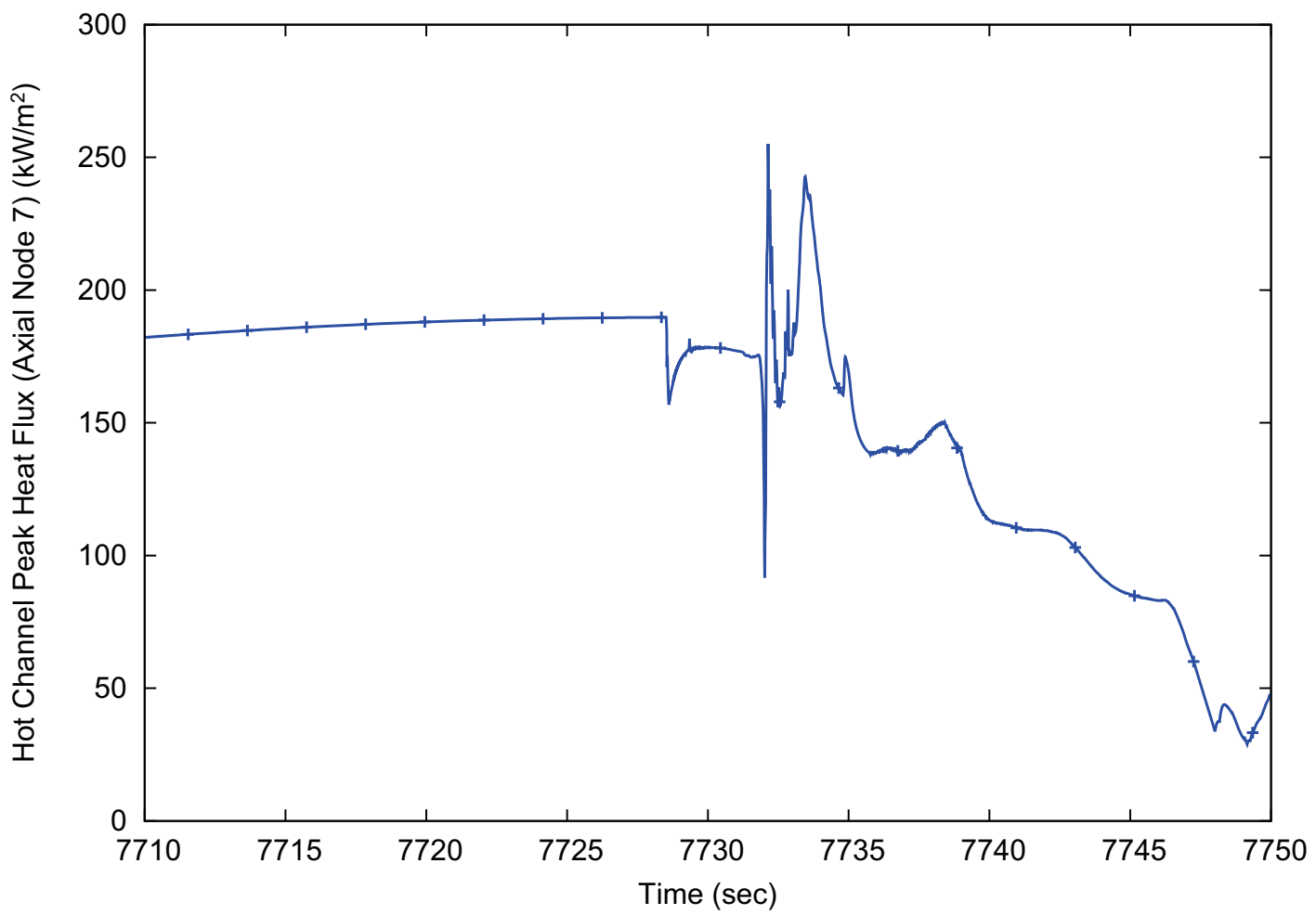
Figure 15.0-17: Return to Power ECCS Transition Case – Hot Channel Heat Flux (MCHFR Case)
