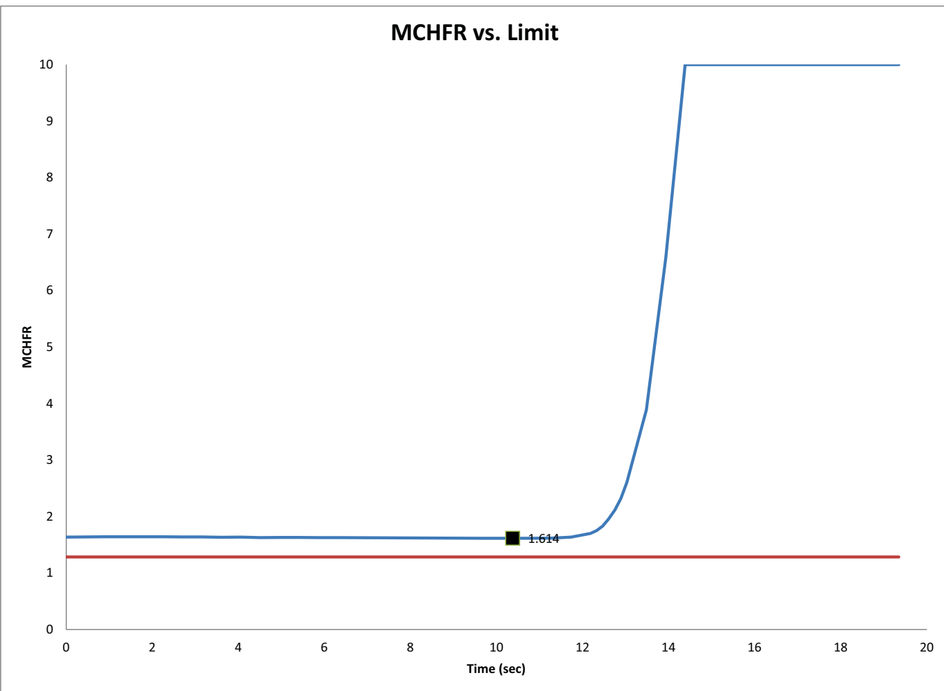
Figure 15.4-35: Critical Heat Flux Ratio (15.4.3 Control Rod Misoperation, Single Control Rod Assembly Withdrawal)
