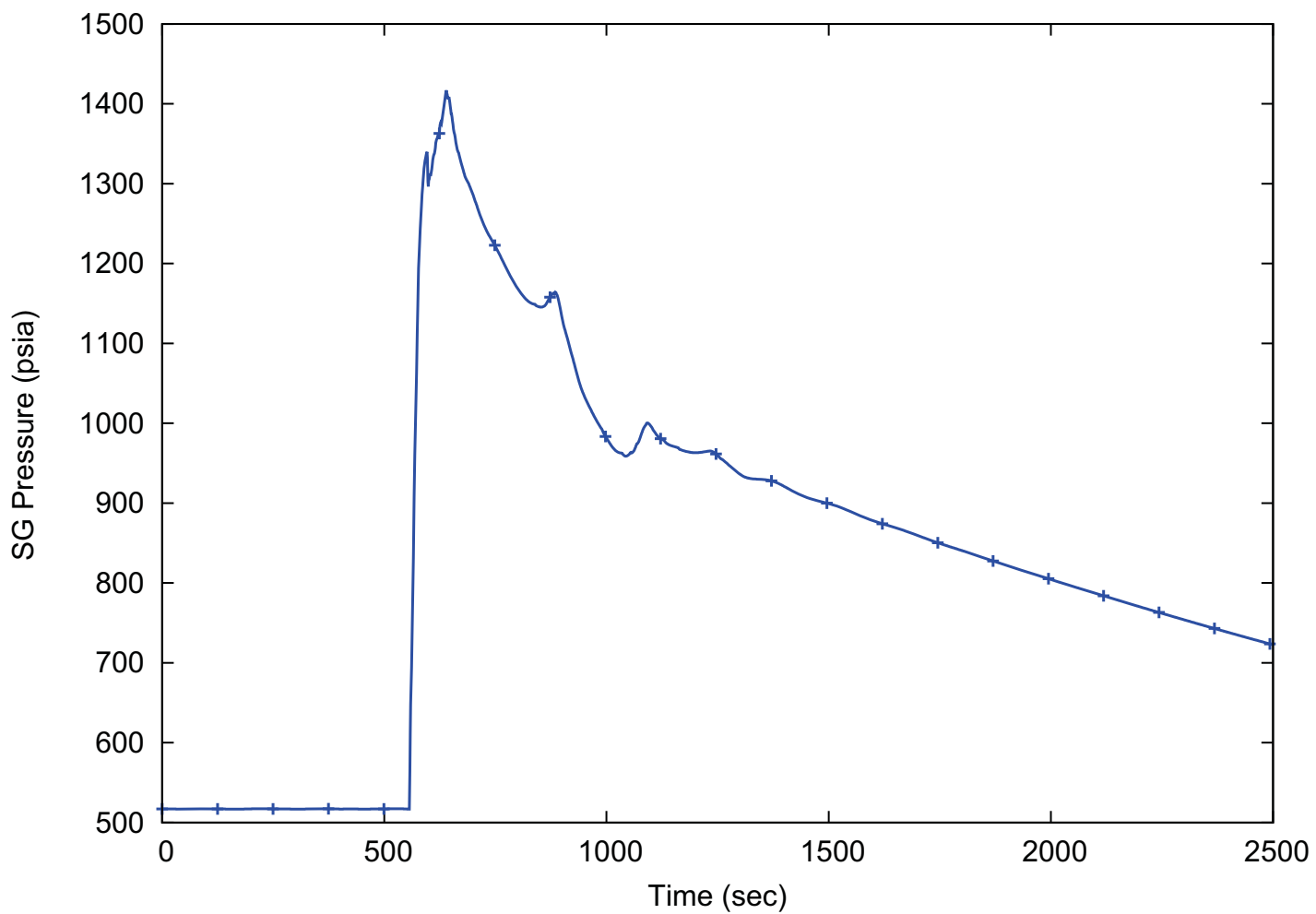
Figure 15.5-9: Steam Generator Pressure (Typical) - Increase in RCS Inventory (PZR Spray Available)
