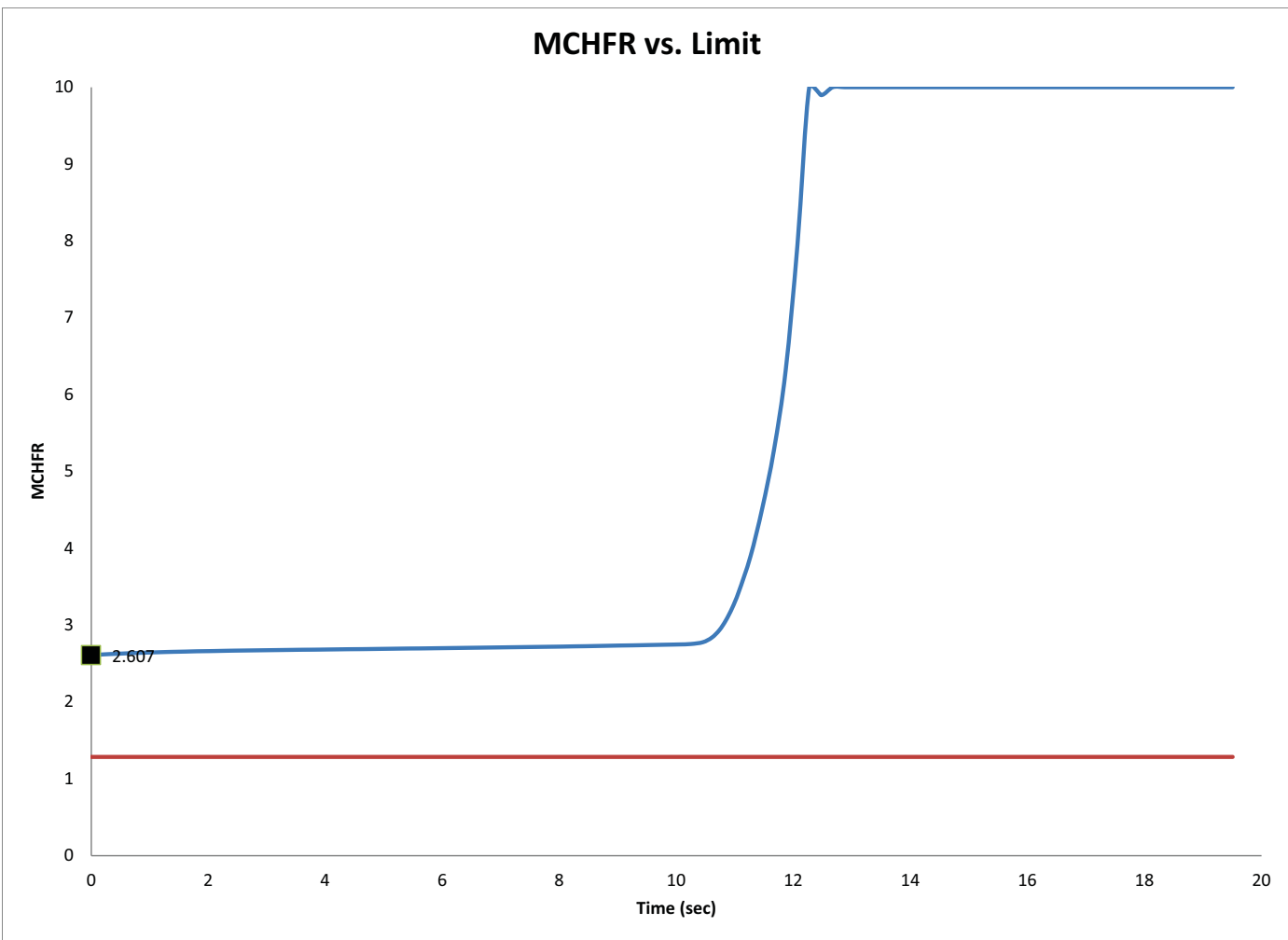
Figure 15.2-44: Hot Channel Node MCHFR - Limiting MCHFR Case (15.2.8 Feedwater Line Break)
