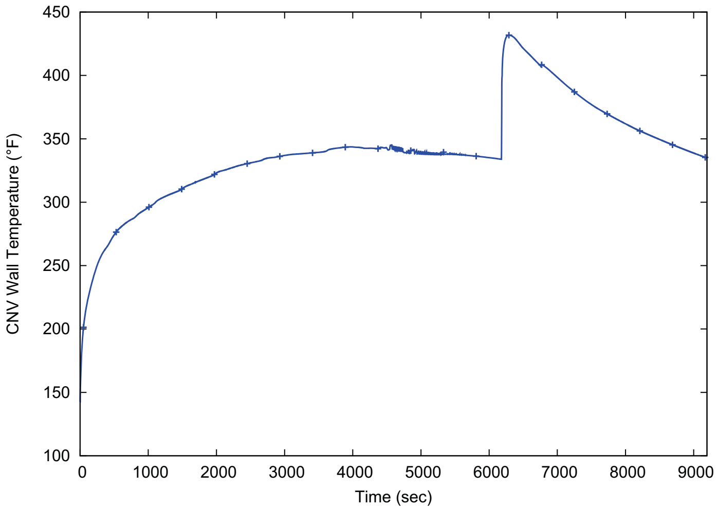
Figure 15.6-52: Loss of Coolant Accident - Containment Wall Temperature
