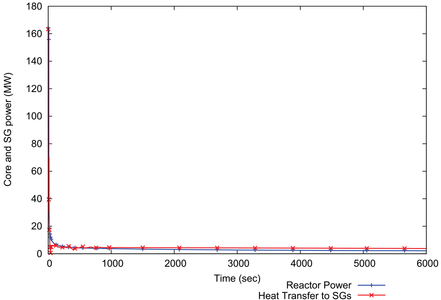
Figure 15.6-25: Steam Generator Tube Failure – Limiting Reactor Pressure Vessel Pressure Scenario – Core and Steam Generator Power
