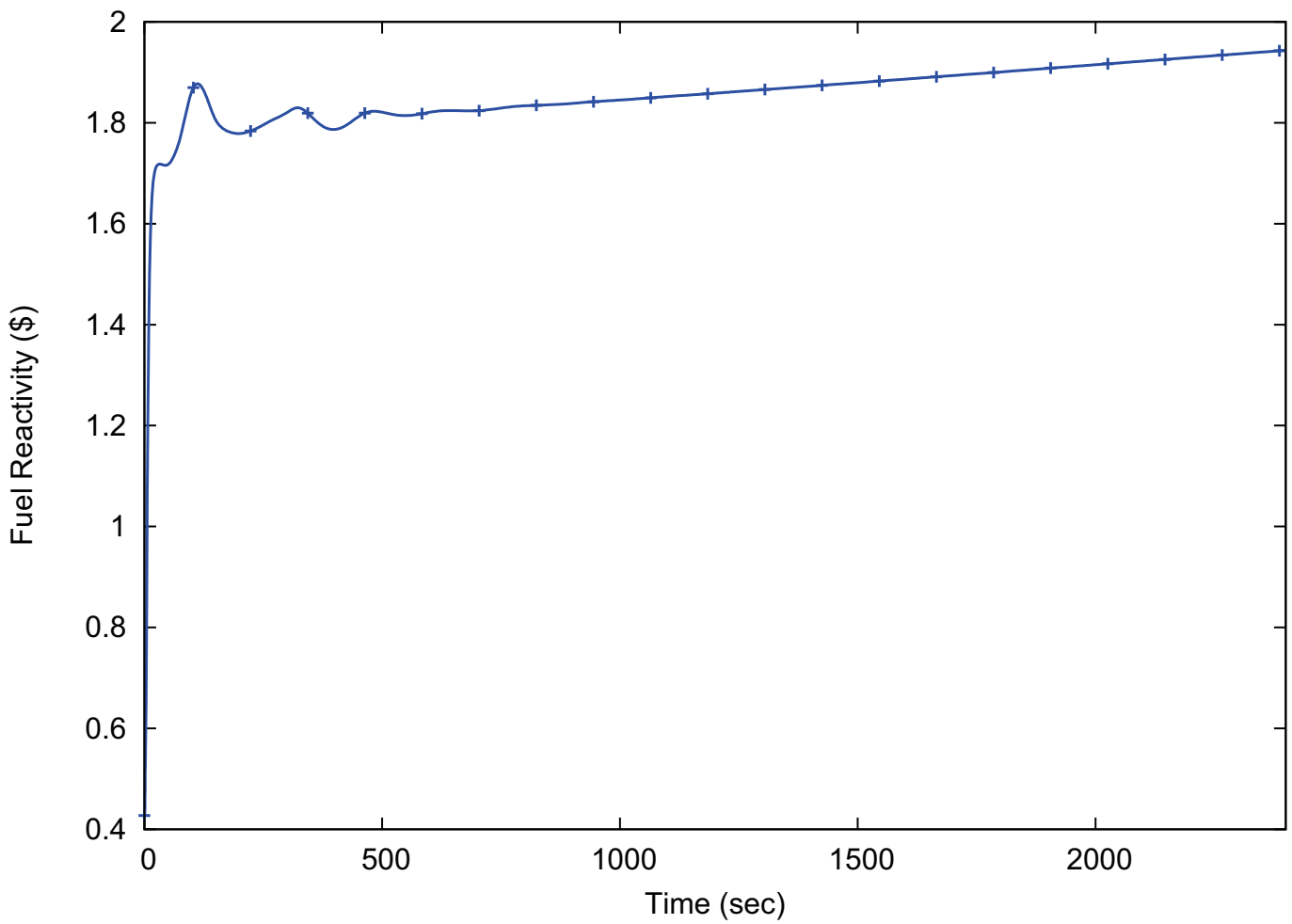
Figure 15.4-27: Fuel Reactivity (15.4.3 Control Rod Misoperation, Control Rod Assembly drop)
