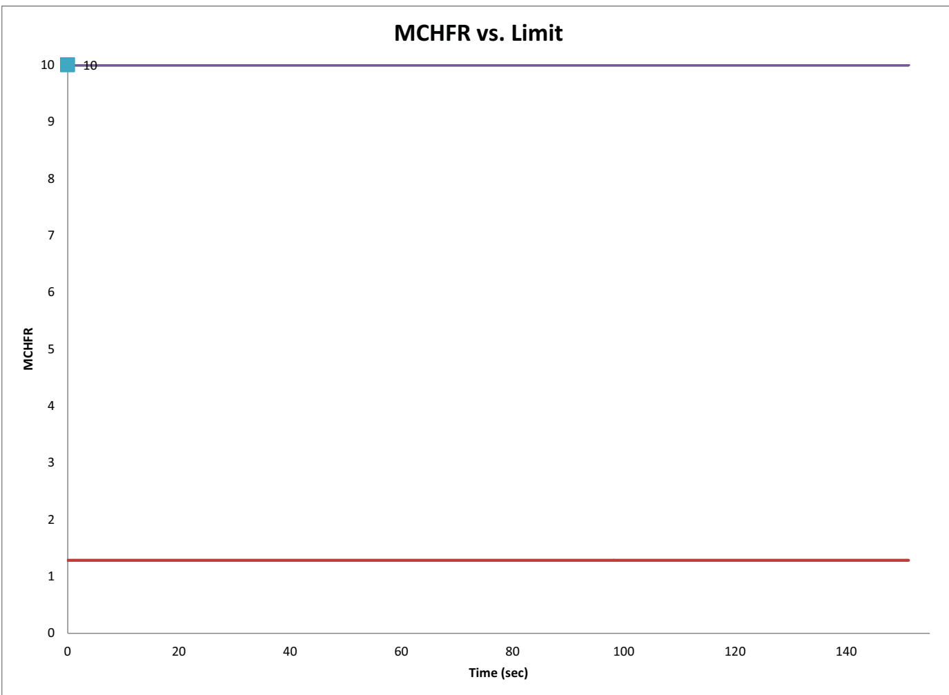
Figure 15.4-5: Critical Heat Flux Ratio (15.4.1 Uncontrolled Control Rod Assembly Withdrawal from a Subcritical or Low Power Condition)
