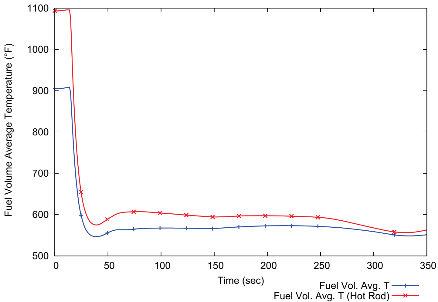
Figure 15.6-12: Failure of Lines Carrying Primary Coolant Outside Containment - Maximum Reactor Pressure Vessel Pressure Scenario - Fuel Volume Average Temperature
