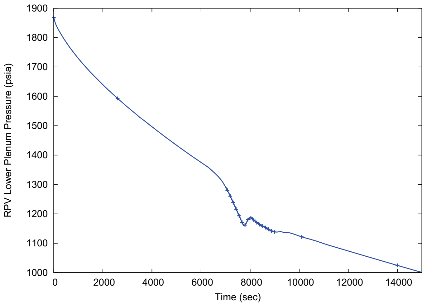
Figure 15.0-13: Return to Power – Reactor Pressure Vessel Lower Plenum Pressure (Peak Power Case)
