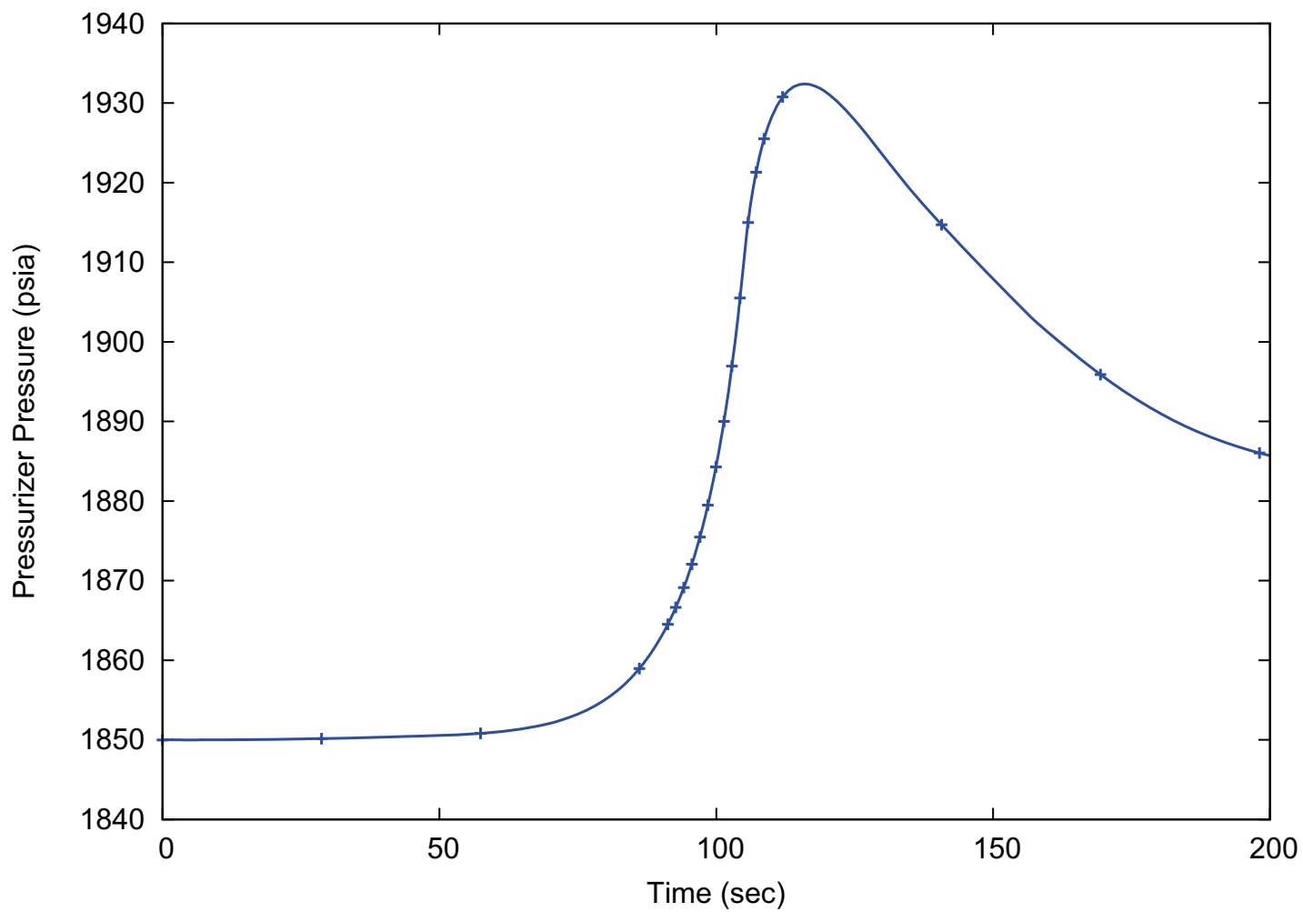
Figure 15.4-4: Pressurizer Pressure (15.4.1 Uncontrolled Control Rod Assembly Withdrawal from a Subcritical or Low Power Condition)
