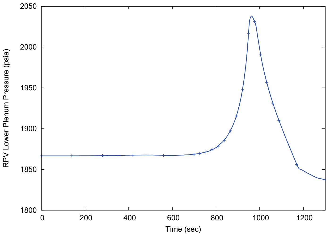
Figure 15.4-34: Reactor Coolant System Pressure for Maximum Pressure Case (15.4.1 Uncontrolled Control Rod Assembly Withdrawal from a Subcritical or Low Power Condition)
