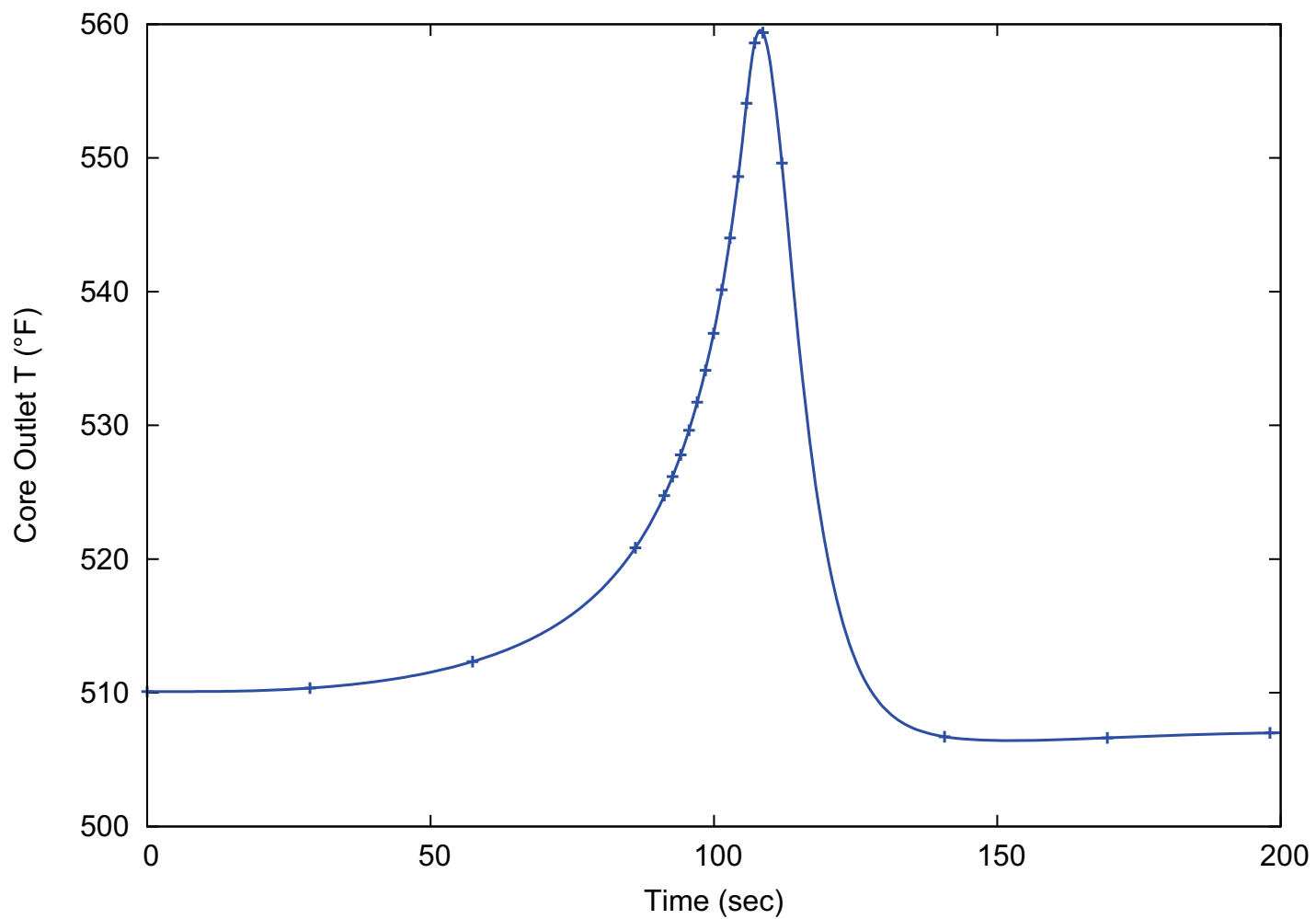
Figure 15.4-3: Core Outlet Temperature (15.4.1 Uncontrolled Control Rod Assembly Withdrawal from a Subcritical or Low Power Condition)
