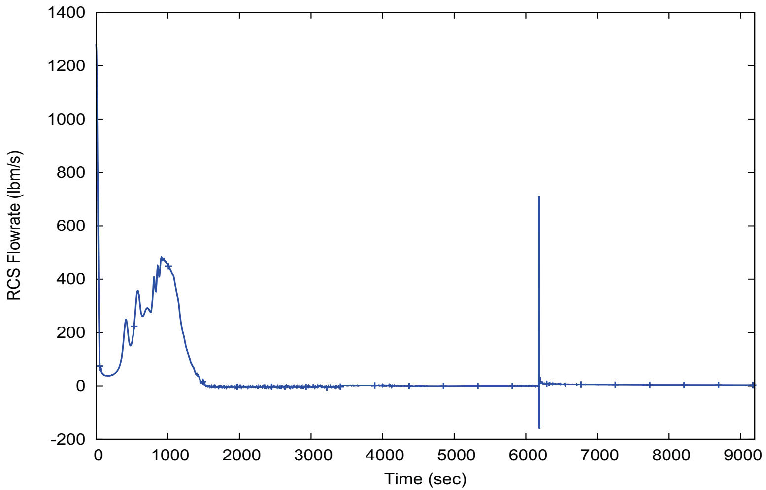
Figure 15.6-50: Loss of Coolant Accident - Reactor Coolant System Flowrate
