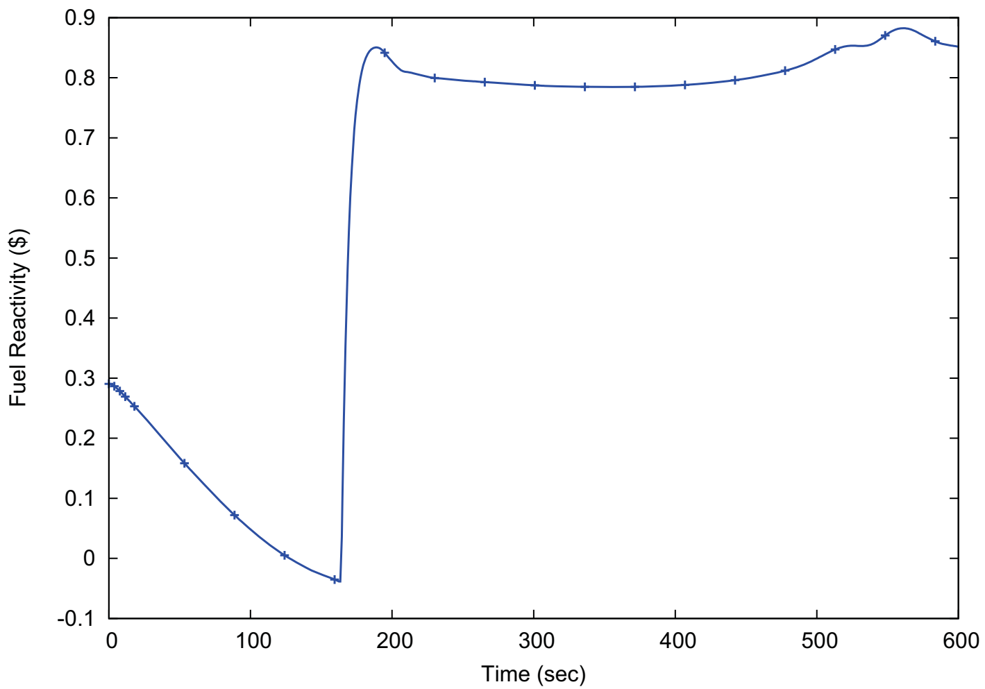
Figure 15.4-19: Fuel Reactivity (15.4.3 Control Rod Misoperation, Single Control Rod Assembly Withdrawal)
