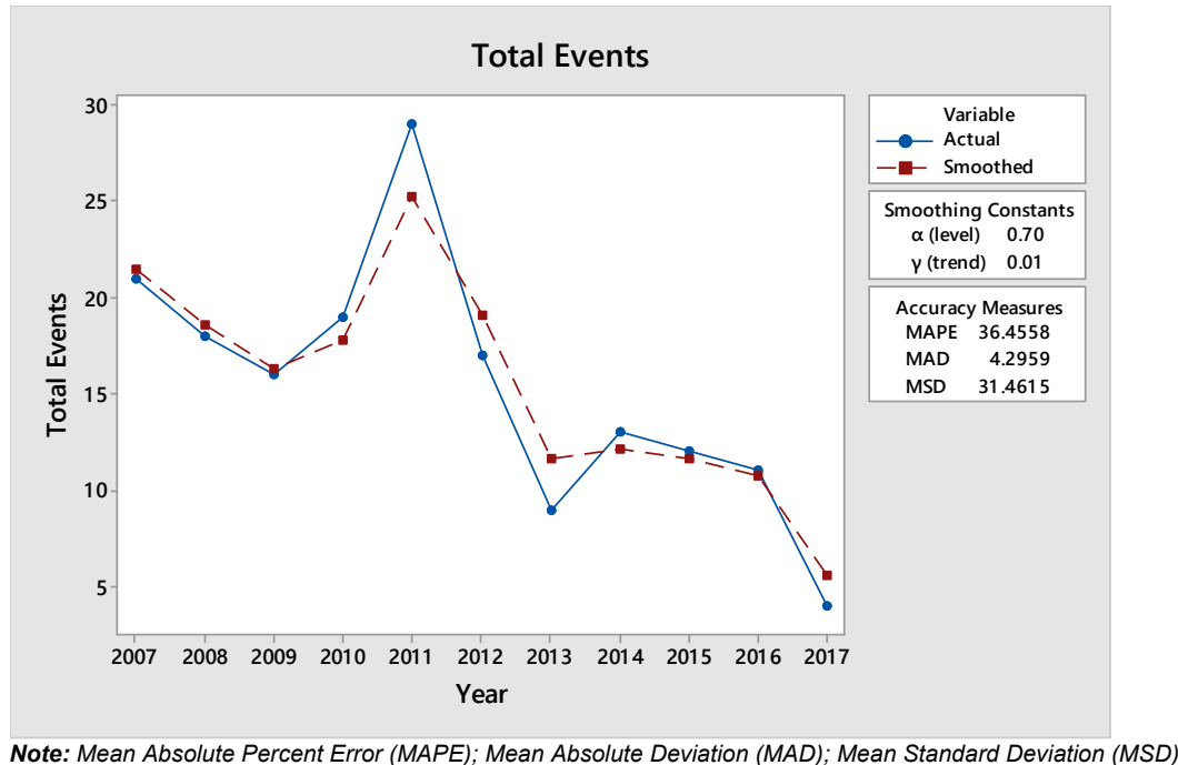
Figure 2. Time Series Model
