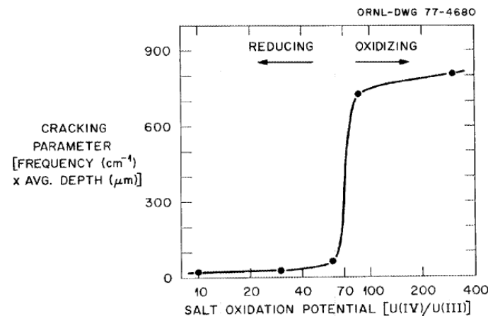
Fig. 12. Cracking Behavior of Hastelloy N Exposed 260 hr at 700°C to MSBR Fuel Salt Containing \text{CrTe}_{1.266} .
