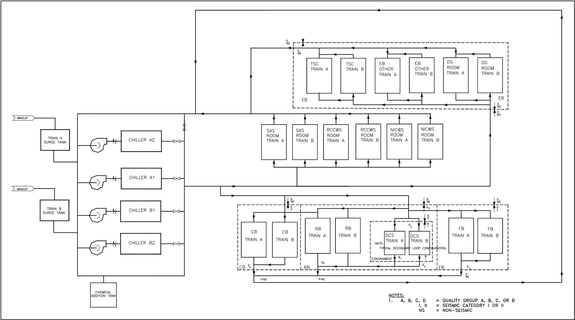
Figure 2.12.5-1. NICWS Functional Arrangement
