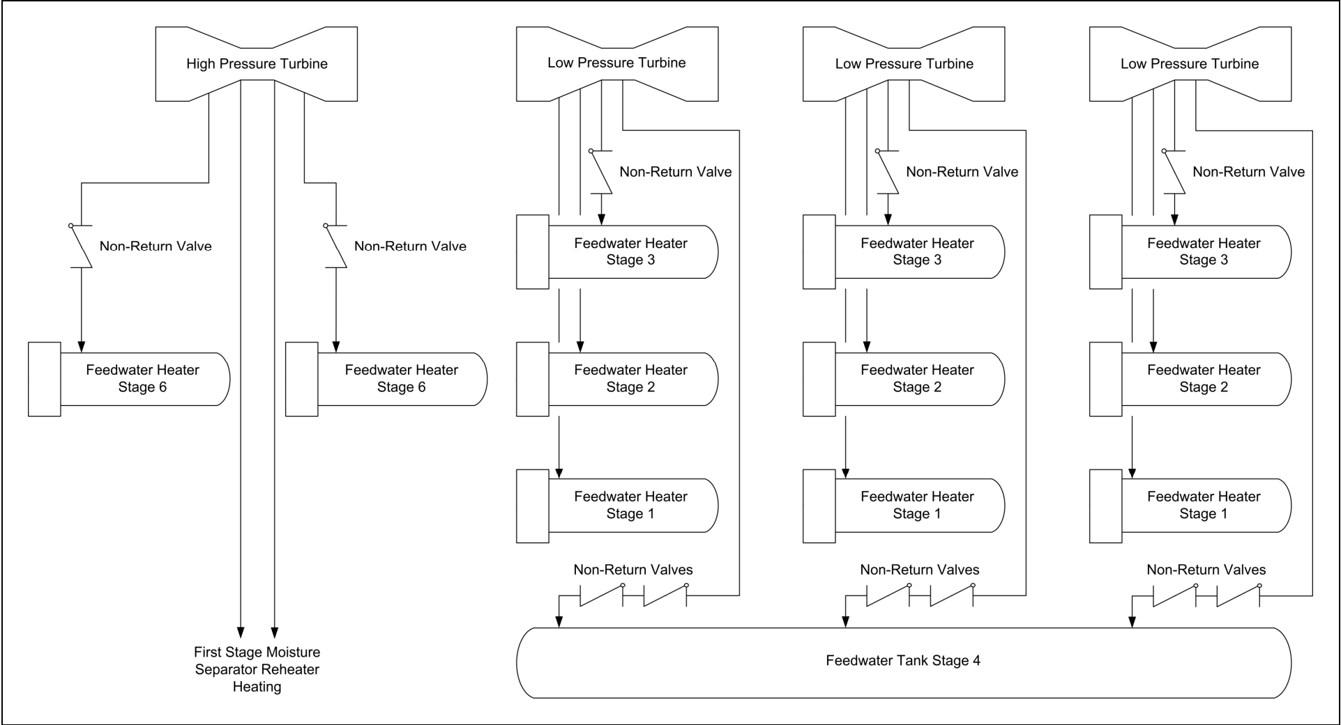
Figure 2.11.1-3. Extraction Steam Functional Arrangement
