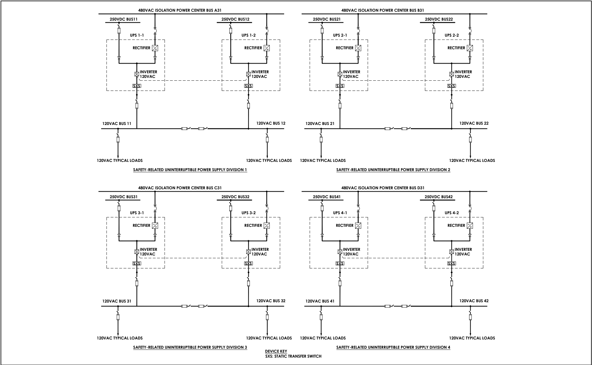
Figure 2.13.5-1. Safety-Related UPS System Functional Arrangement
