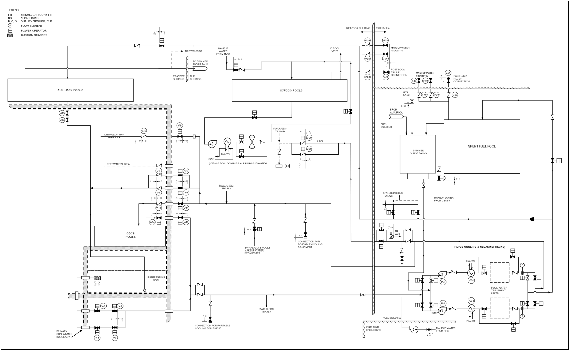
Figure 2.6.2-1. Fuel and Auxiliary Pools Cooling System
