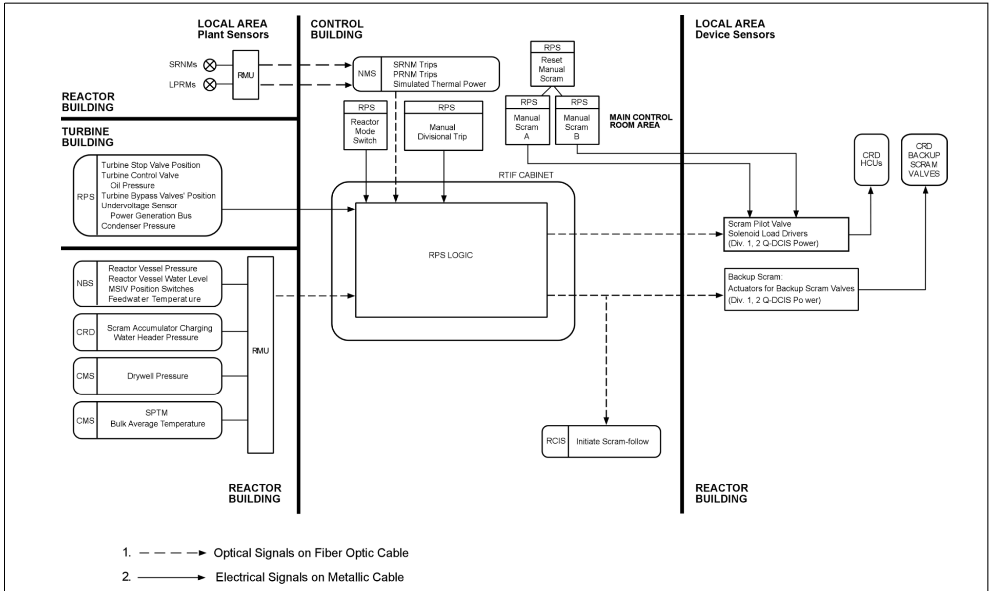
Figure 2.2.7-1. RPS Functional Arrangement
