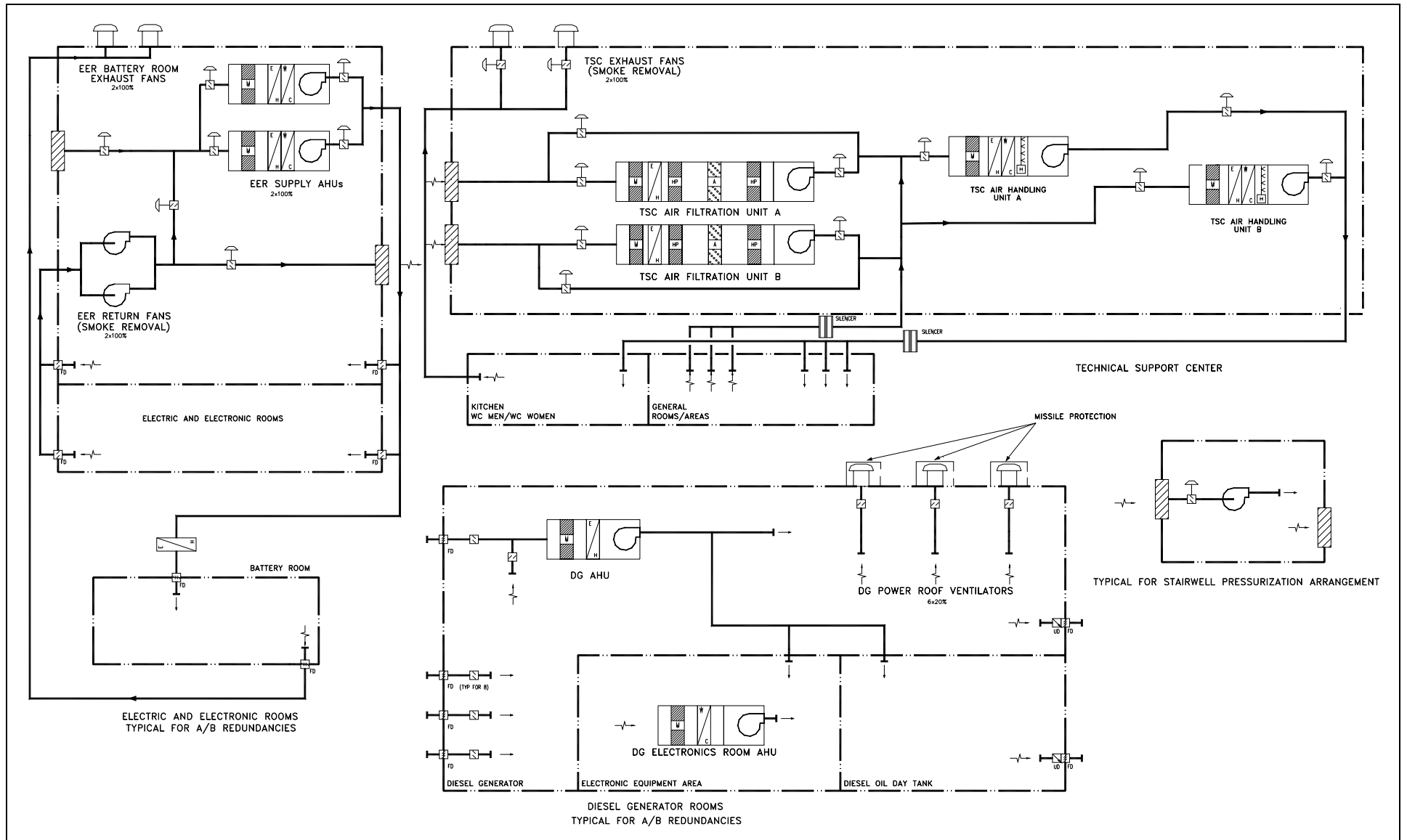
Figure 2.16.2-9. EBVS Functional Arrangement Diagram
