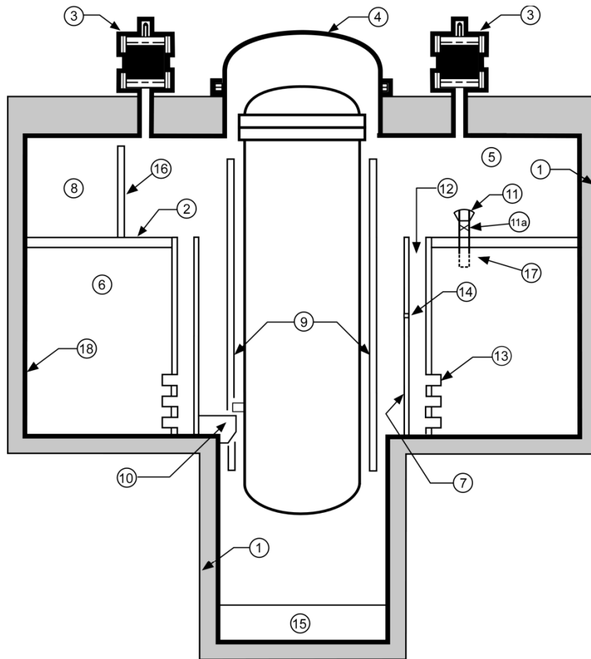
Figure 2.15.1-1. Containment System
