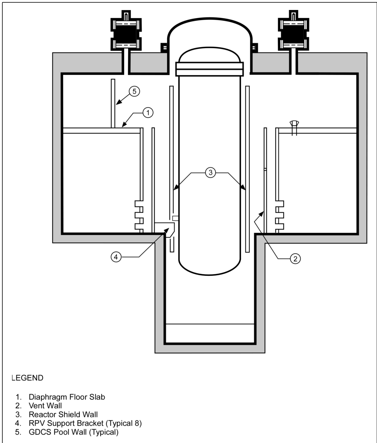
Figure 2.15.3-1. Containment Internal Structures
