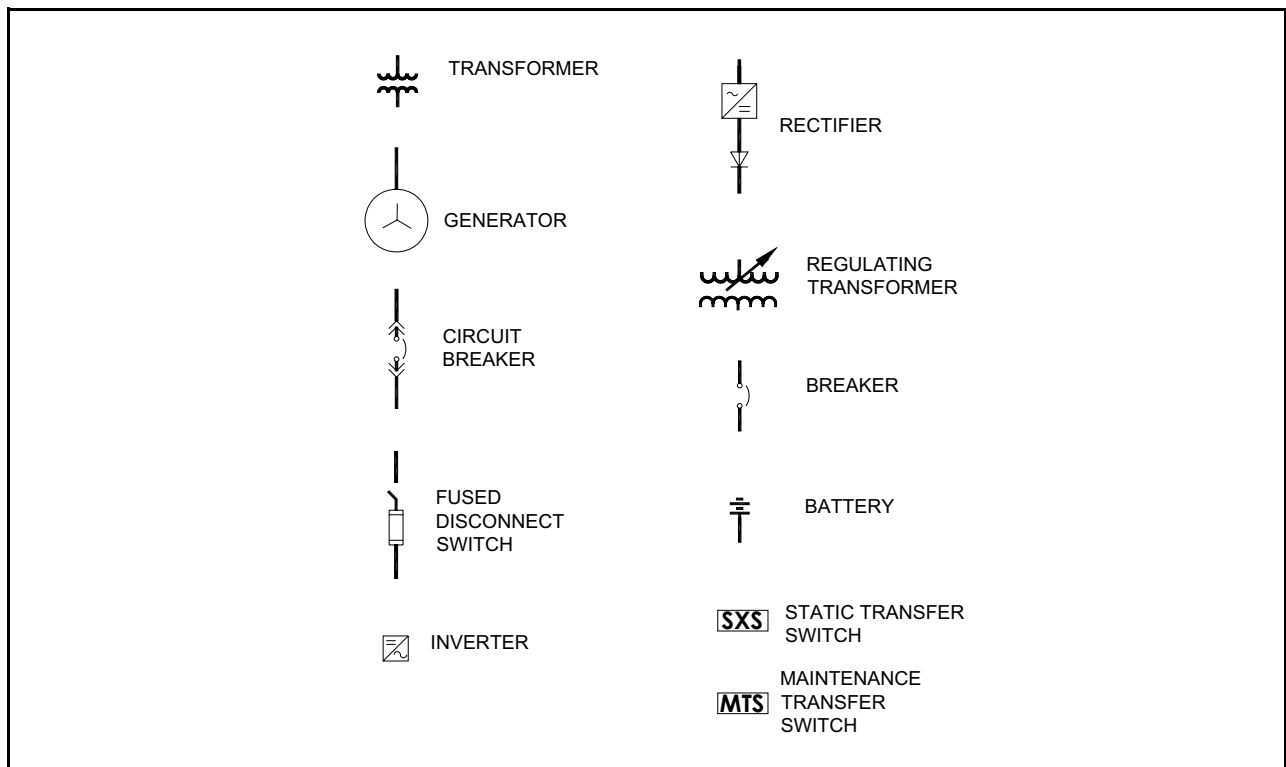
Figure 1.2-2. Legend for Tier 1 Electrical System Diagrams
