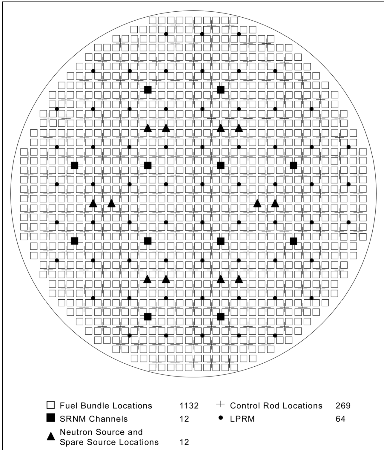
Figure 2.1.1-2. Fuel Bundle, Neutron Sources, Neutron Detectors and Control Rod Functional Arrangement
