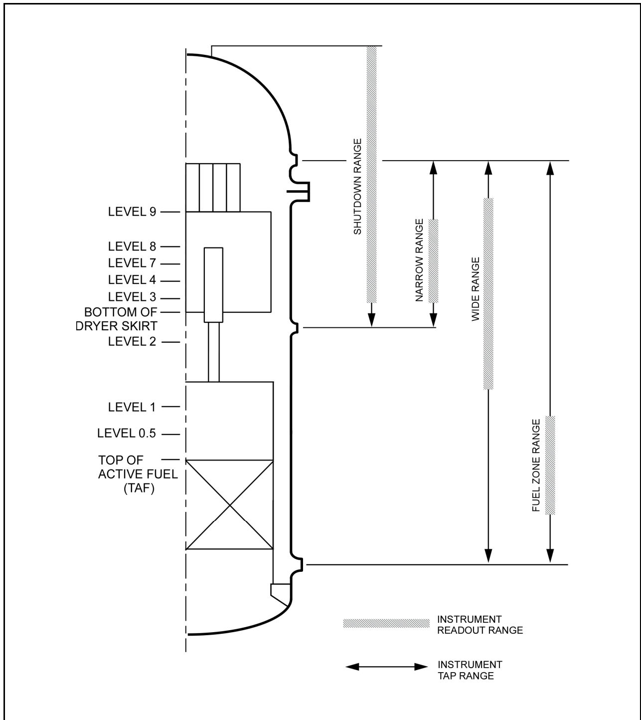
Figure 1.1.1-1 RPV Water Level Range Definition
