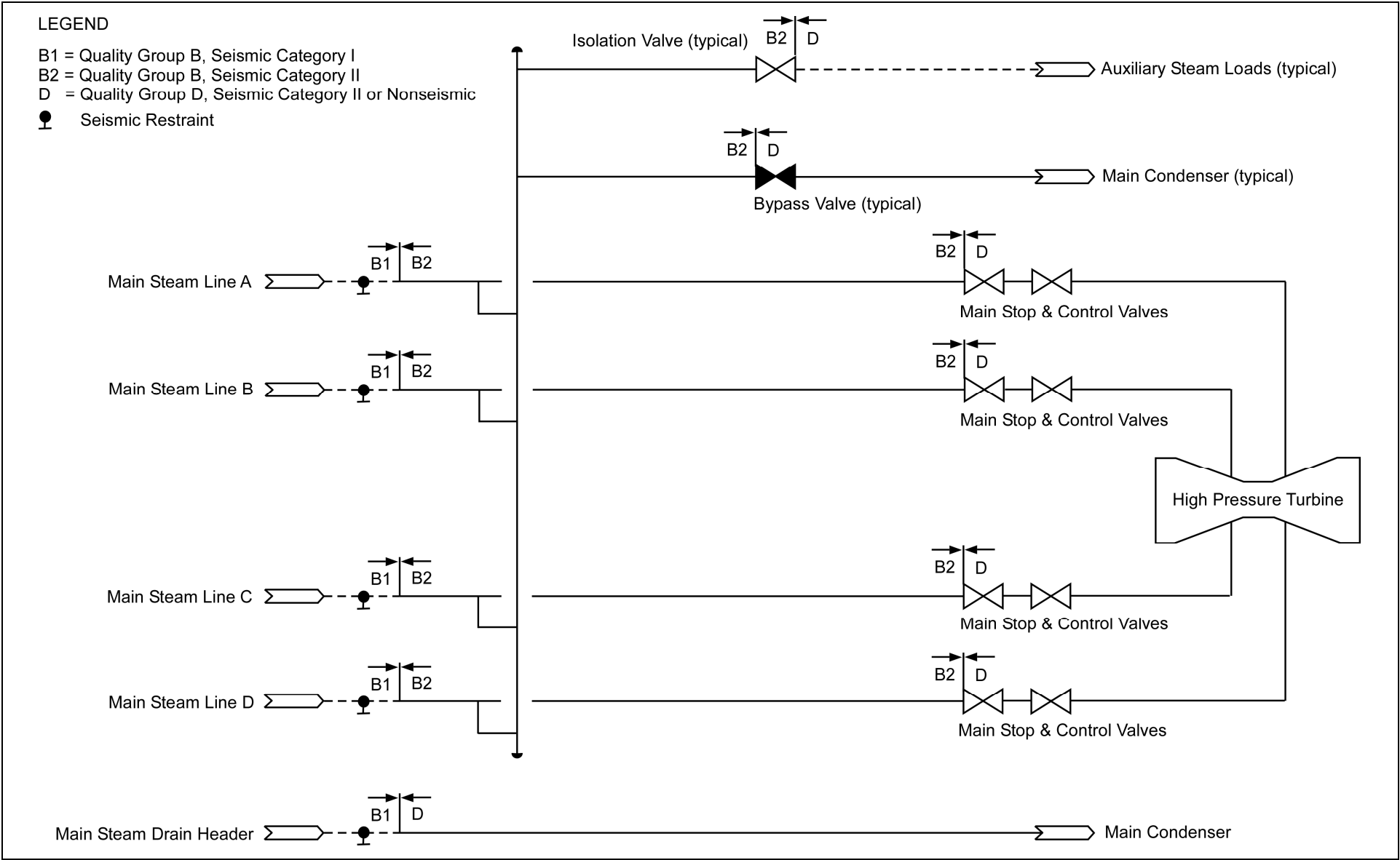
Figure 2.11.1-1. TMSS Functional Arrangement
