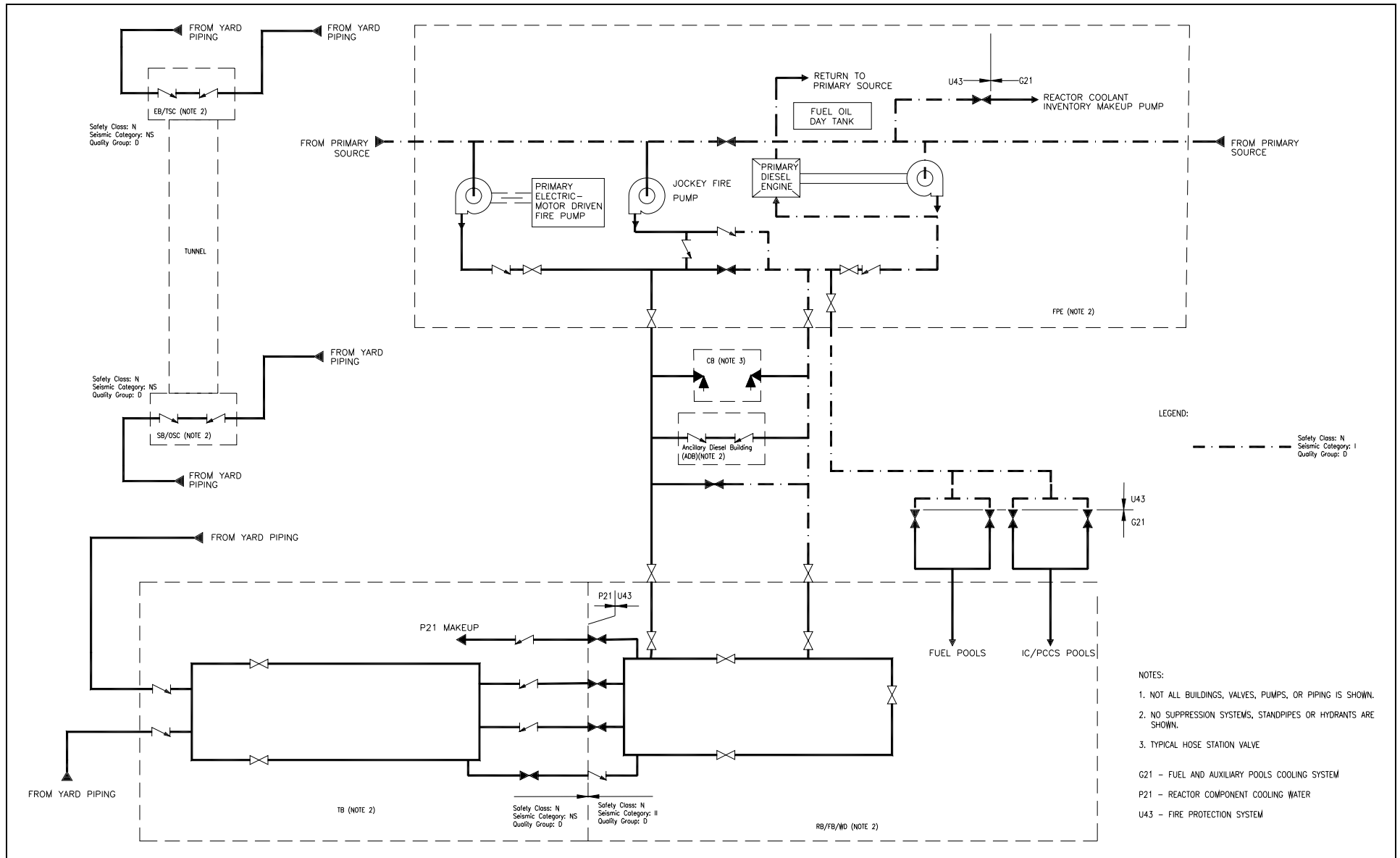
Figure 2.16.3-1. Fire Protection System
