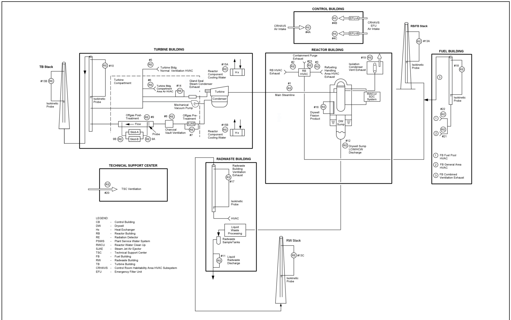
Figure 2.3.1-1. Process Radiation Monitoring System Diagram
