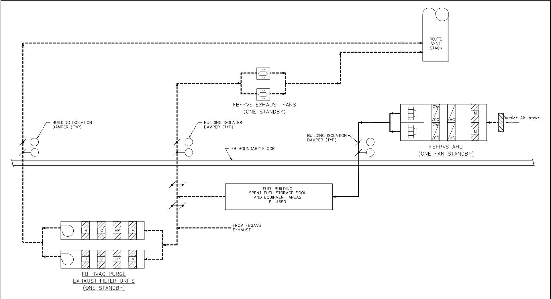
Figure 2.16.2-8. FBFPVS Functional Arrangement Diagram
