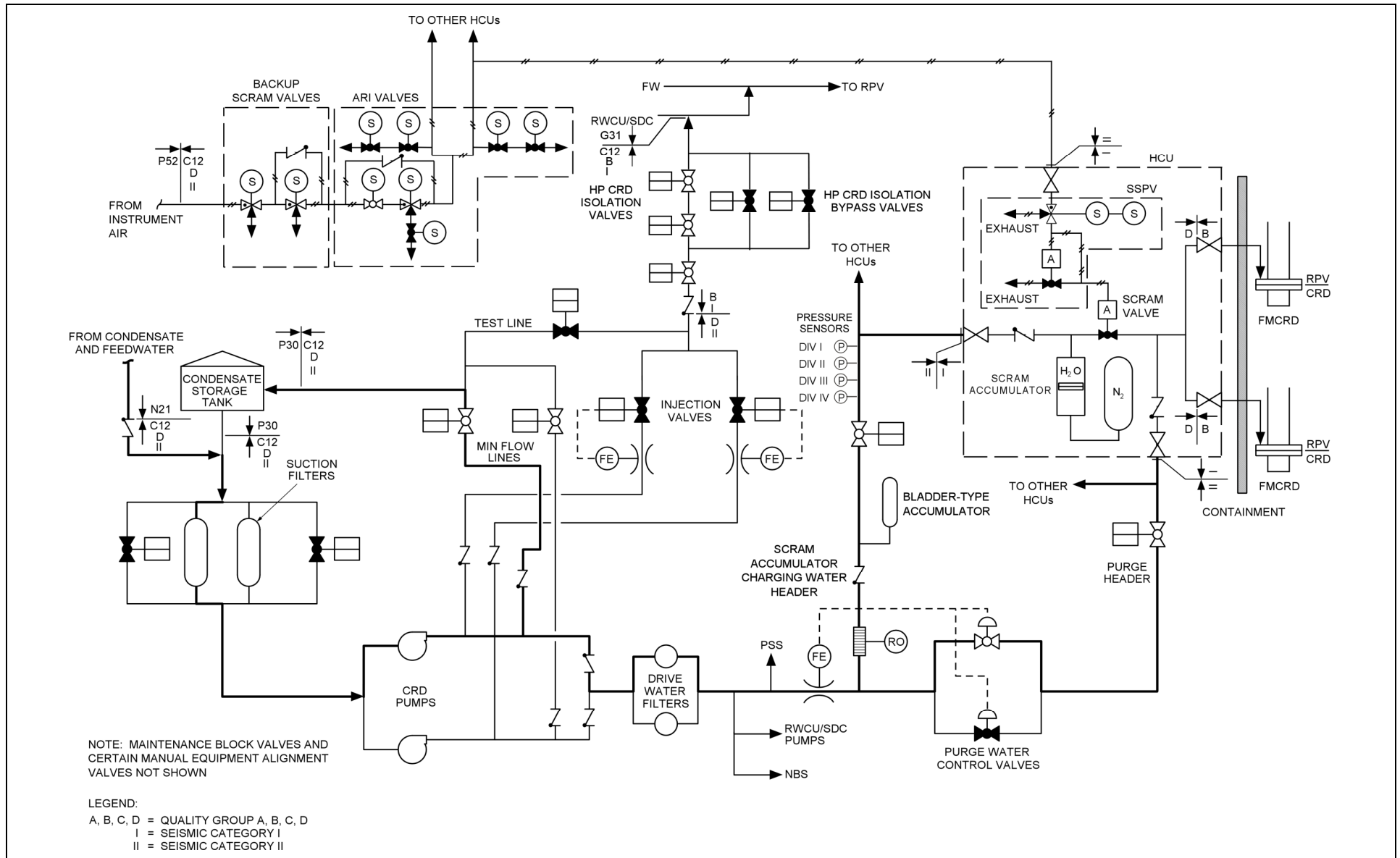
Figure 2.2.2-1. Control Rod Drive System
