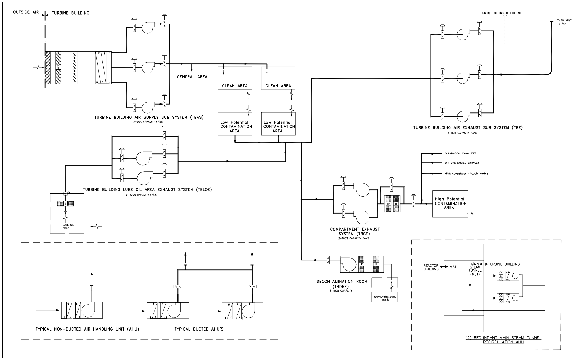
Figure 2.16.2-6. TBVS Functional Arrangement Diagram
