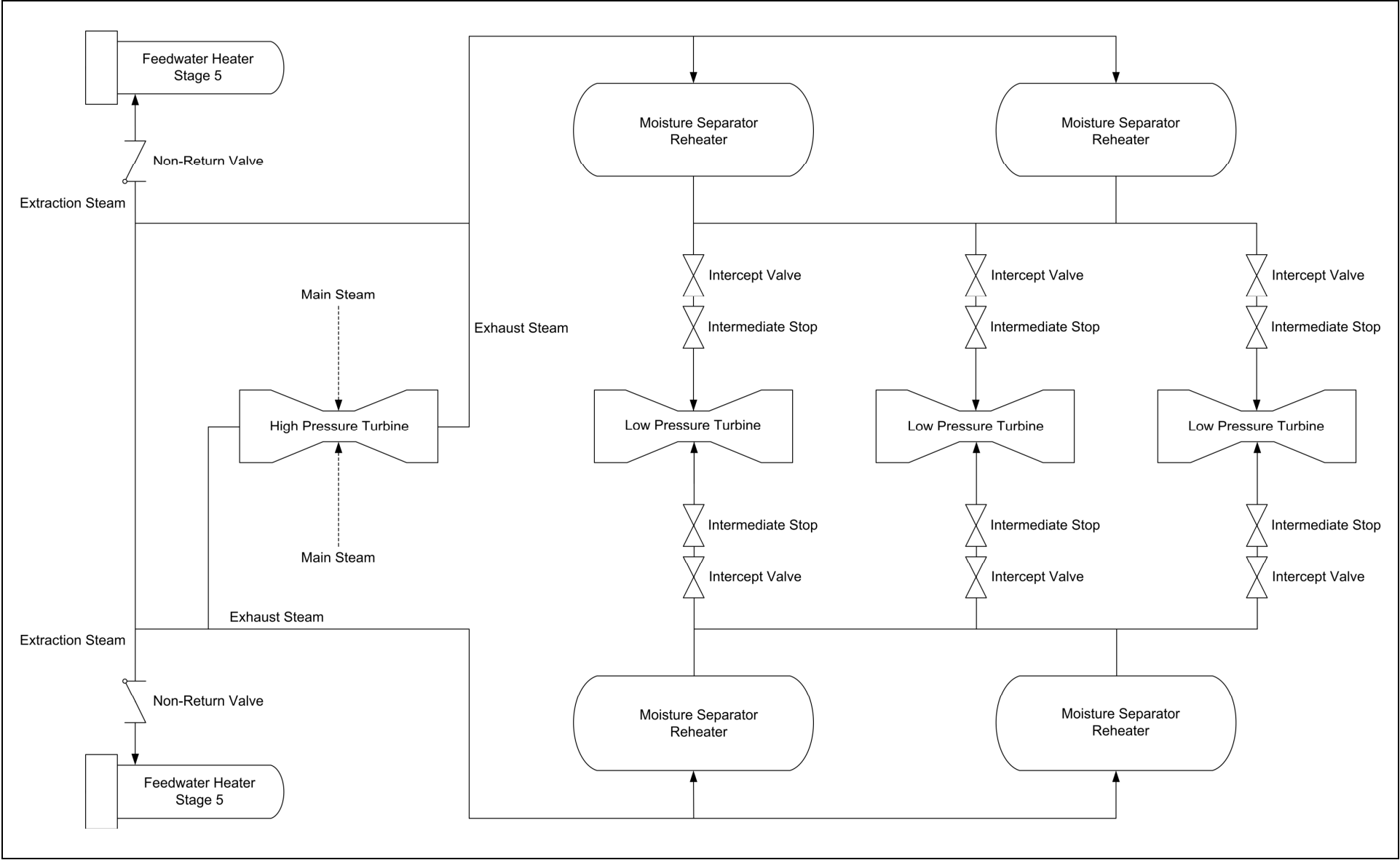
Figure 2.11.1-2. High Pressure Turbine Exhaust Functional Arrangement
