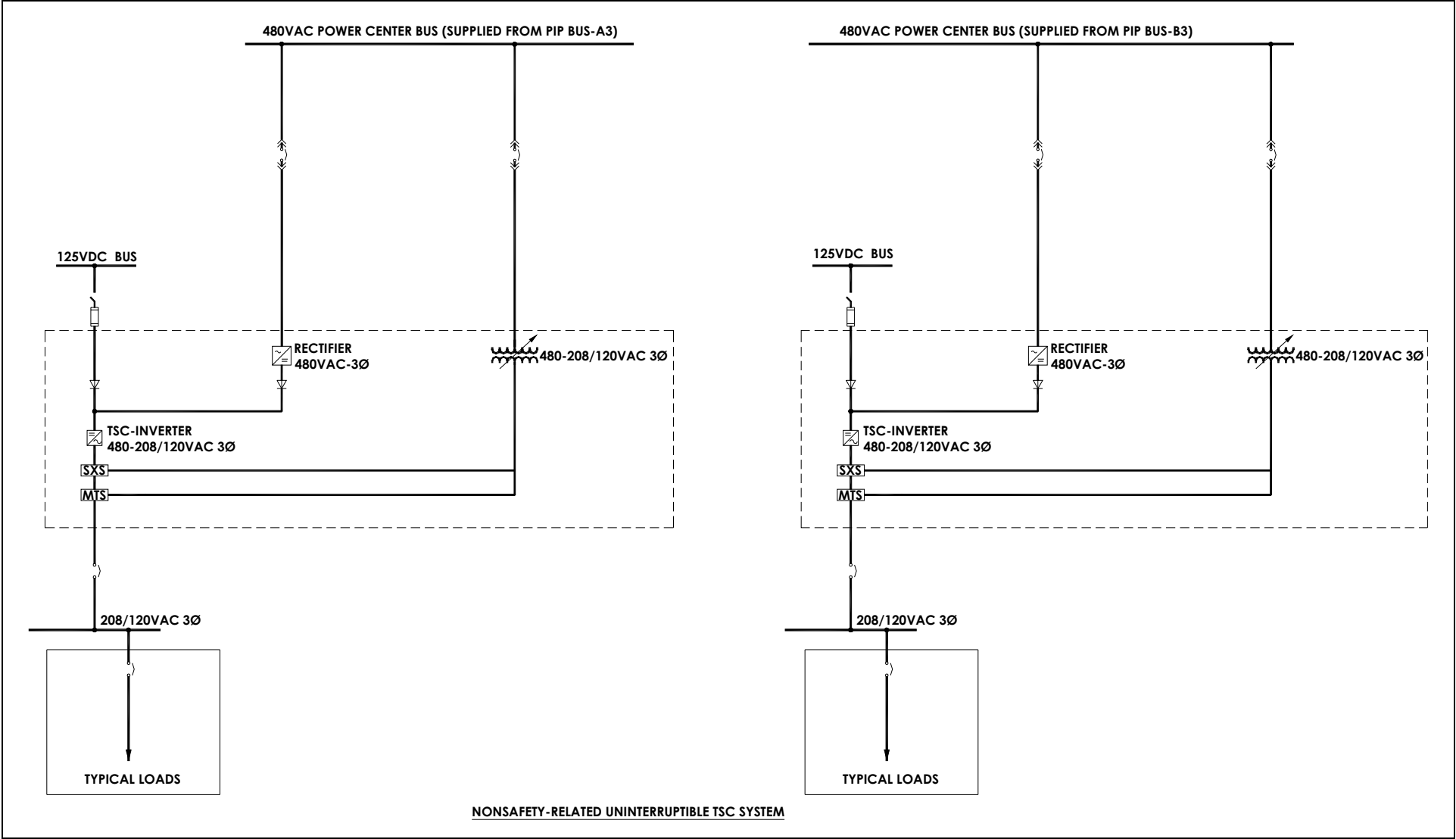
Figure 2.13.5-2. Sh 2. Nonsafety-Related UPS System Functional Arrangement
