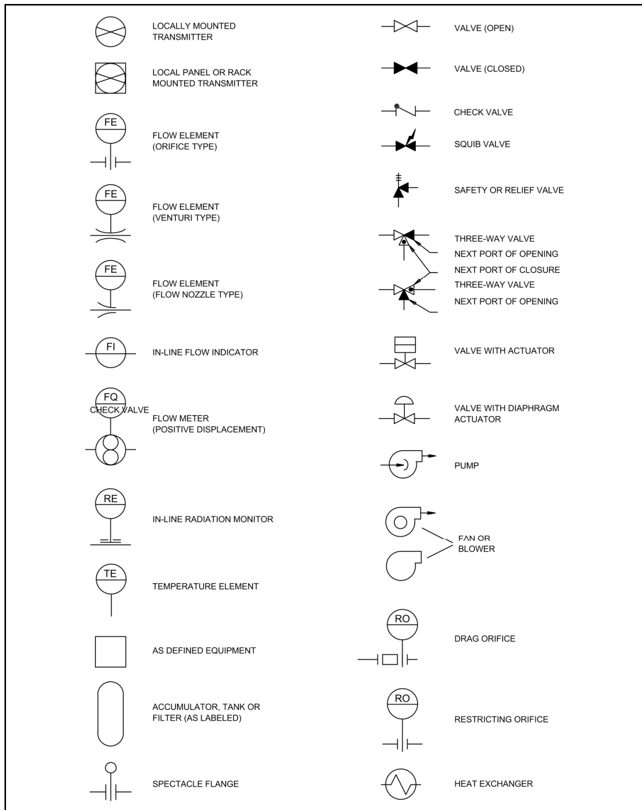
Figure 1.2-1. Legend for Tier 1 System Diagrams
