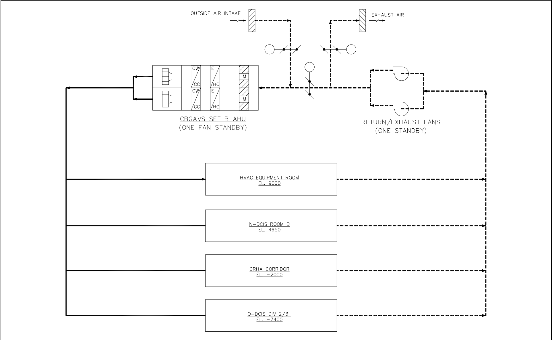
Figure 2.16.2-5b. CBGAVS (Set B) Functional Arrangement Diagram
