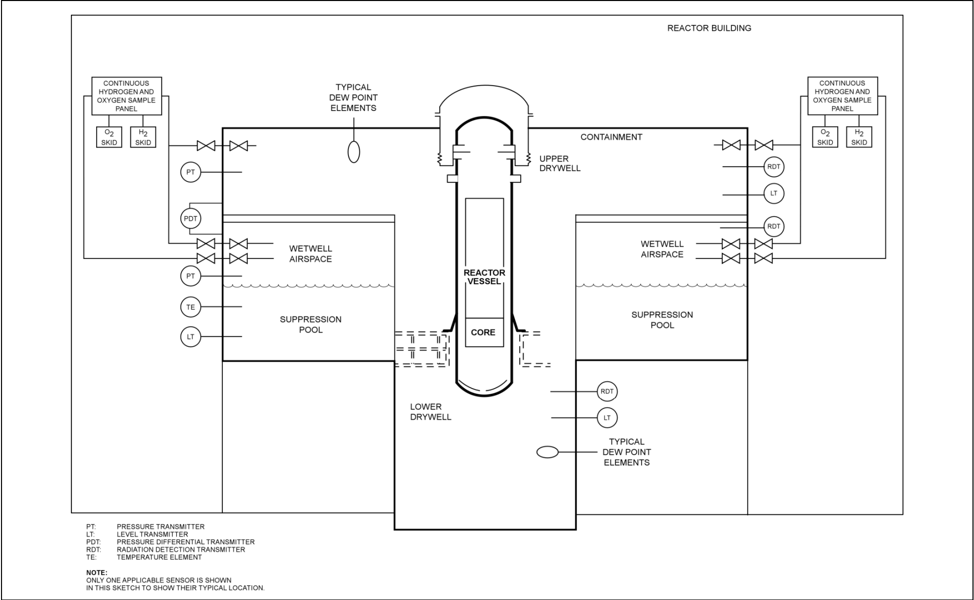
Figure 2.15.7-1. Containment Monitoring System Functional Arrangement
