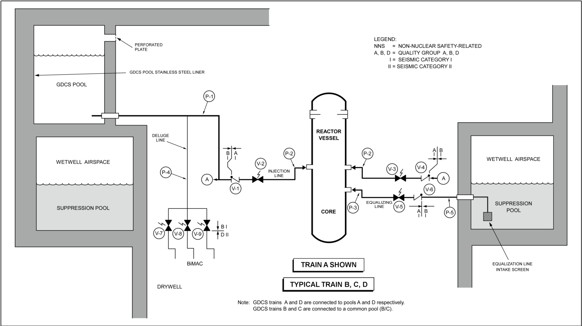
Figure 2.4.2-1. Gravity-Driven Cooling System
