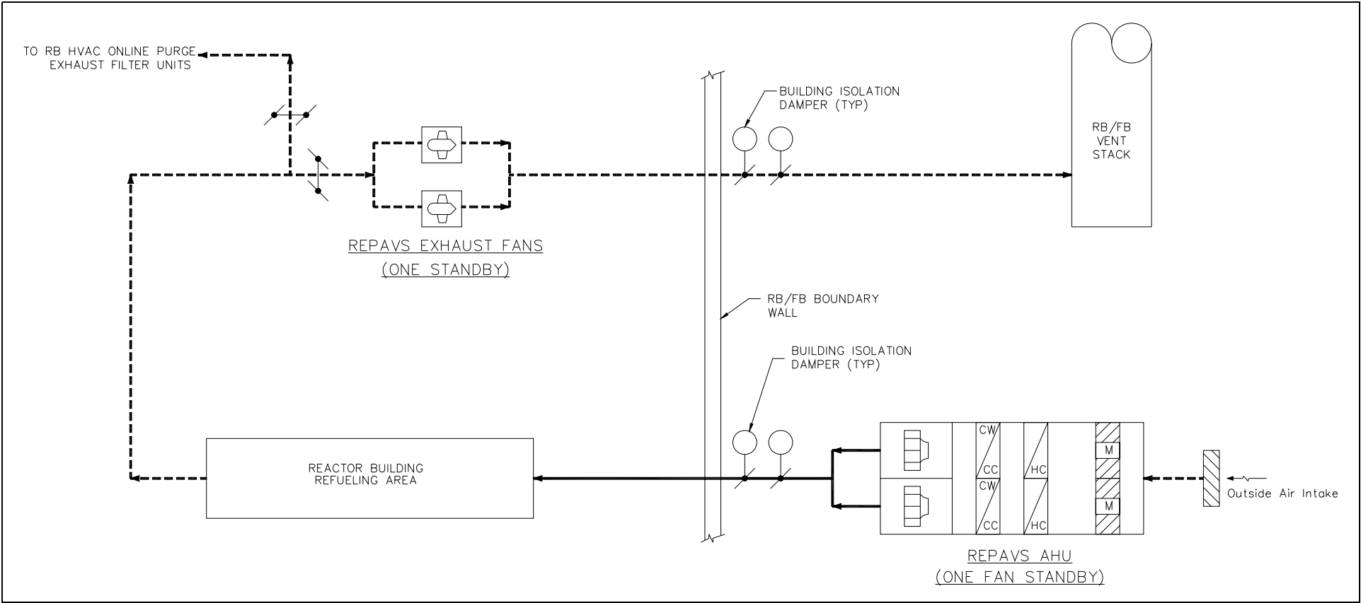
Figure 2.16.2-3. REPAVS Functional Arrangement Diagram
