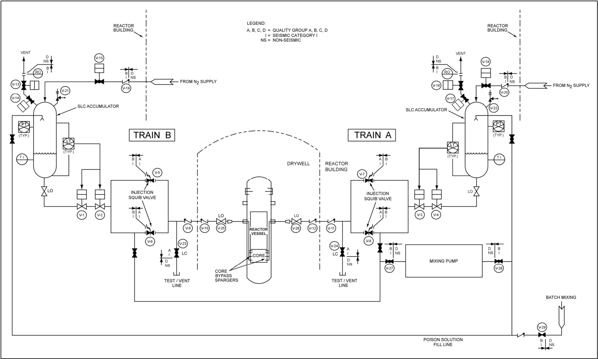
Figure 2.2.4-1. Standby Liquid Control System Simplified Diagram
