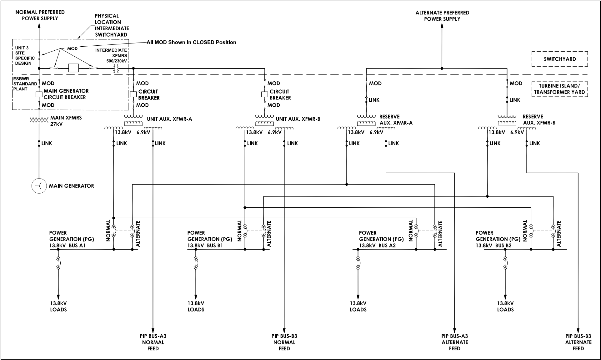
Figure 2.13.1-1 Sh 1. Electric Power Distribution System Functional Arrangement
