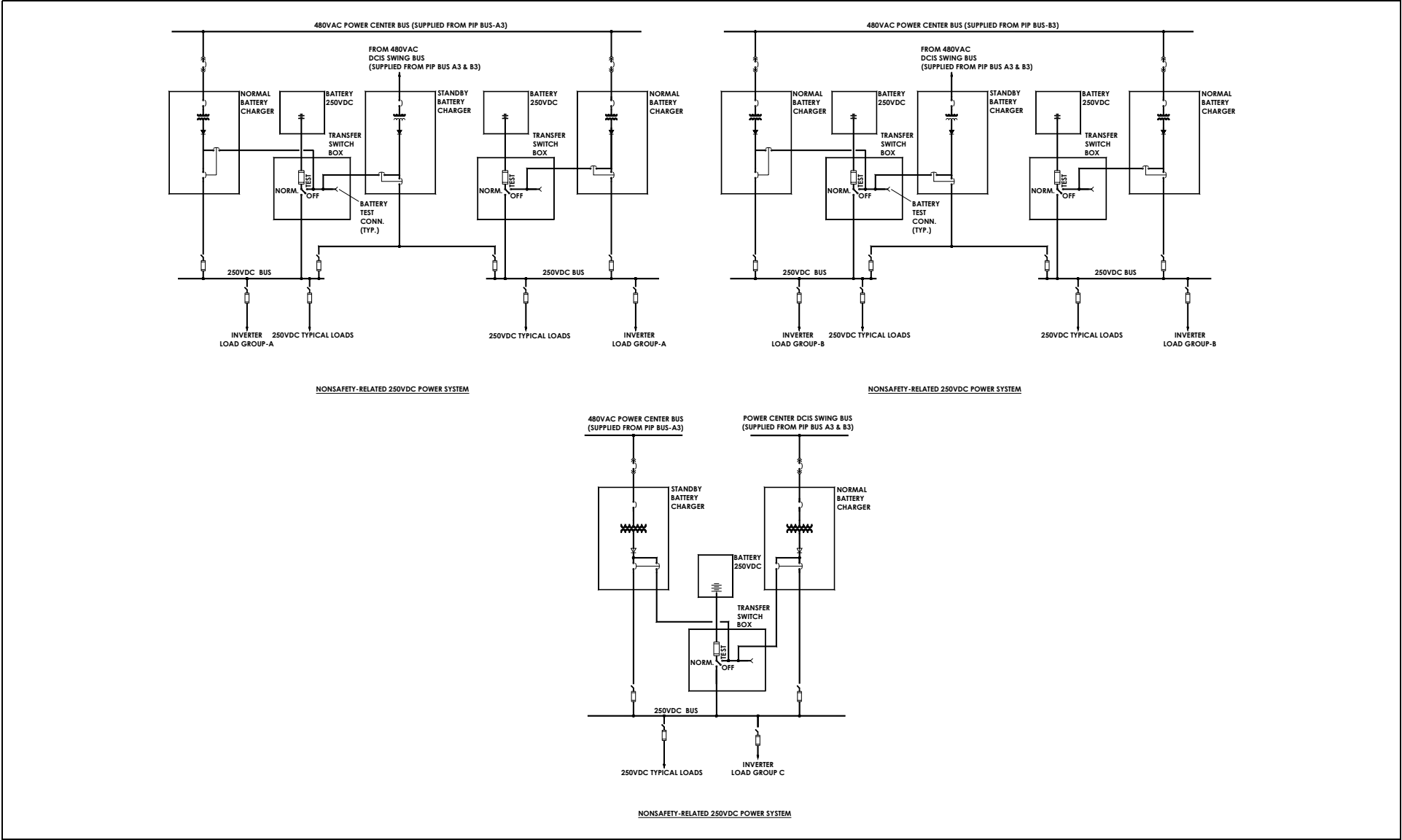
Figure 2.13.3-2 Sh 1. Nonsafety-Related 250 VDC System Functional Arrangement
