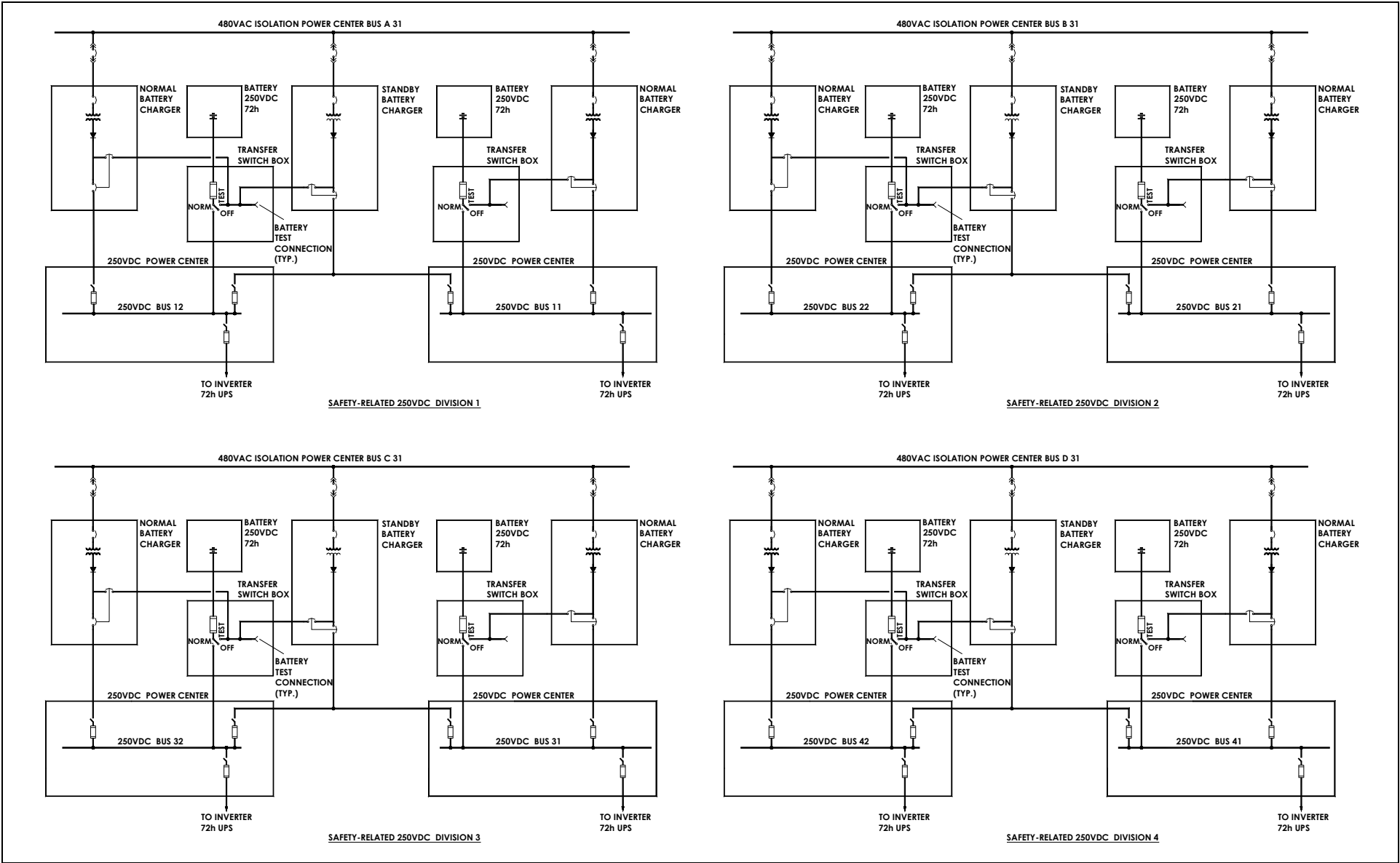
Figure 2.13.3-1. Safety-Related 250 VDC System Functional Arrangement
