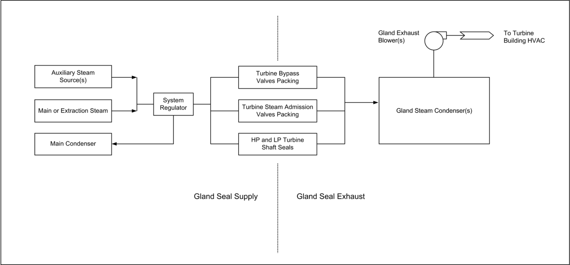
Figure 2.11.5-1. Turbine Gland Seal System Arrangement
