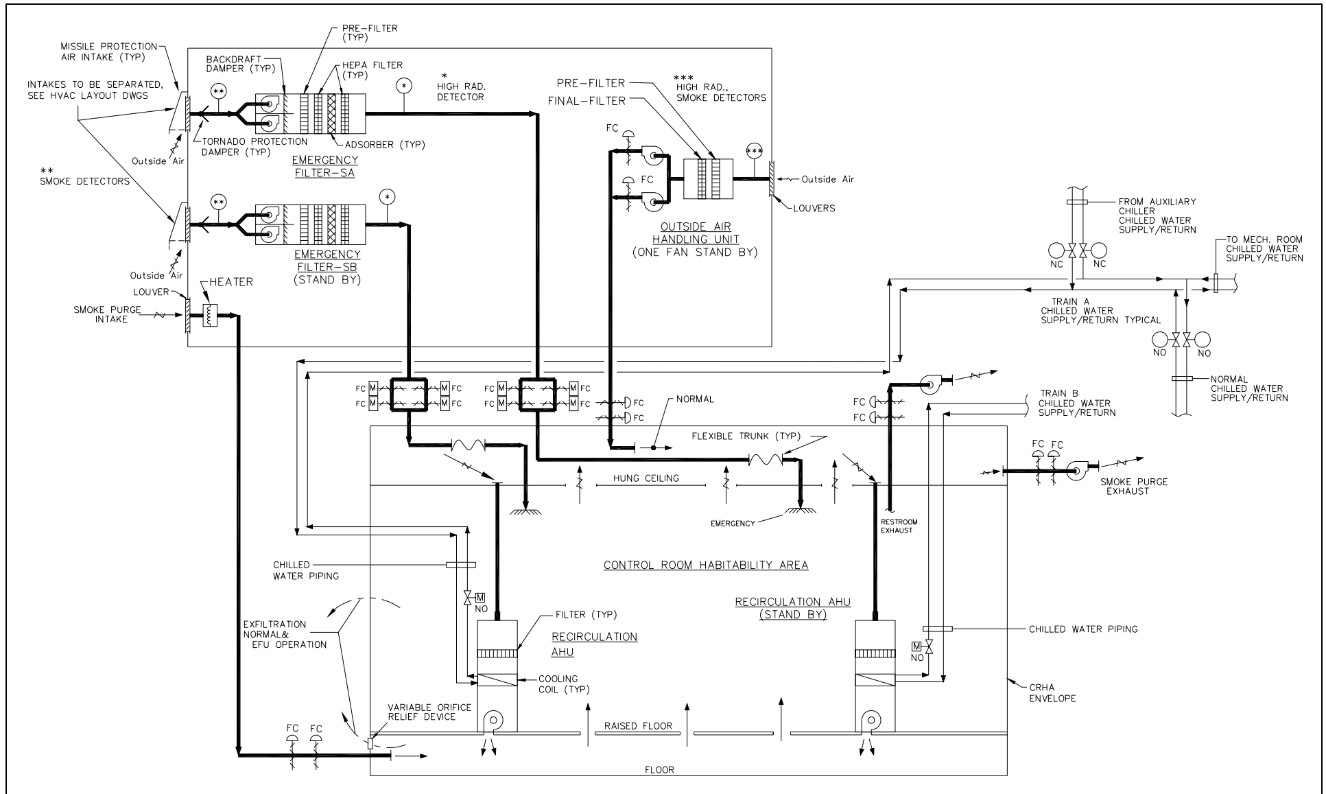
Figure 2.16.2-4. CRHAVS Functional Arrangement Diagram
