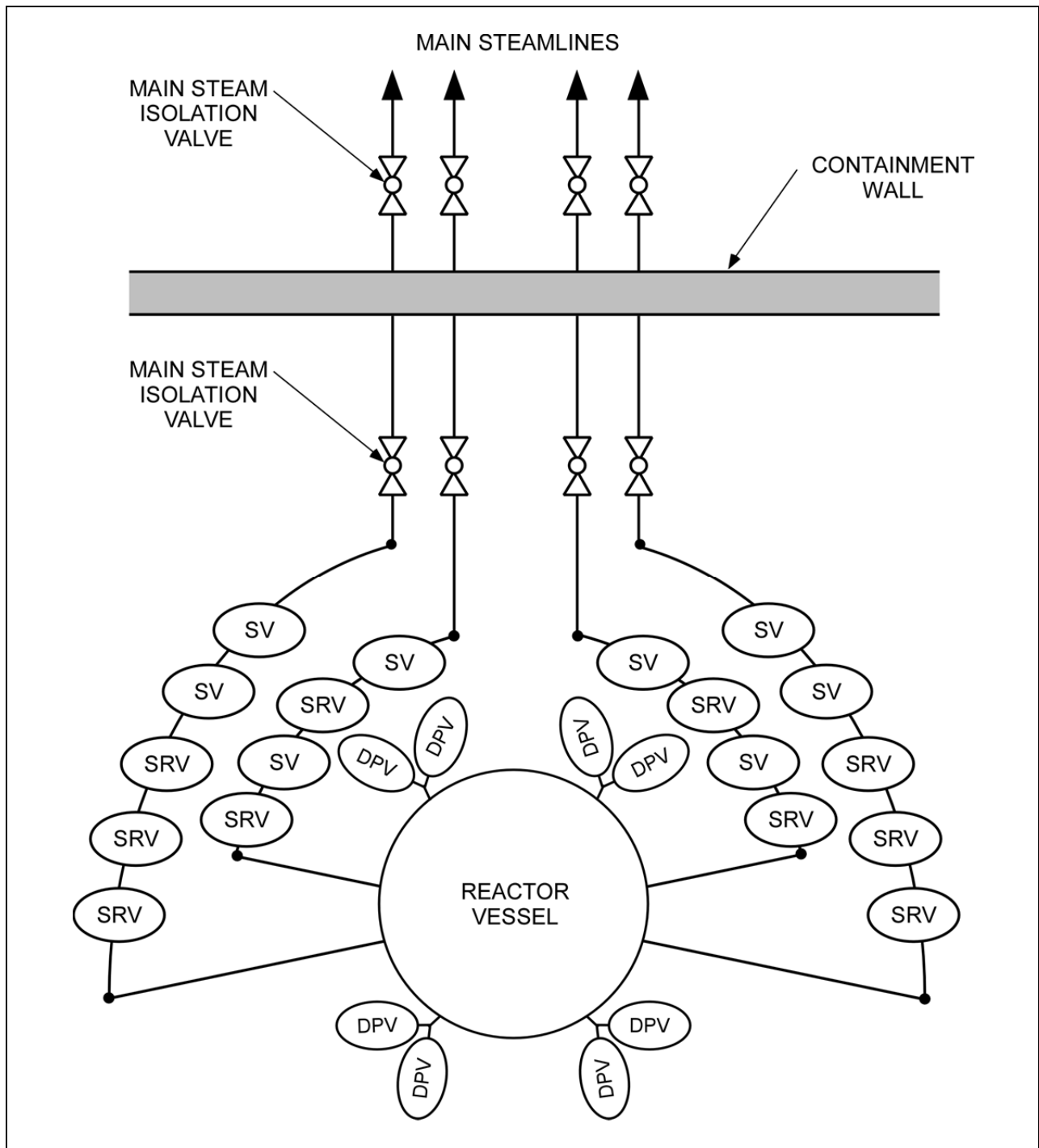
Figure 2.1.2-1. Safety Relief Valves, Depressurization Valves and Steamline Diagram
