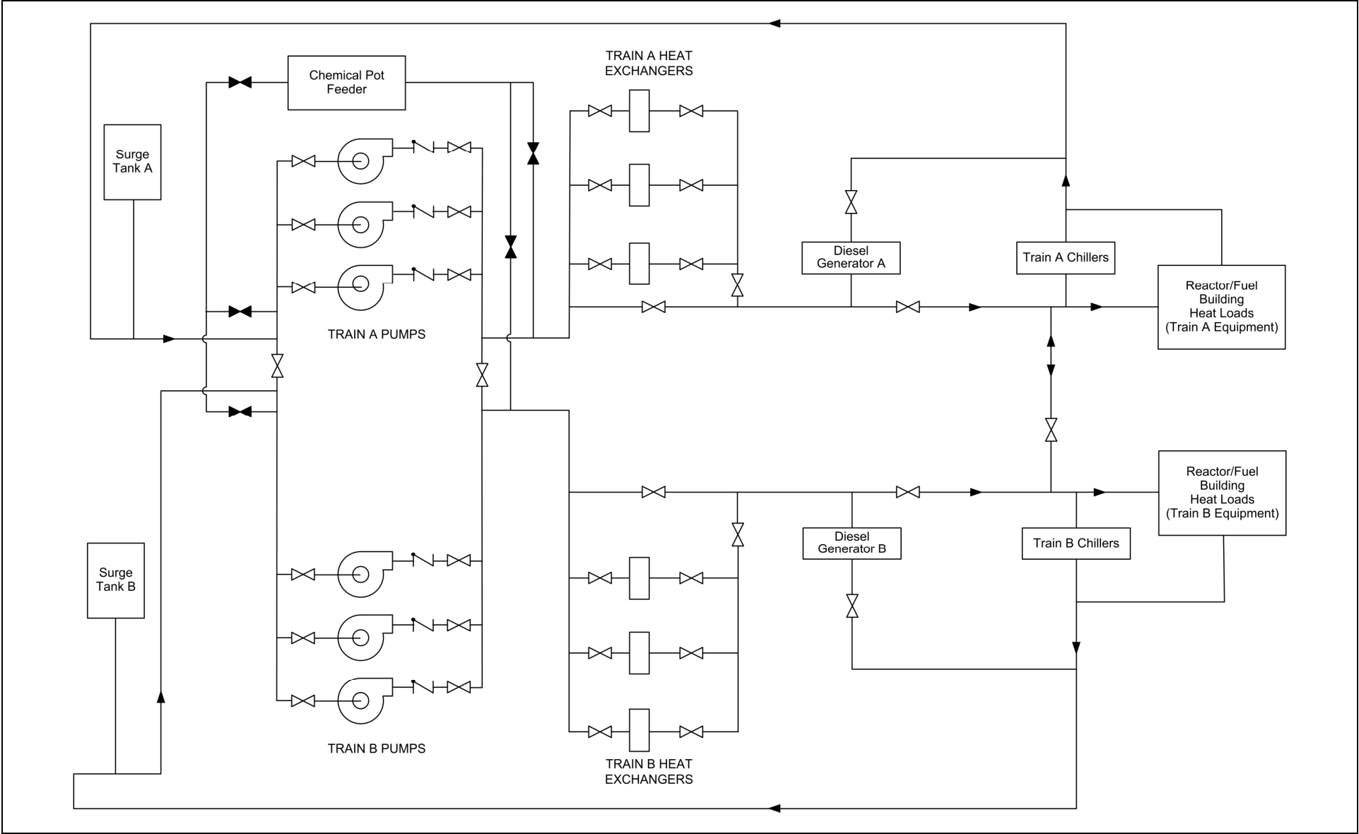
Figure 2.12.3-1. Reactor Component Cooling Water System Functional Arrangement
