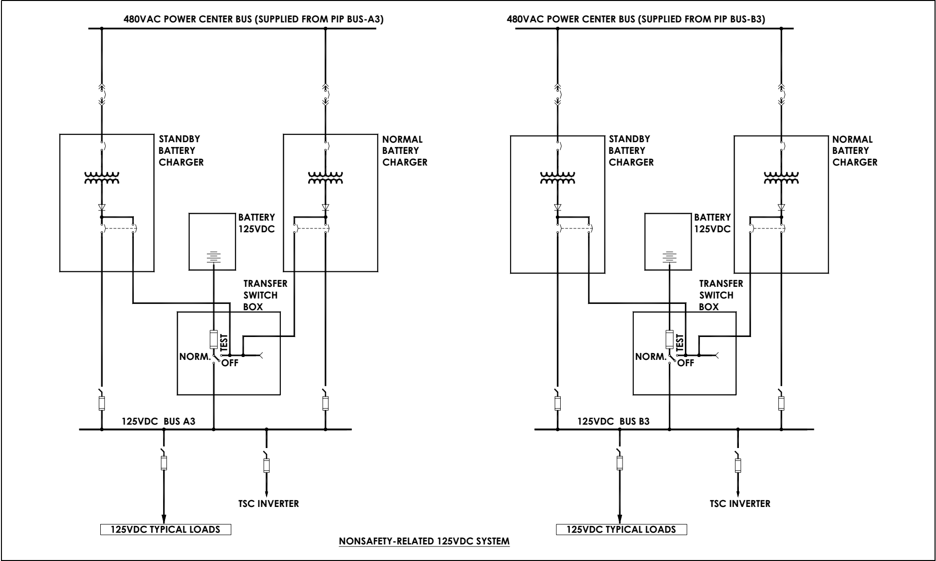
Figure 2.13.3-2 Sh 2. Nonsafety-Related 125 VDC System Functional Arrangement
