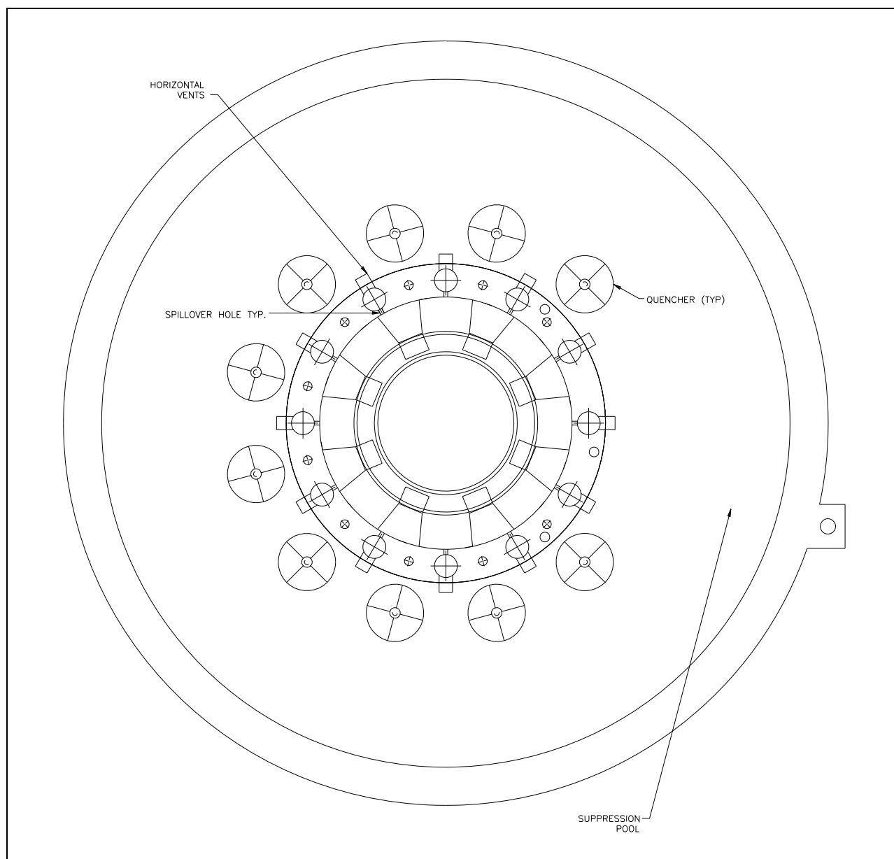
Figure 2.1.2-3. Safety Relief Valve Discharge Line Quencher Arrangement
