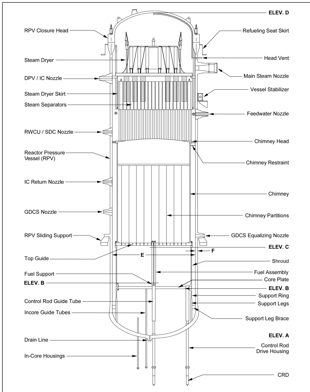
Figure 2.1.1-1. Reactor Pressure Vessel and Internals Key Features Layout
