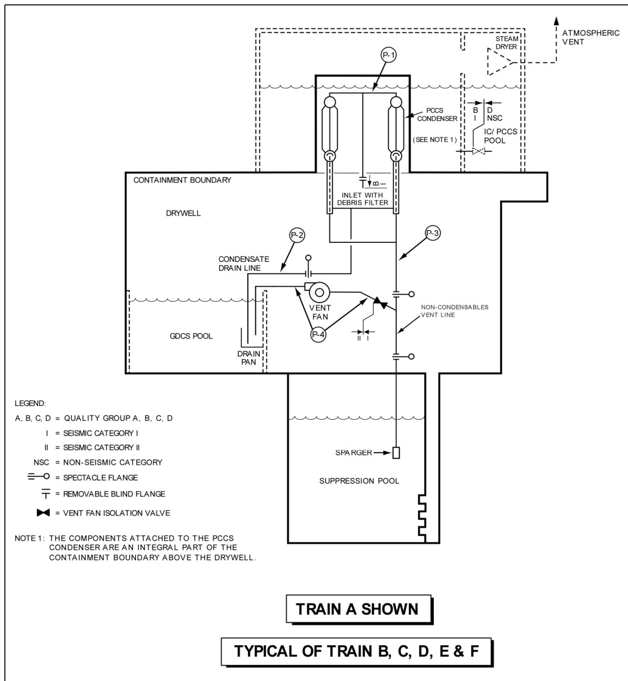
Figure 2.15.4-1. Passive Containment Cooling System Schematic
