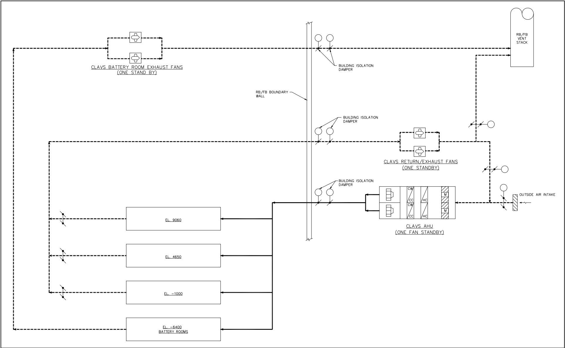
Figure 2.16.2-1. CLAVS Functional Arrangement Diagram (Typical Train A/B)
