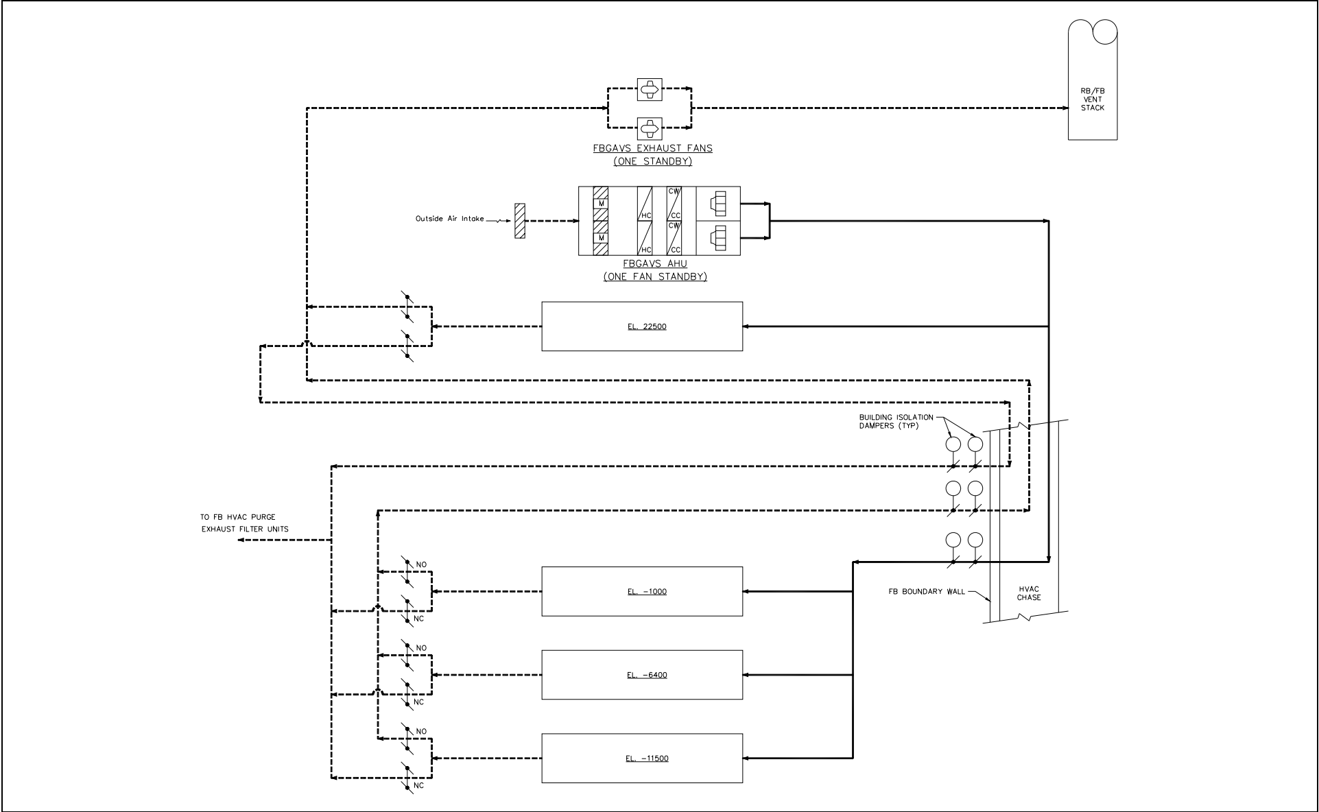
Figure 2.16.2-7. FBGAVS Functional Arrangement Diagram
