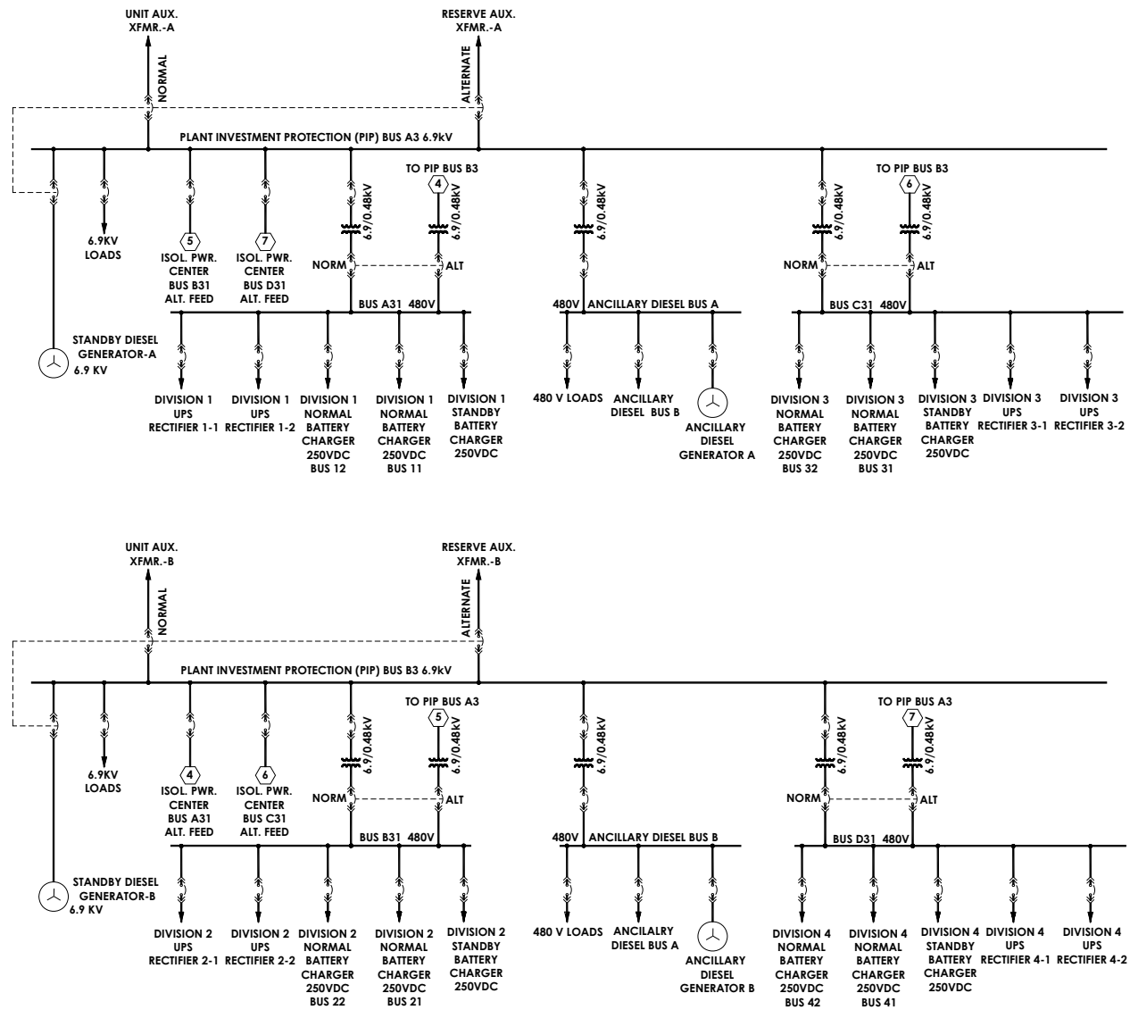
Figure 2.13.1-1 Sh 2. Electric Power Distribution System Functional Arrangement
