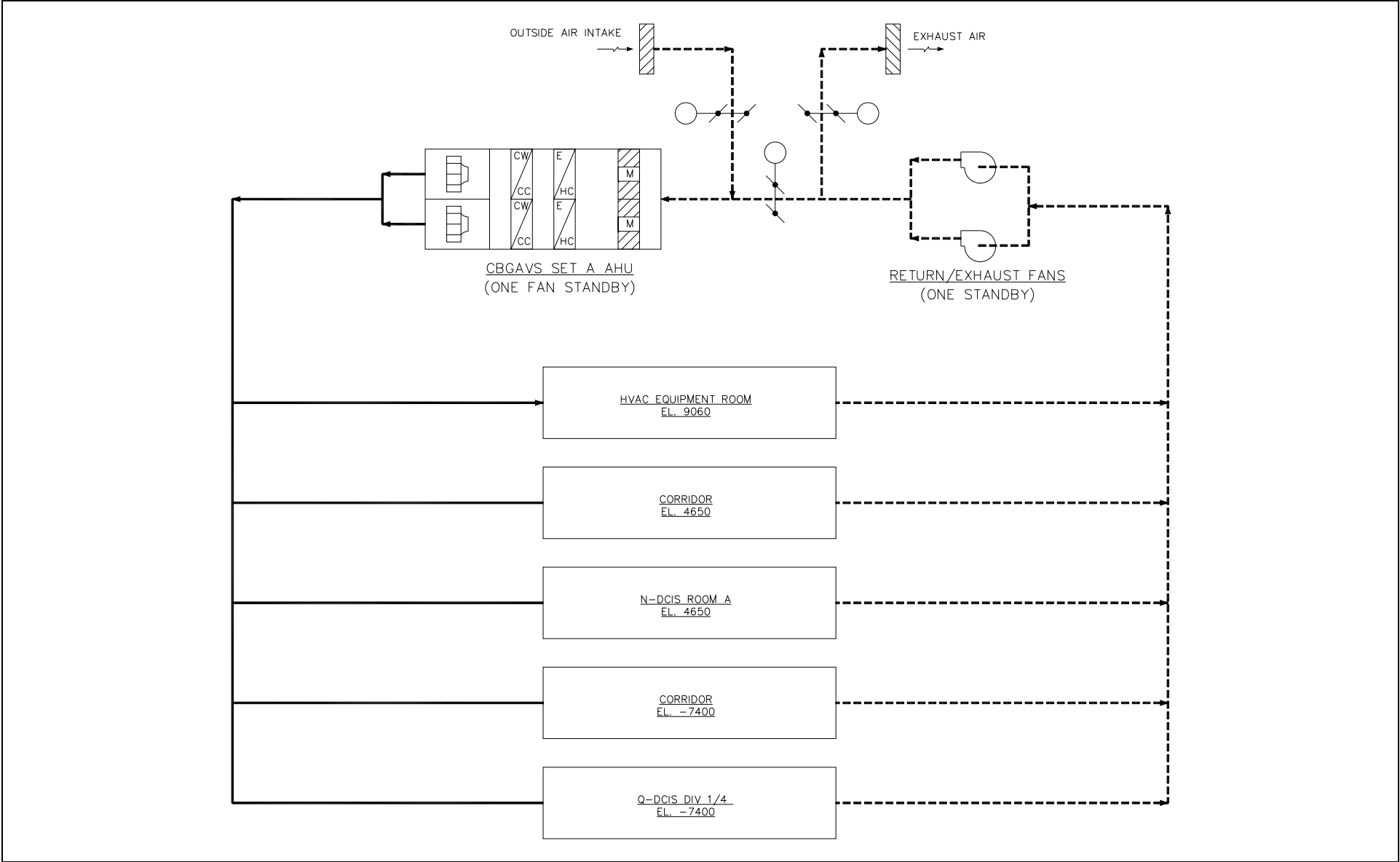
Figure 2.16.2-5a. CBGAVS (Set A) Functional Arrangement Diagram
