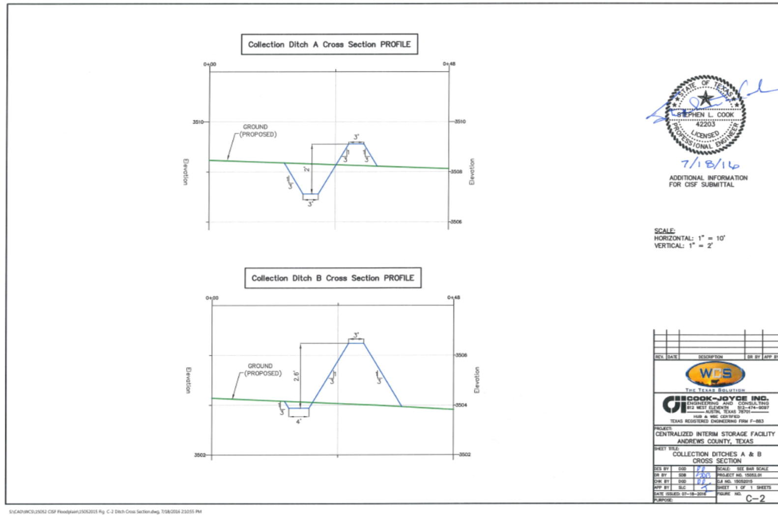
Figure 2-27 CJI C-2 Collection Ditches A & B Cross Section
