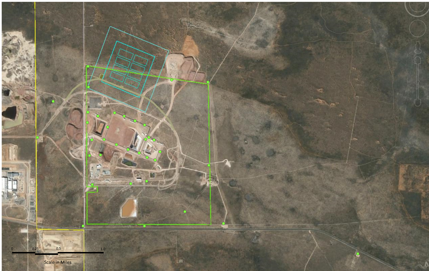
Figure 4.12-10 On-site Thermoluminescent dosimeters (TLDs) or Optically Stimulated Luminescent dosimeters (OSLs) monitoring locations (36 locations in 2014).
