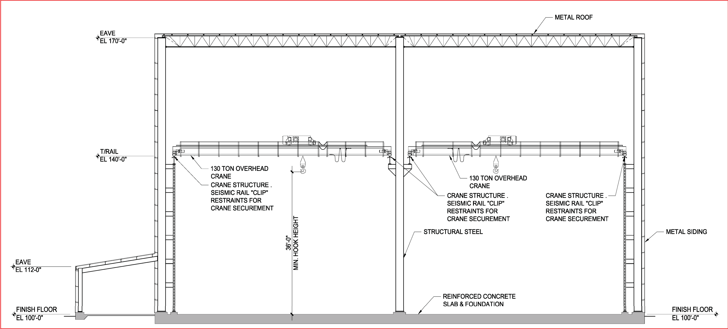
Figure 1-8 Cask Handling Building Section View
