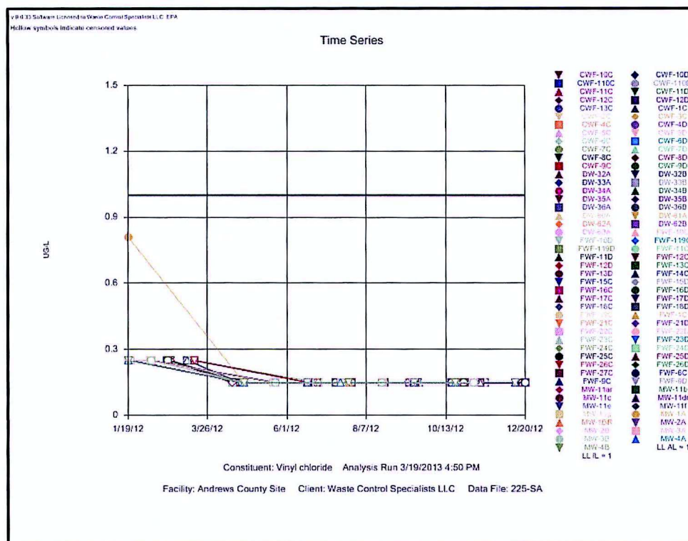
Figure 128 : Vinyl Chloride Concentration in 225' Zone Groundwater
