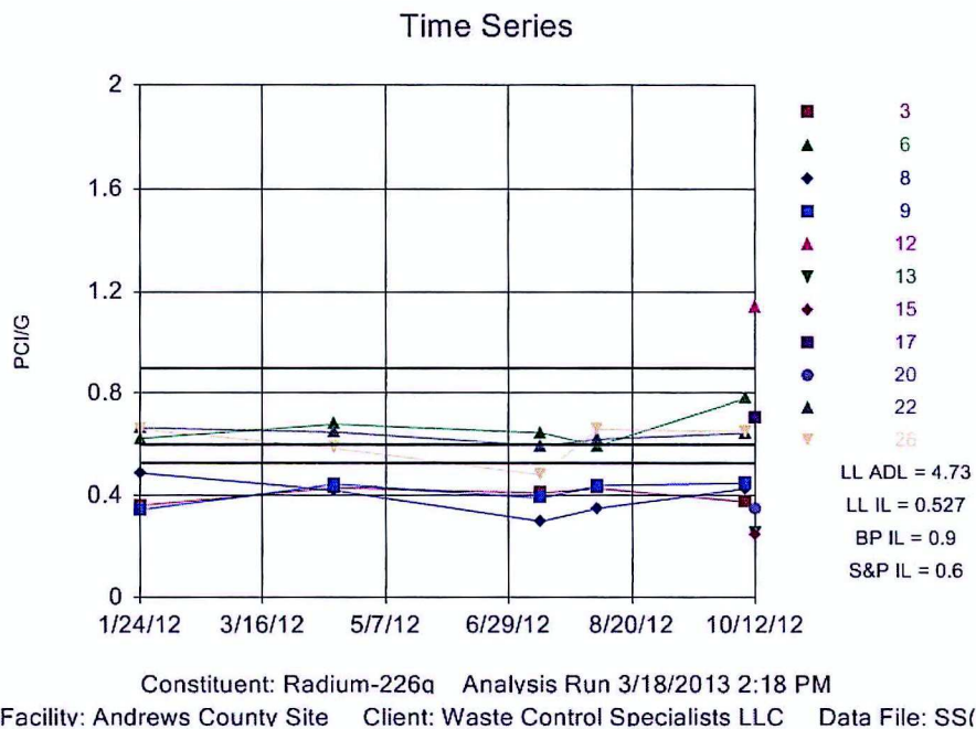
Figure 10 : Radium-226 Activity Concentration in Soil (0-2")
