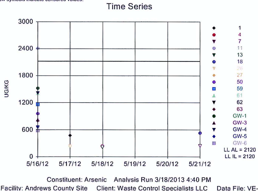
Figure 60 : Arsenic Concentration in Vegetation
