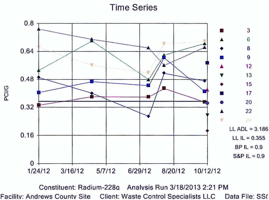
Figure 11 : Radium-228 Activity Concentration in Soil (0-2")
