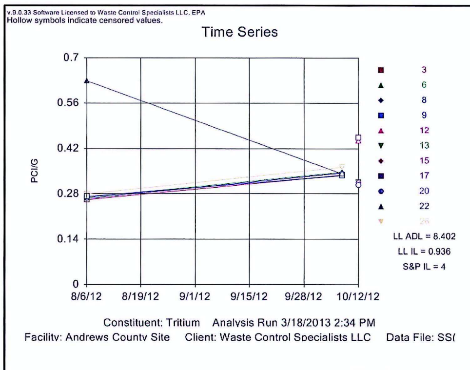
Figure 15 : Tritium Activity Concentration in Soil (0-2")
