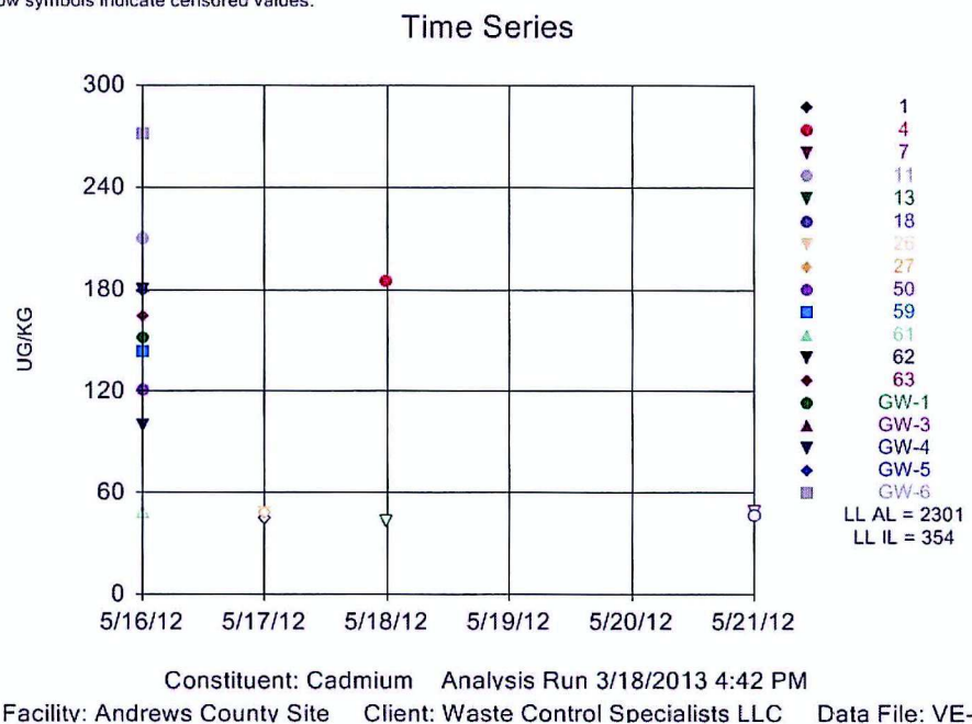
Figure 61 : Cadmium Concentration in Vegetation
