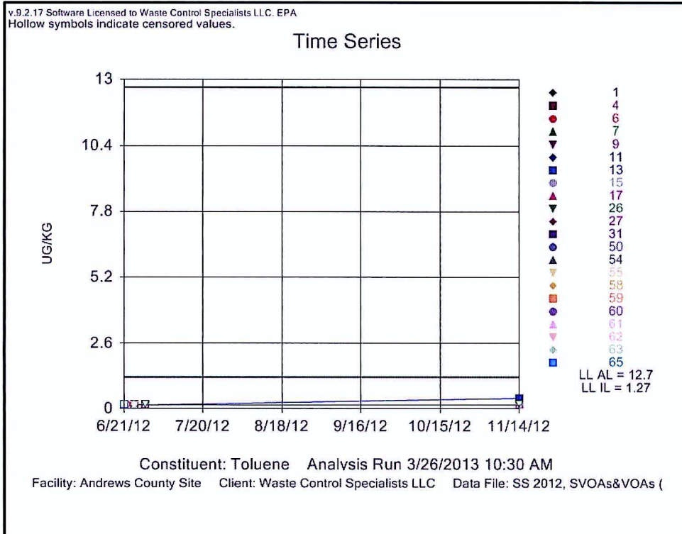
Figure 24 : Toluene Concentration in Soil (0-2")
