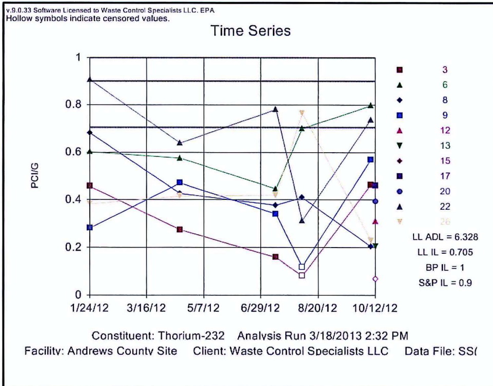
Figure 14 : Thorium-232 Activity Concentration in Soil (0-2")
