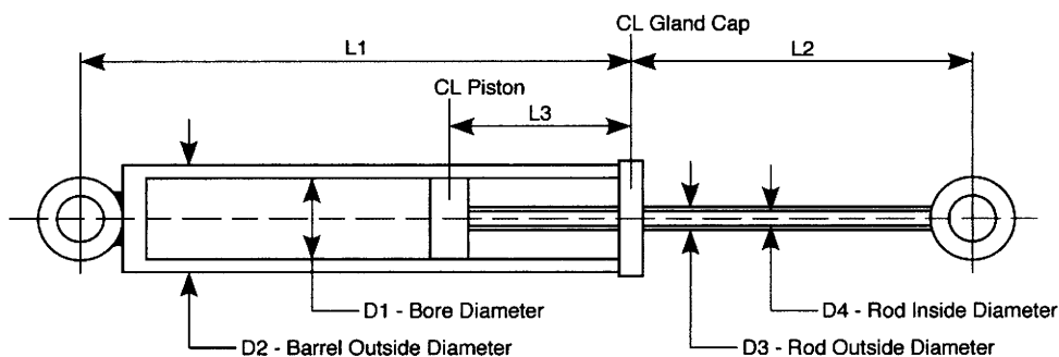
Dimension Notation
