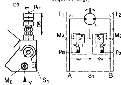
Port plate 192 (pressure relief valves with pressure sequence range)
