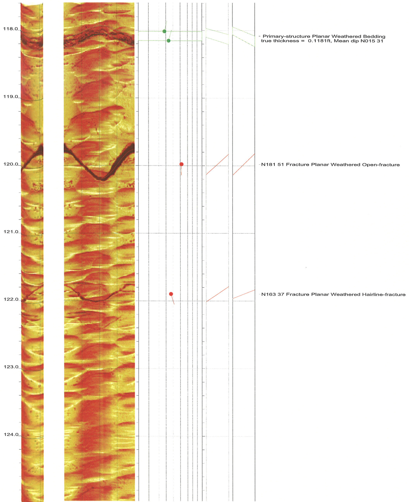
North Anna COL Boring B-909 Acoustic Televiwer Dips Sheet 17 of 28
