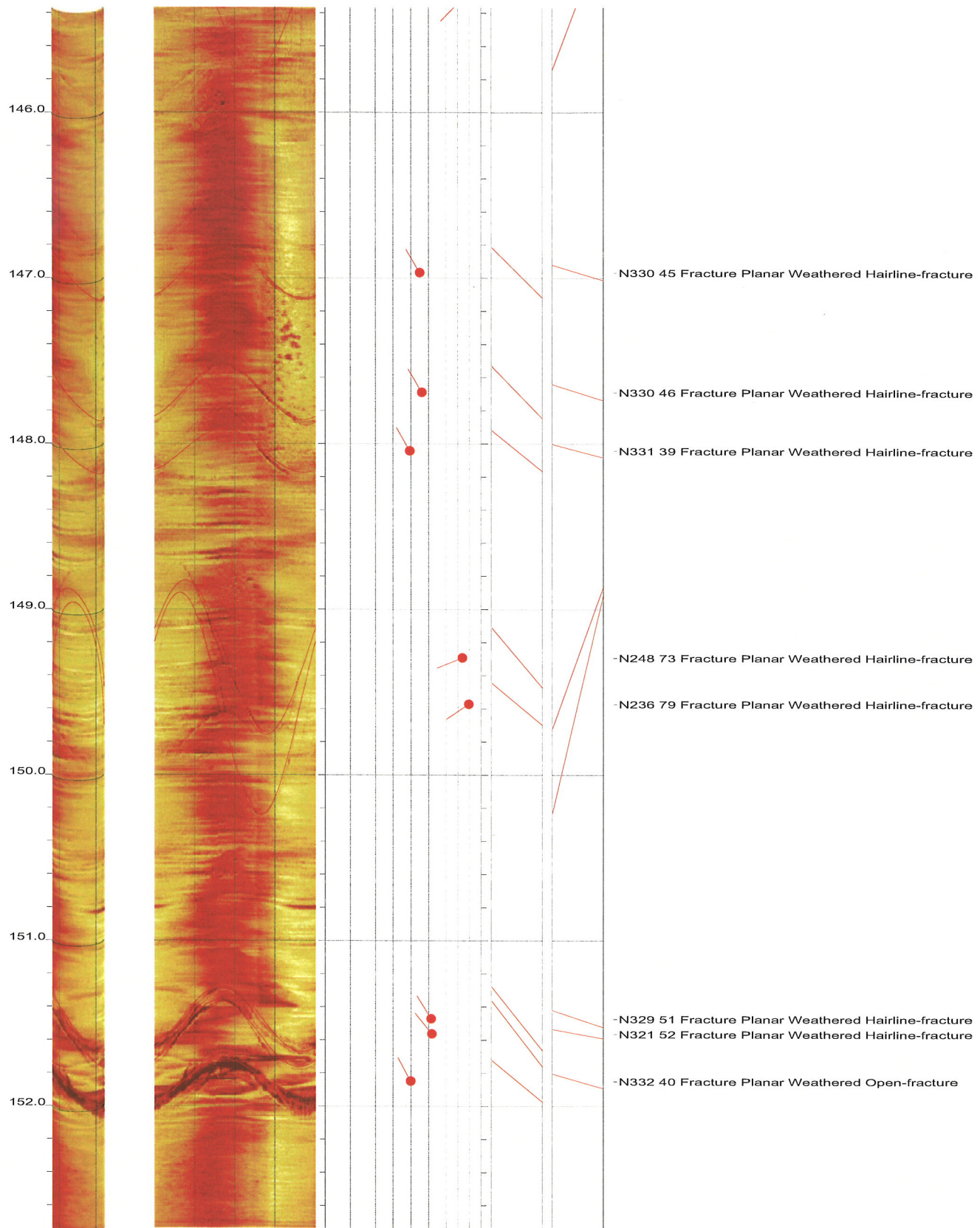
North Anna COL Boring B-907 Acoustic Televiewer Dips Sheet 21 of 22
