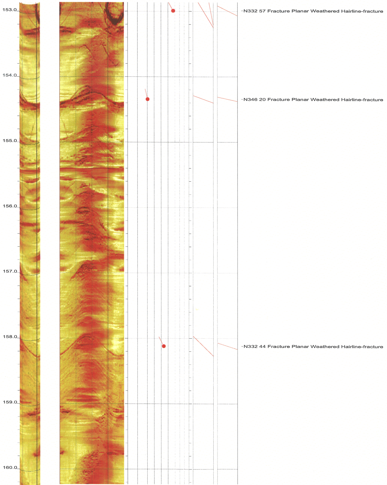
North Anna COL Boring B-901 Acoustic Televiewer Dips Sheet 17 of 36
