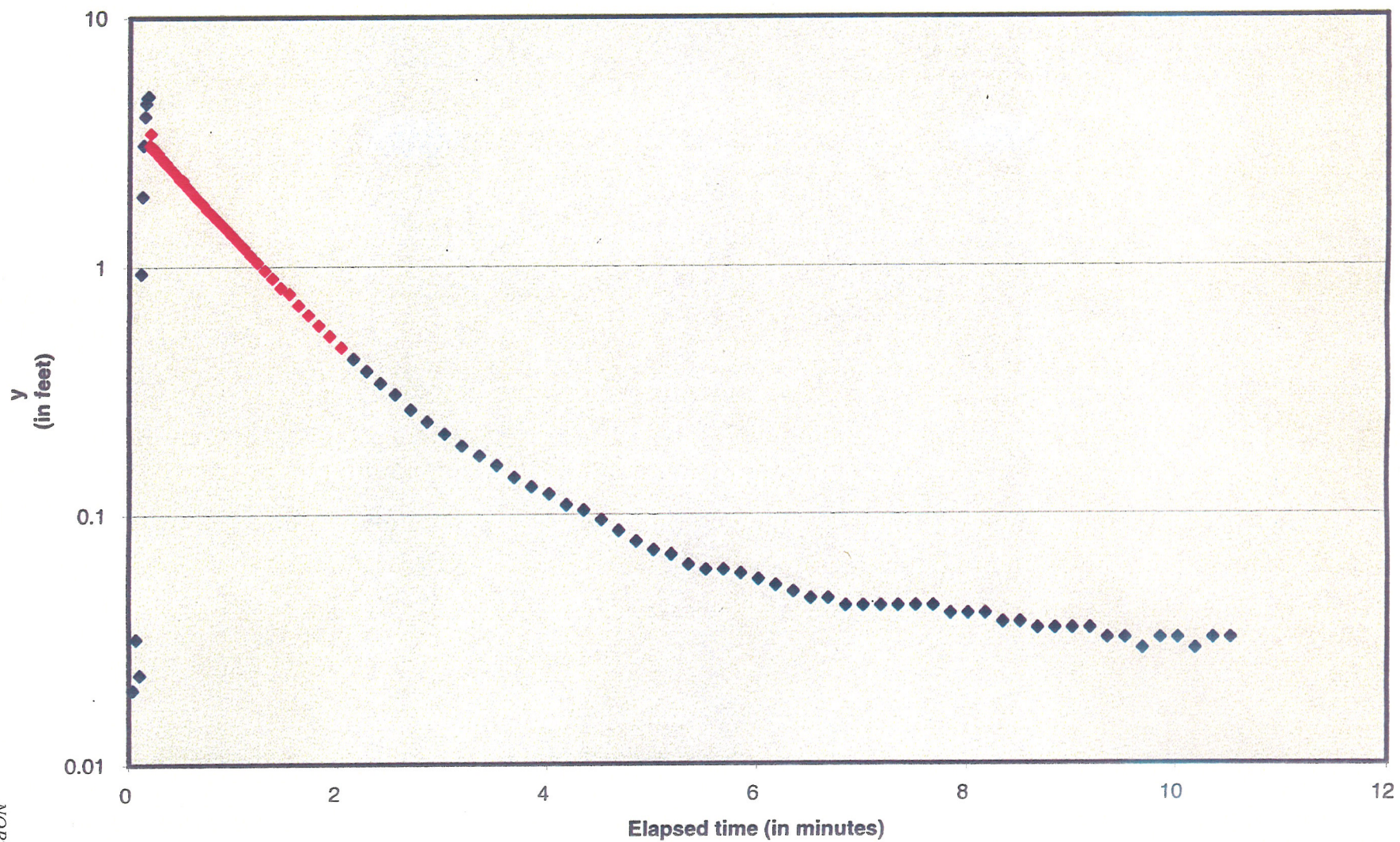
OW-949 (slug-in2) Recovery vs. Time
