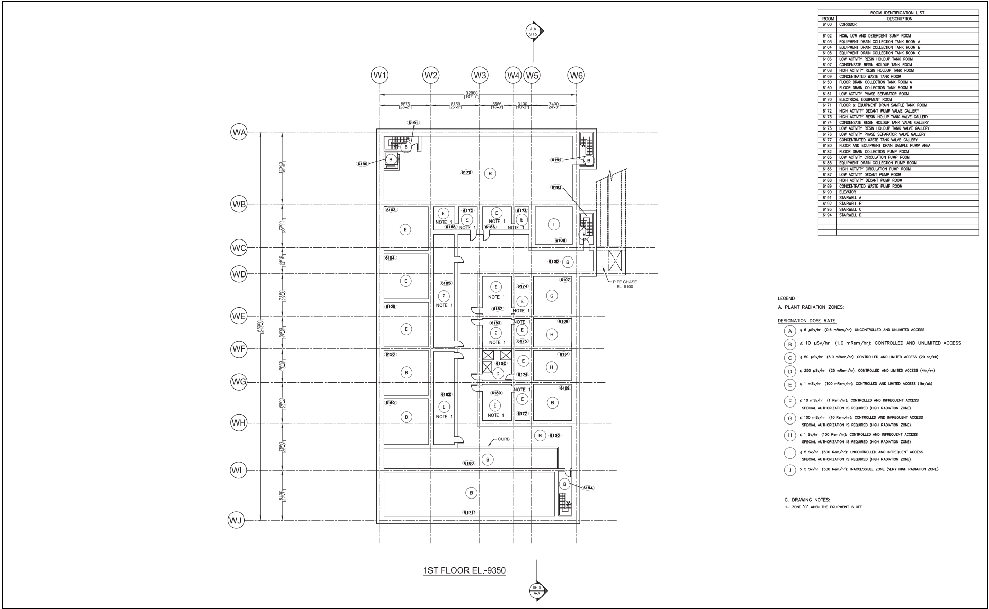
Figure 12.3-19R Radwaste Building Radiation Zones EL -9350
