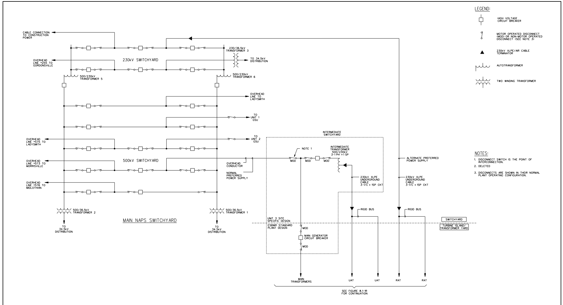
NAPS COL 8.2.4-1-A Figure 8.2-201 500/230 kV Switchyard Single-Line Diagram NAPS COL 8.2.4-2-A
