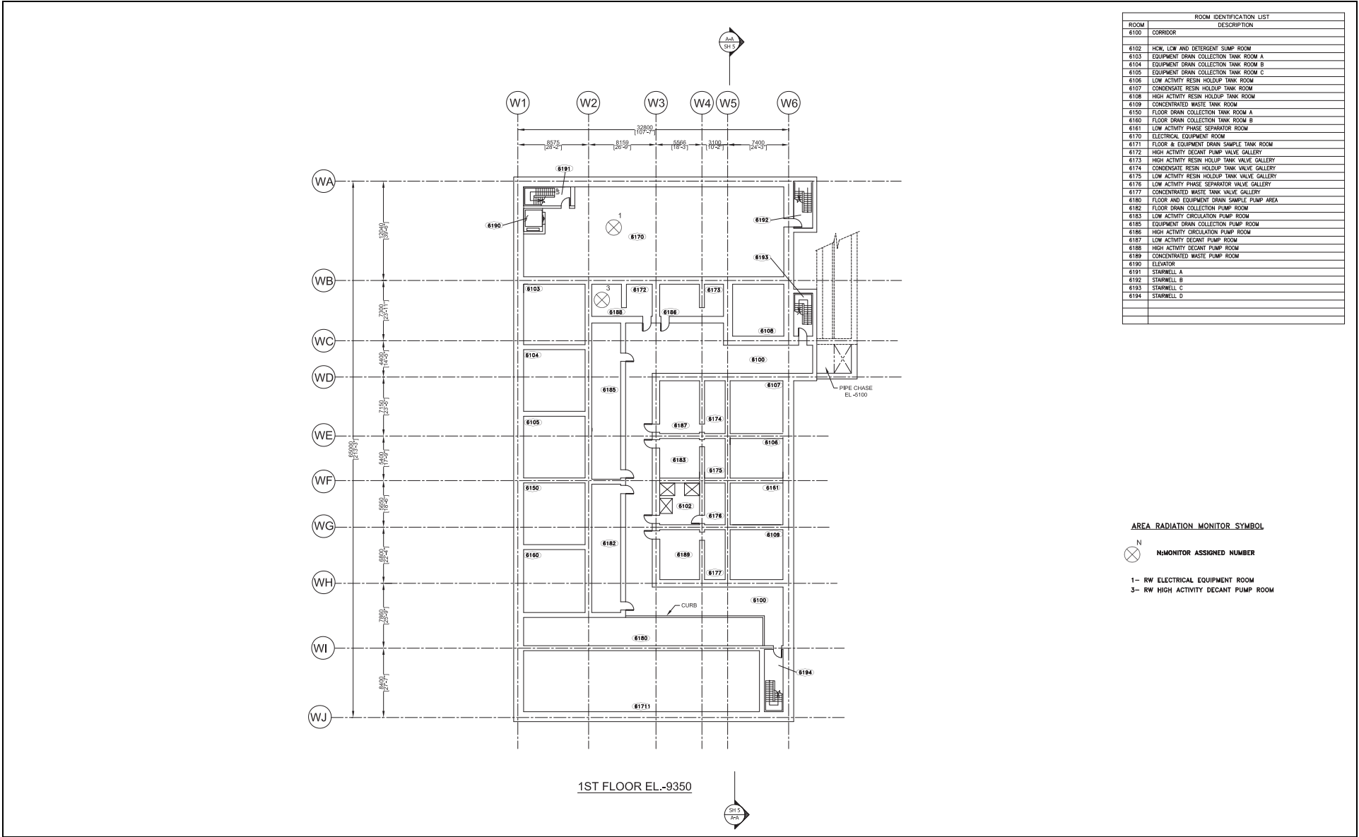
NAPS DEP 11.4-1 Figure 12.3-39R Radwaste Building Radiation Monitors EL -9350
