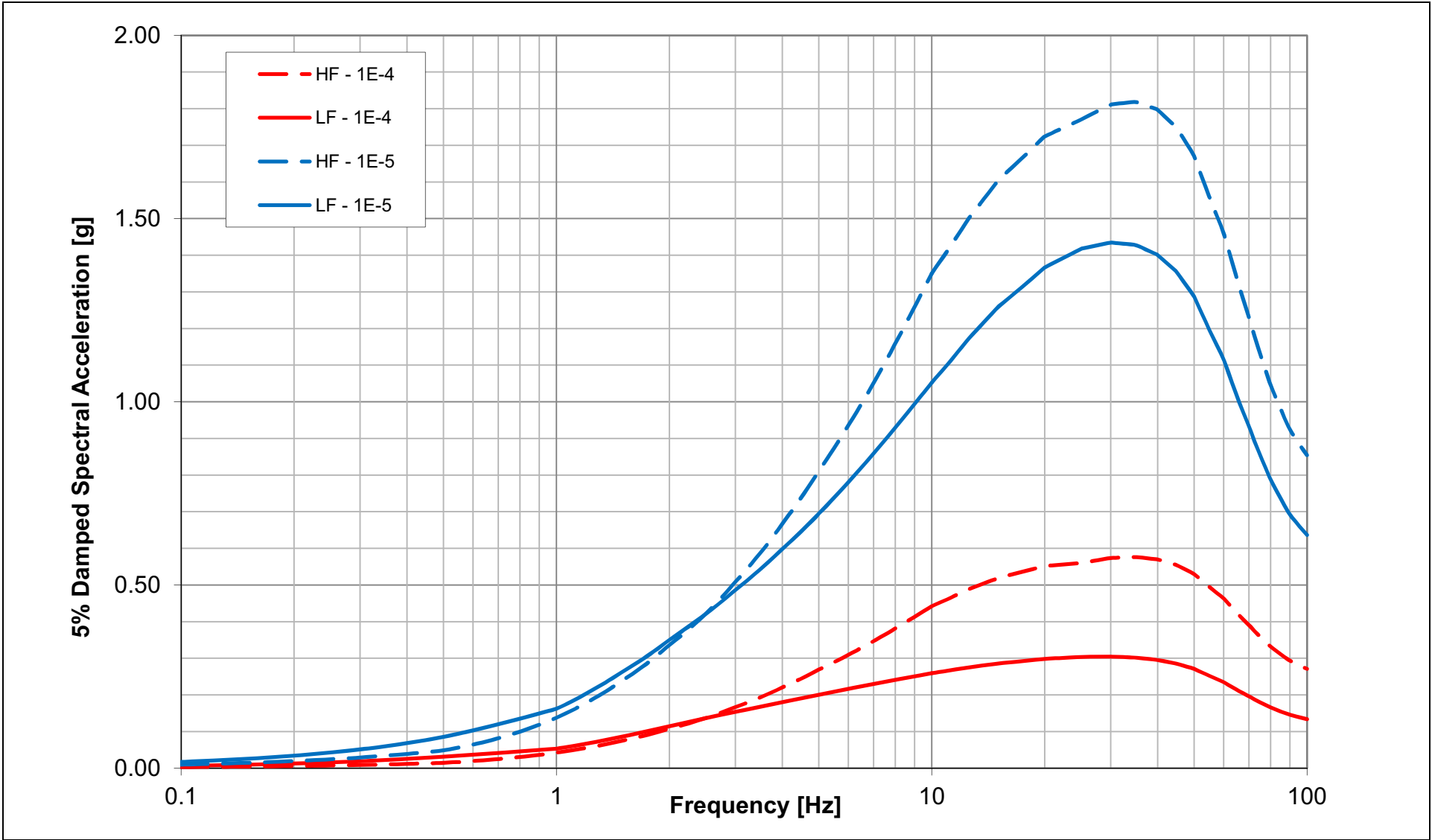
NAPS COL 2.0-27-A Figure 2.5.2-274 High Frequency (HF) and Low Frequency (LF) Hard Rock Input Ground Motion Spectra NAPS ESP VAR 2.0-4
