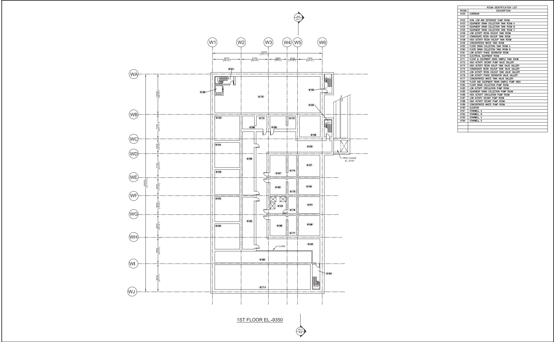
Figure 1.2-21R Radwaste Building Plan at Elevation -9350
