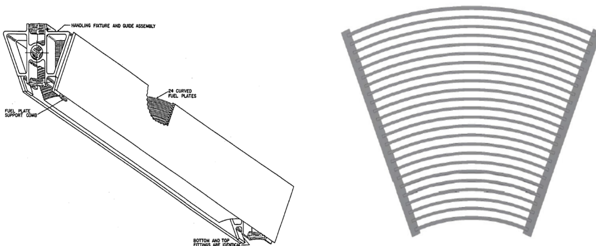
Figure 4-4 MURR fuel element
