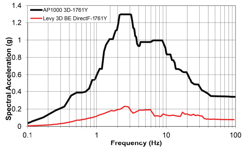
LEVY 3D SSI DIRECT FACTORED Y BE (1761)
