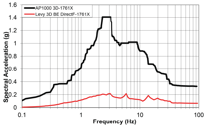
LEVY 3D SSI DIRECT FACTORED X BE (1761)
