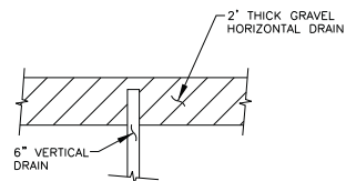
HORIZONTAL & VERTICAL DRAINS TYPICAL SECTION
