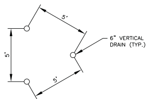
TYPICAL SPACING OF VERTICAL DRAINS
