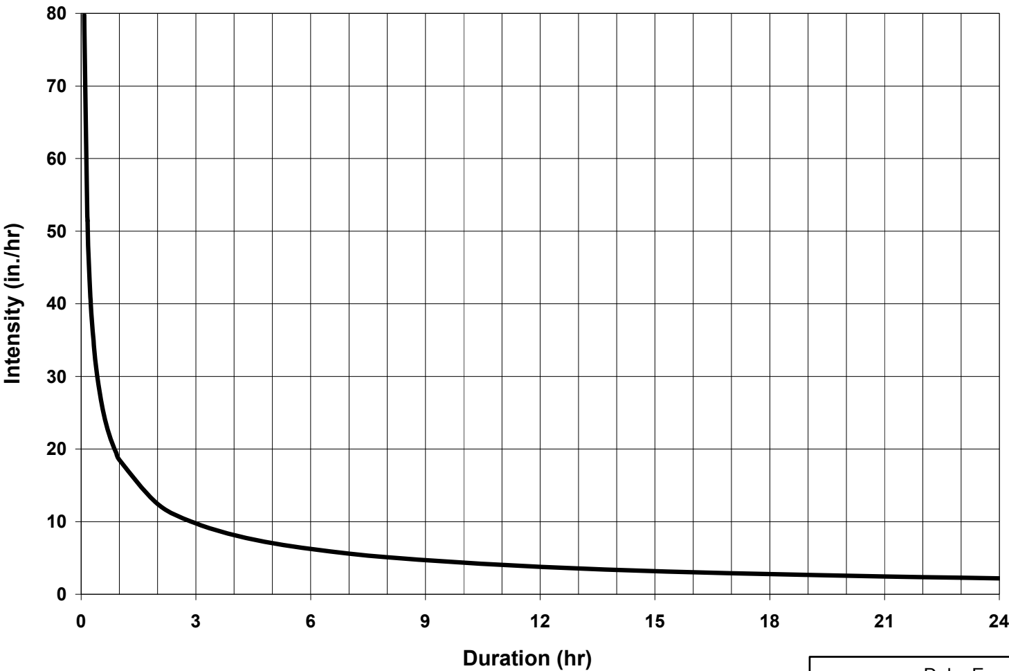
Duke Energy Florida Levy Nuclear Plant Units 1 and 2 Part 2, Final Safety Analysis Report Local Intense Probable Maximum Precipitation Intensity-Duration Curve FIGURE 2.4.2-203 Rev 6
