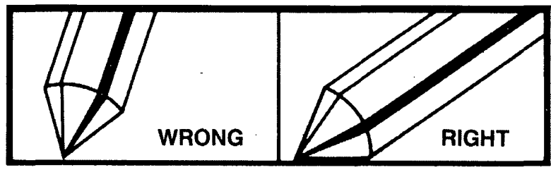
Figure E: Correct and incorrect way to hold the soldering iron against the parts to be soldered.
