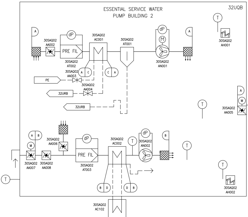
Figure 9.4.11-1—Essential Service Water Pump Building Ventilation System
