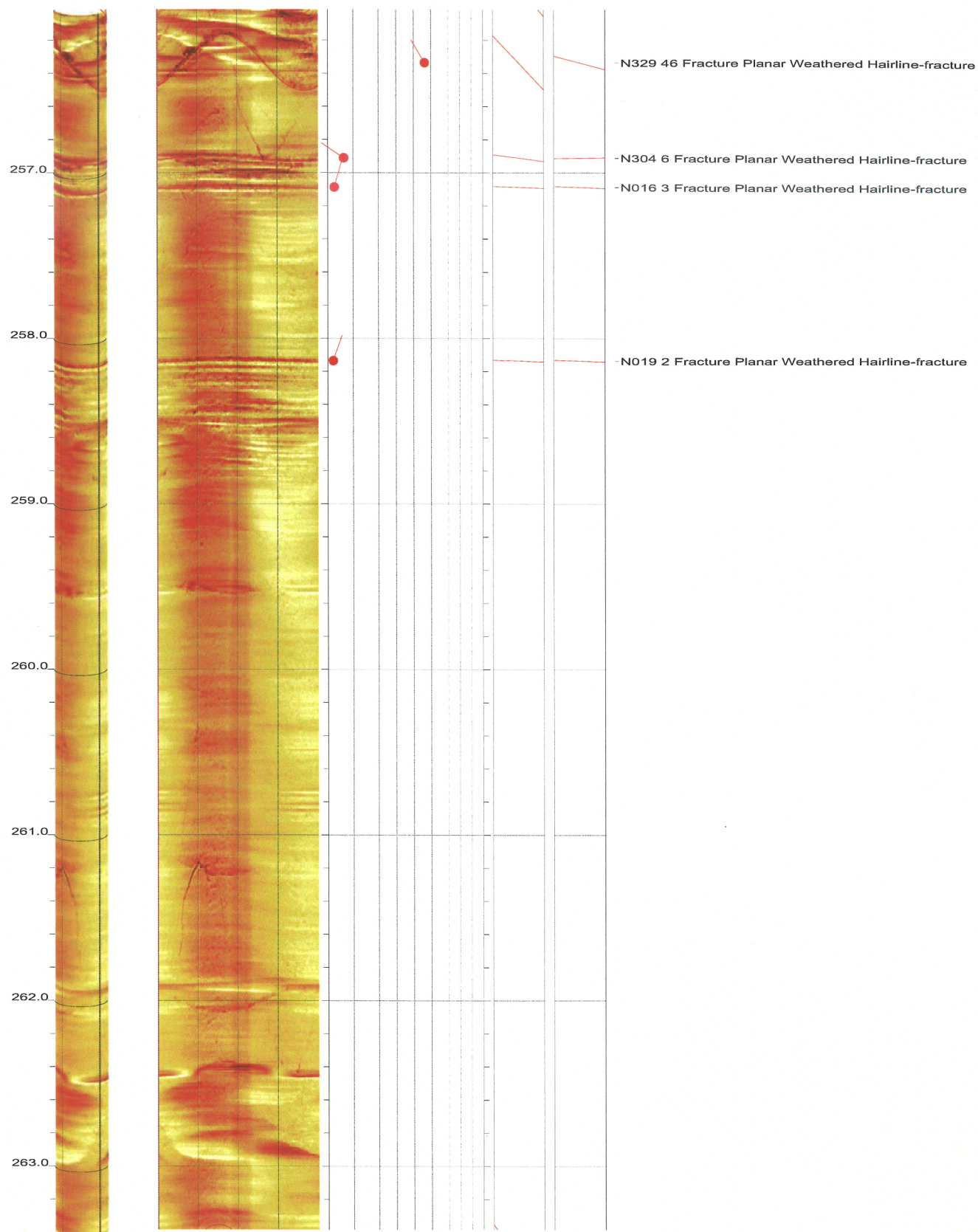
North Anna COL Boring B-901 Acoustic Televiewer Dips Sheet 31 of 36
