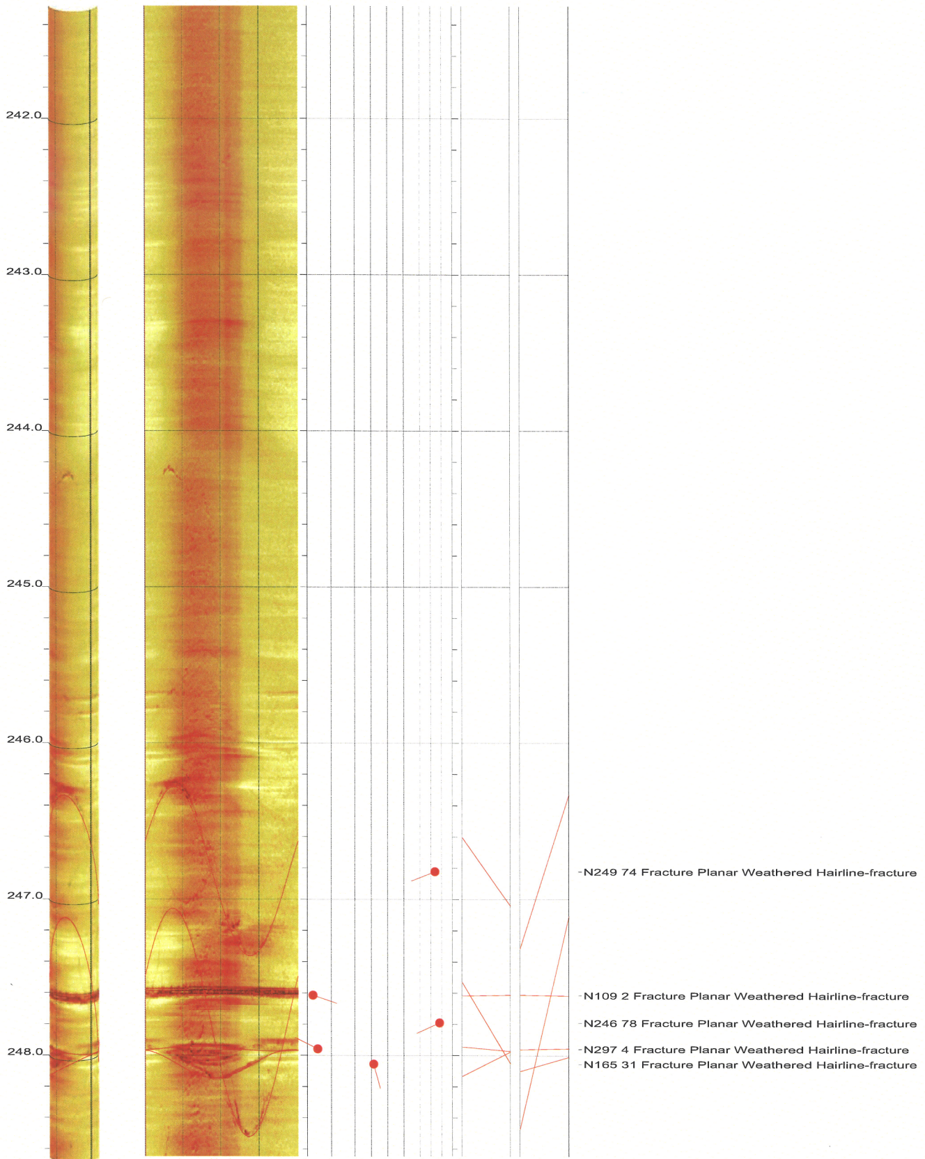
North Anna COL Boring B-901 Acoustic Televiewer Dips Sheet 29 of 36
