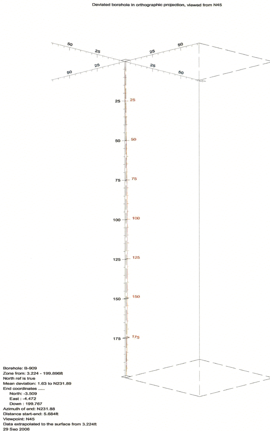
Figure 19. Boring B-909, Deviation Projection (dimensions in feet)
